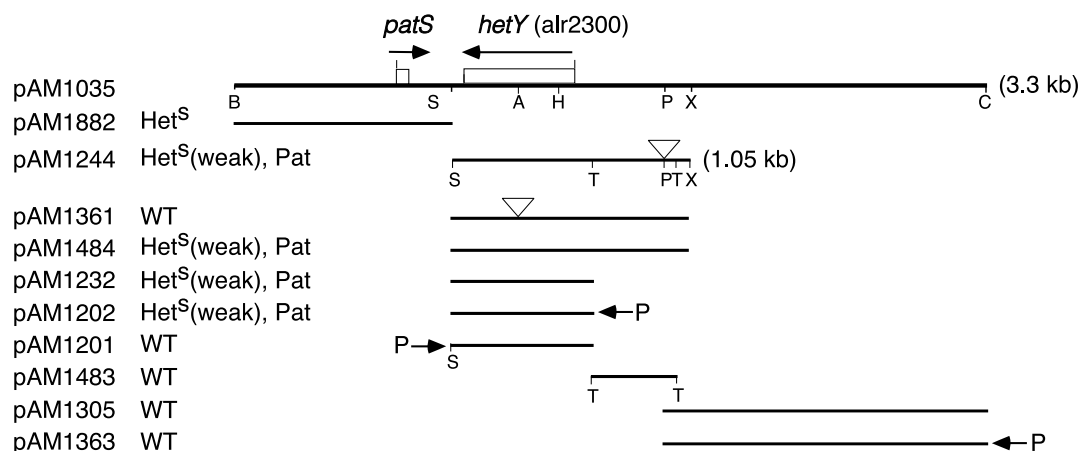
FIG. 1. Heterocyst suppression by DNA fragments subcloned from cosmid 8E11. Each shuttle plasmid was conjugated into Anabaena strain PCC 7120, and the heterocyst phenotype was determined. Phenotypes were scored as wild type (WT), heterocyst suppression (Het S ), and abnormal heterocyst pattern (Pat). Only selected restriction sites are shown. Symbols: arrows over ORF, direction of transcription; P with arrow, external promoter; inverted triangle, insertion of \Omega Sp r /Sm r cassette; A, AccI ; B, Bam HI; C, Cla I; H, Hinc II; P, Pac I; S, Sca I; T, Taq I; X, Xba I.
