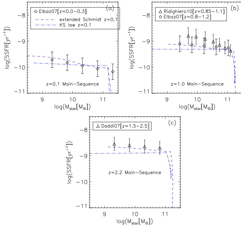
Figure 8. Observed star-forming main sequence from z = 0 to z = 2 compared to the predictions of implementing either the extended Schmidt law (dashed lines) or the KS law (dot-dashed lines) into the analytic model of gas accretion in the \Lambda CDM cosmology.
