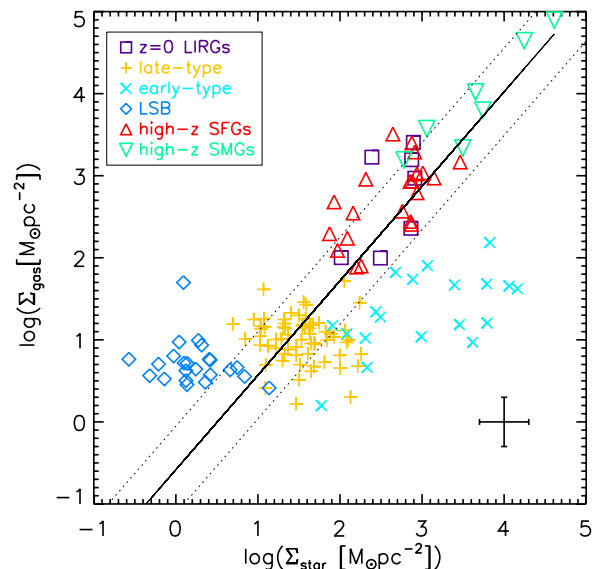
Figure 6. Gas mass surface density vs. stellar surface density. The solid line is the fit to galaxies excluding LSB and early-type ones. The dotted lines is the observed 1\sigma scatter.
