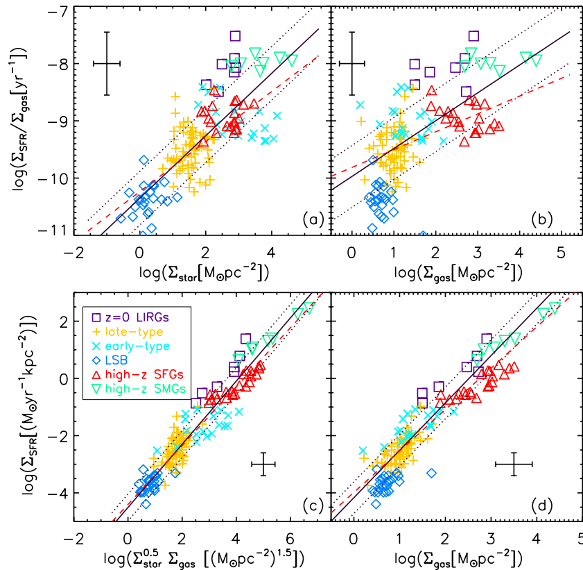
Figure 3. Similar to Figures 1 and 2 but using different CO-to-H 2 conversion factors for normal galaxies ( \alpha = 3.17 M_{\odot} \text{pc}^{-2} (\text{K km s}^{-1})^{-1} ) and merging objects (local LIRGs and high- z submillimeter galaxies; \alpha = 1.0 M_{\odot} \text{pc}^{-2} (\text{K km s}^{-1})^{-1} ). The solid and dotted lines are the intrinsic best-fit and observed 1\sigma scatter, respectively, to all data points but excluding LSB and early-type galaxies for panels (b) and (d). The dashed lines show the best fit to all the non-mergers but excluding LSB and early-type ones for panels (b) and (d).
