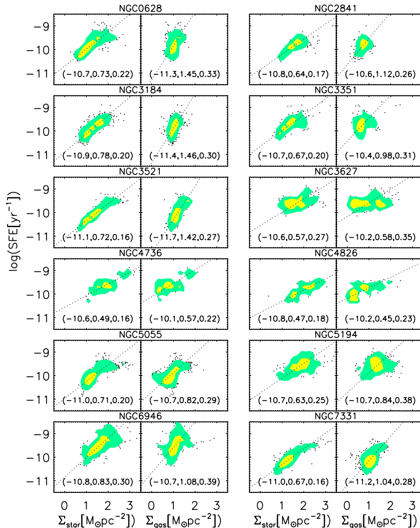
Figure 4. Extended Schmidt law at sub-kiloparsec resolution (the left side of each panel) compared to the KS law (the right side of each panel) in a sample of 12 spiral galaxies. The filled yellow and green areas enclose 50% and 90% of the total data points, respectively, while the dots are those outside the 90% area. The numbers listed in the parenthesis are in a sequence of interception, slope, and 1\sigma observed scatter as given by the ordinary least-squares bisector fit (Isobe et al. 1990), while the dotted line is the best fit.
