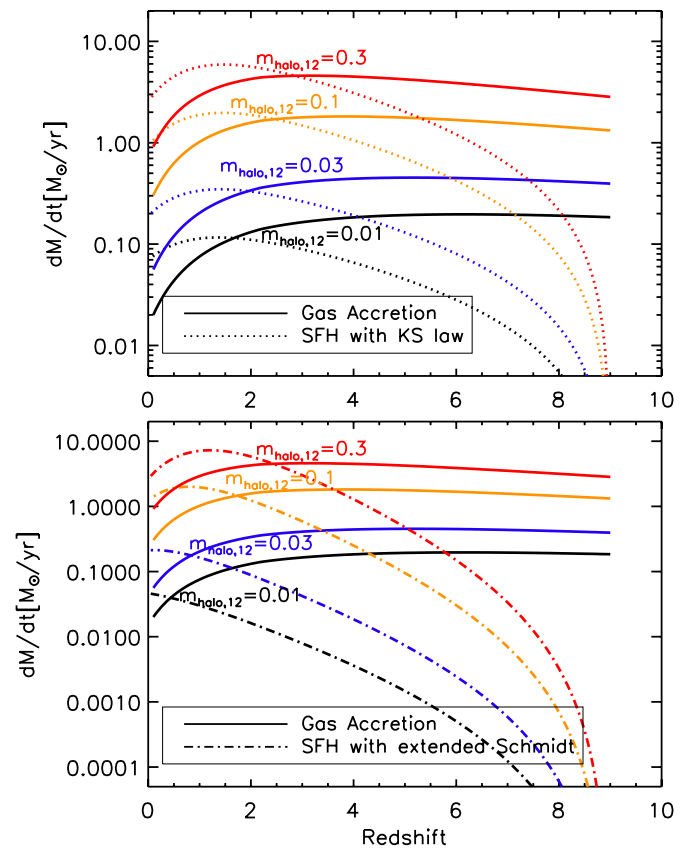
Figure 7. Upper: the evolution of SFR( z ) (dotted lines) as predicted by the KS law for given gas accretion histories (solid lines with the same colors) in four different halo masses where m_{\text{halo},12} is the halo mass at z=0 in units of 10^{12} M_{\odot} . Lower: the SFR histories with the extended Schmidt law.
