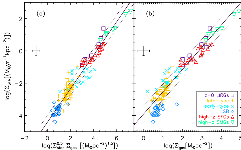
Figure 2. Comparison between the extended Schmidt law and Kennicutt–Schmidt relationship in the ability to predict the SFR. The solid and dotted lines are the intrinsic best-fit and observed 1\sigma scatter, respectively, as listed in Table 4. The fit to the KS law (right panel) is done excluding LSB and early-type galaxies. Typical measurement error bars are plotted.
