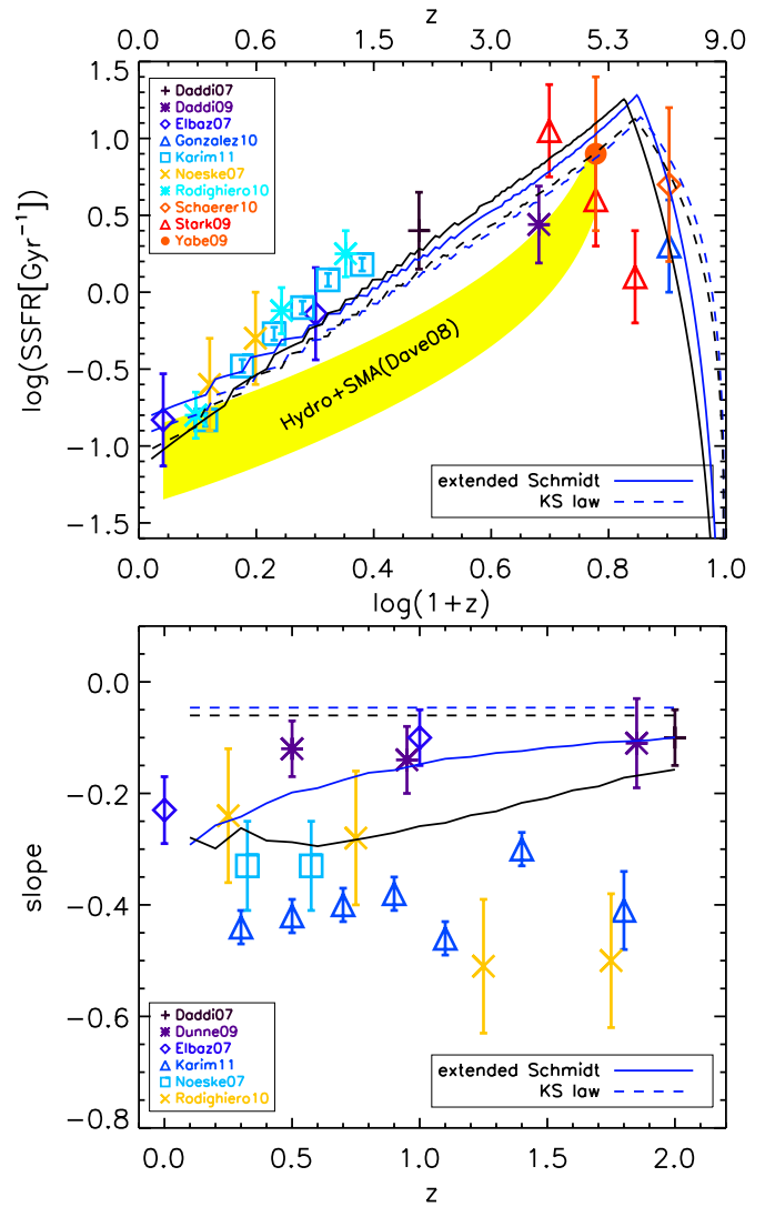
Figure 9. Upper panel: the observed evolution of the specific star formation rate (SSFR) for M_{\text{star}} = 10^{10} M_{\odot} compared to the predictions by the extended Schmidt (solid lines) and KS laws (dashed lines). The data are taken directly from the literature except for Stark et al. (2009) where we further correct the extinction according to the luminosity- and redshift-dependent extinction correction curve of Bouwens et al. (2009). “SMA” stands for the semi-analytic model. Lower panel: the evolution of the observed slope (specific SFR \propto M_{\text{star}}^{\text{slope}} ) as a function of the redshift from different studies. The solid and dashed lines show the result for the extended and KS laws, respectively, while the blue and black colors indicate the galaxy size evolution of \propto (H(z=4)/H(z)) and \propto (H(z=4)/H(z))^{0.4} , respectively. The data points correspond to the following references described in the legend: Daddi et al. 2007, 2009; Elbaz et al. 2007; González et al. 2010; Karim et al. 2011; Noeske et al. 2007a; Rodighiero et al. 2010; Schaerer & de Barros 2010; Stark et al. 2009; Yabe et al. 2009; and Dunne et al. 2009.
