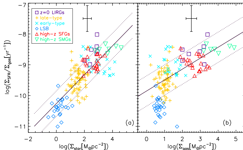
Figure 1. (a) The star formation efficiency ( =\Sigma_{\text{SFR}}/\Sigma_{\text{gas}} ) as a function of the stellar mass surface density. (b) The SFE as a function of the gas density. The solid and dotted lines are the intrinsic best-fit and observed 1\sigma scatter, respectively, as listed in Table 4. The fit to the SFE– \Sigma_{\text{gas}} (right panel) is done excluding LSB and early-type galaxies. Typical measurement error bars are plotted.
