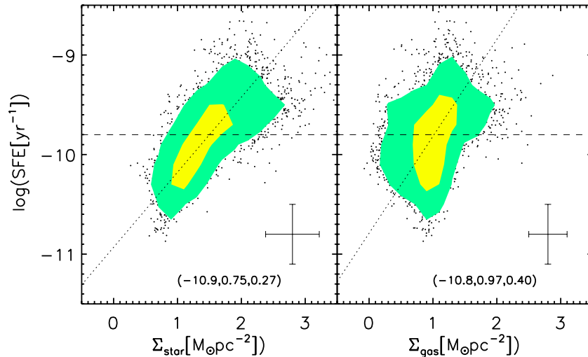
Figure 5. Extended Schmidt law at sub-kiloparsec resolution (the left side) and the KS law (the right side) of all sub-kiloparsec regions in 12 spiral galaxies. The filled yellow and green areas enclose 50% and 90% of the total data points, respectively, while the dots are those outside the 90% area. The numbers listed in the parenthesis are in a sequence of interception, slope, and 1\sigma observed scatter as given by the ordinary least-squares bisector fit (Isobe et al. 1990), while the dotted line is the best fit. The horizontal dashed line marks the transition below which the KS law has a much steeper slope (also see Bigiel et al. 2008).
