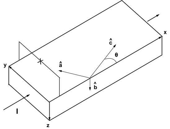
FIG. 1: The current I in the superconducting channel of the width W ( 0 < y < W ) and of the thickness d . The crystal axis b coincides with z . The cross denotes the Josephson junction.
