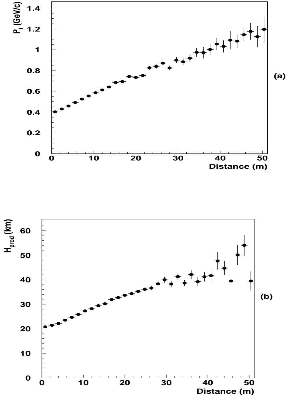
FIG. 1. Average separation of underground muon pairs at Gran Sasso depth, as a function of \langle P_{\perp} \rangle of the parent mesons (a) and of the slant height in the atmosphere (b). The results are obtained with the HEMAS Monte Carlo.
