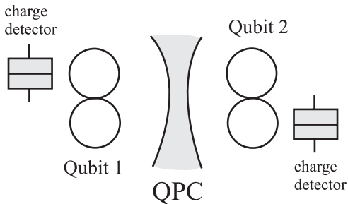
FIG. 3: Bell inequality setup. In order to be able to do a measurement of a violation of a Bell inequality, we use a QPC as a parity meter between two qubits to create a Bell state. The two outer detectors are then used to projectively measure charge in the \sigma_z basis of each qubit.
