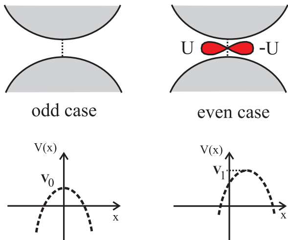
FIG. 2: Upper part: Top view of QPC in the parity meter setup. In the odd parity class, where (Q_L, Q_R) is (1, -1) or (-1, 1) , no dipole is generated across the QPC and it is nicely symmetric. In the even parity class, where (Q_L, Q_R) is (1, 1) or (-1, -1) , the situation is different. There, a dipole is generated across the QPC by the particular position of the electrons in the quantum dots. The dipole shifts the saddle point to the right (left) depending on the direction of the polarization of the dipole, but for both polarizations the shift is to higher energies. Note that the QPC in this figure is rotated by 90^\circ with respect to the QPC in Fig. 1. Lower part: Illustration of the saddle point potential for the two configurations.
