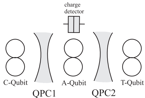
FIG. 4: CNOT gate setup. This setup contains three qubits and two parity meters, i.e. QPC’s, in between them. The qubits are the control qubit (C-Qubit), the ancilla qubit (A-Qubit) and the target qubit (T-Qubit). An additional projective measurement device is attached to the A-qubit.
