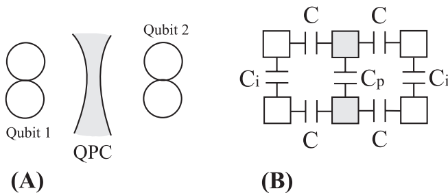
FIG. 1: Parity meter setup. In (A), two DQD's are shown with a QPC in between them. By measuring the current through the QPC, we are able to determine the parity class of the two-qubit state formed by a single electron in each DQD qubit. In (B), a capacitive model is illustrated for the setup considered in (A). The two grey boxes in the middle correspond to the dipole across the QPC.
