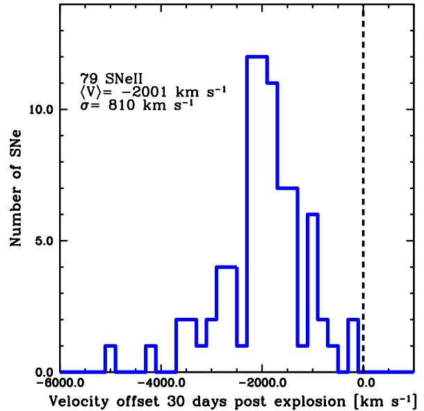
Figure 3. Histogram of the distribution of SN H \alpha emission velocity offsets for observations at 30 d after explosion.
