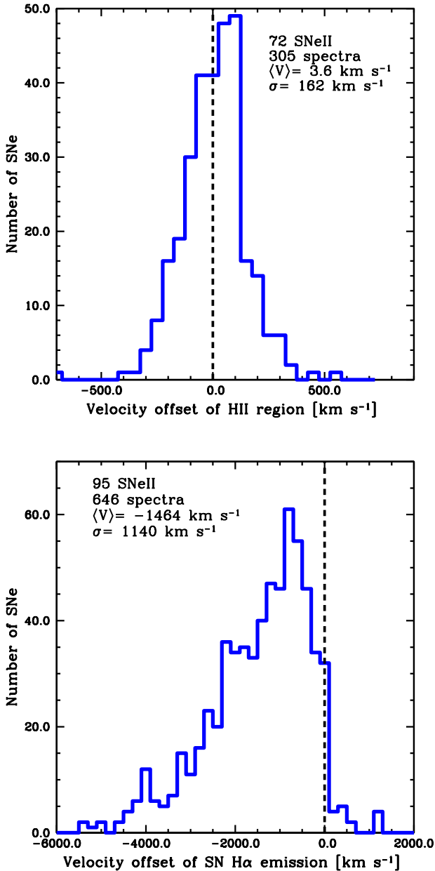
Figure 2. Top: Histogram showing the velocity of the narrow peak emission (associated with a coincident H II region) detected in each SN spectrum, and given with respect to the host galaxy recession velocity. Bottom: Histogram of the distribution of velocity offsets of H \alpha SN emission for the entire sample of type II SN spectra (corresponding to different post-explosion epochs).
