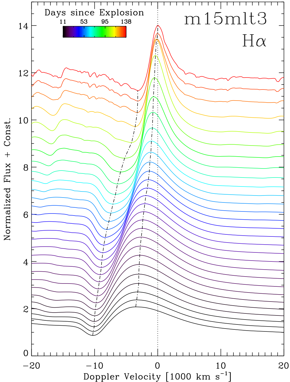
Figure 5. Evolution of the H\alpha spectral region from 11 d (bottom curve) until 138 d (top curve) after explosion in the SN II-P model m15mlt3 (Dessart et al. 2013). The abscissa is the Doppler velocity with respect to H\alpha . Individual times are color coded, and the time difference between consecutive models is 10% of the current time. The two broken lines track the location of maximum absorption and peak emission in H\alpha . The peak blueshift, strong at early times, decreases as the spectrum formation region recedes, and eventually becomes zero at the end of the plateau phase (in this model at \sim 140 d).
