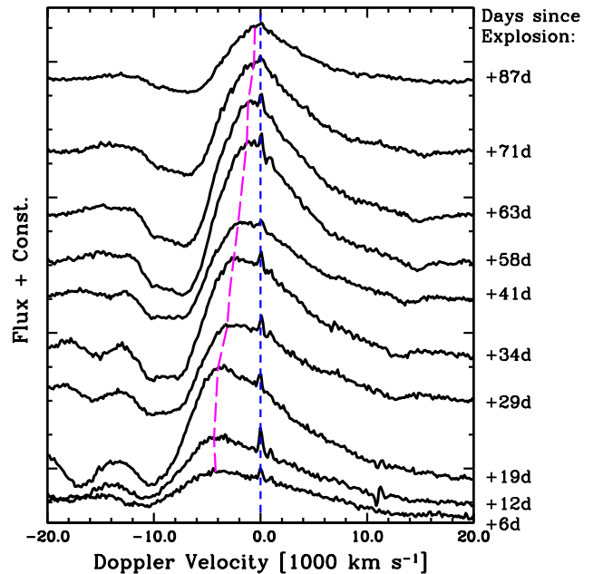
Figure 1. H\alpha spectral sequence of SN 2007X. The rest velocity of the SN position, as measured from the host H II region narrow H\alpha emission, is indicated by the short dashed blue line (i.e. at zero velocity). The long dashed magenta line shows the evolution of the Doppler velocity of the emission peak.
