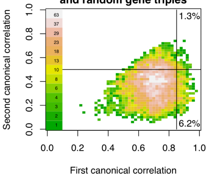
A Canonical correlations between virulence characteristics and random gene triples
