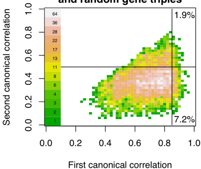
D Canonical correlations between virulence characteristics and random gene triples
