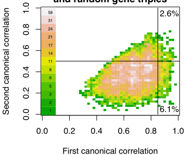
E Canonical correlations between virulence characteristics and random gene triples
