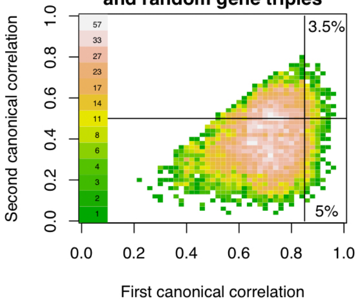
C Canonical correlations between virulence characteristics and random gene triples
