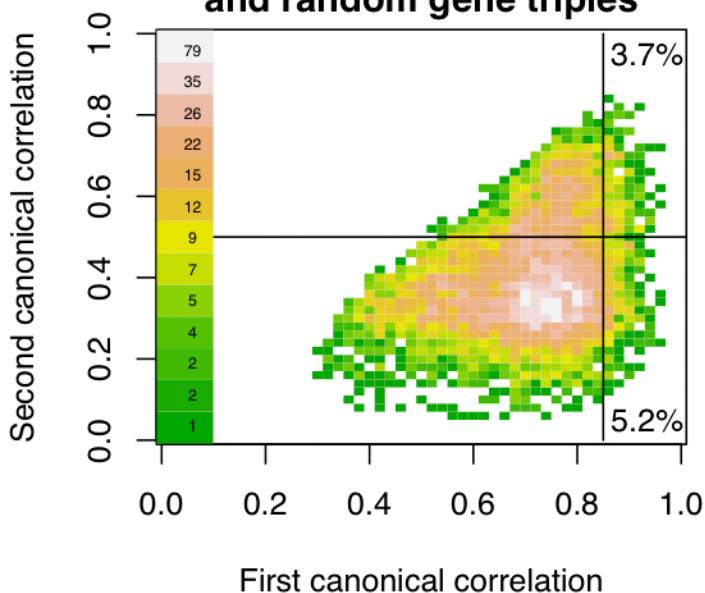
B Canonical correlations between virulence characteristics and random gene triples
