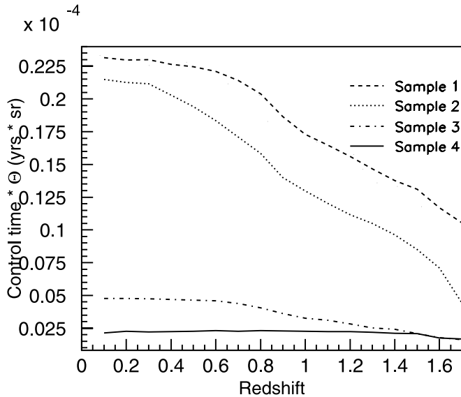
FIG. 4.—Product of the control time and surveyed area as a function of redshift for the four samples listed in Table 2, calculated for a stretch 1 SNe Ia. The dashed line is for sample 1, where the five GOODS-N epochs were used as the search data, and the combined 2004 ACS sample, as the reference. The dotted line is for sample 2, where the four epochs of the 2004 ACS data set were used as the search data, and the combined GOODS-N data, as the reference. The dot-dashed line is for sample 3, where all five epochs of the GOODS-S sample were used as the search data, and the combined epochs 4+5 of the GOODS-S data set, as the reference. The solid line is for sample 4, where all five epochs of the GOODS-S sample were used as the search data, and the combined epochs 1+2 of the GOODS-S data set, as the reference.
