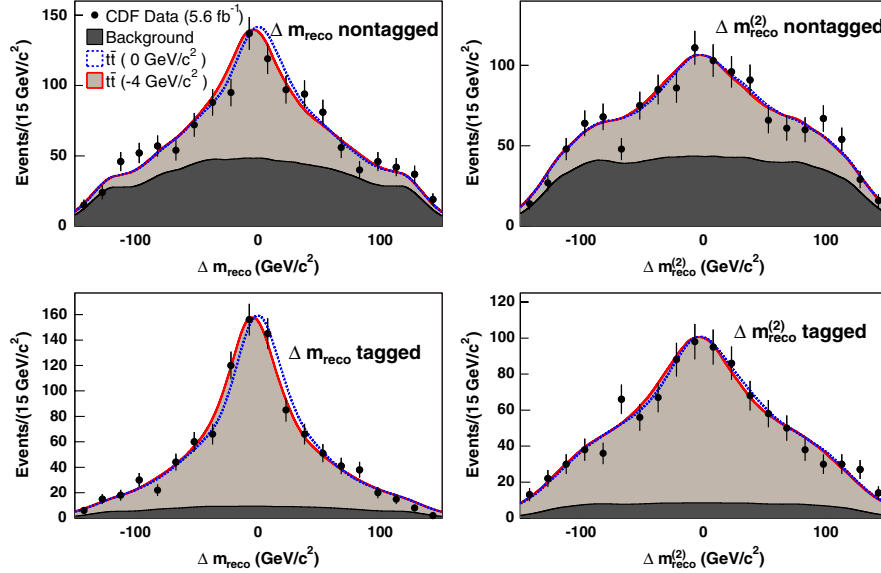
FIG. 1 (color online). Distributions of \Delta m_{\text{reco}} and \Delta m_{\text{reco}}^{(2)} used to extract \Delta M_{\text{top}} for zero b -tagged (nontagged) events and one or more b -tagged (tagged) events. The data are overlaid with the predictions from the KDE probability distributions assuming \Delta M_{\text{top}} = -4 \text{ GeV}/c^2 (solid red line) and \Delta M_{\text{top}} = 0 \text{ GeV}/c^2 (dashed blue line).
