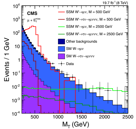
FIG. 7 (color online). Contributions from W - and W' -bosons decaying to \tau\nu \rightarrow \mu\nu\nu\nu compared to the prompt \mu\nu decay channel. Also shown are the contributions from the other backgrounds and the number of data events. The horizontal bars on the data points indicate the widths of the bins.
