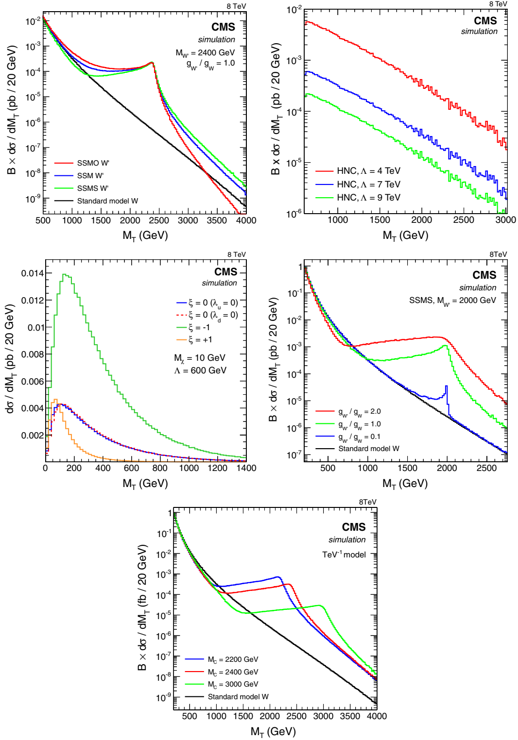
FIG. 3 (color online). Signal shapes at generator level: SSM model compared to the SSMS and SSMO models for g_W/g_{W^-} = 1 (top left), HNC-CI model for various values of \Lambda (top right), DM for various values of \xi (middle left), W' with W -boson interference and a varying coupling strength g_W/g_{W^-} in the same sign scenario (middle right), and TeV^{-1} model (bottom).
