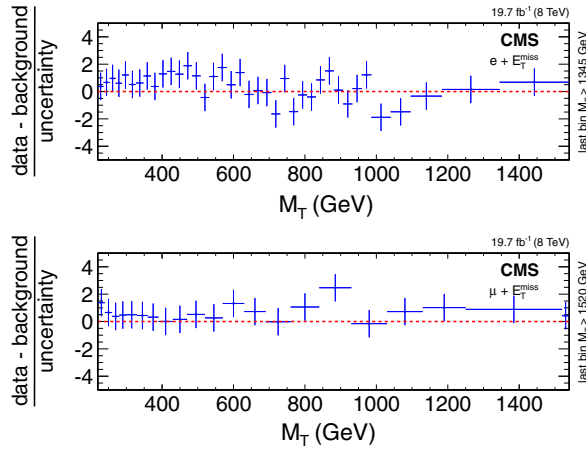
FIG. 6 (color online). Deviation of the number of observed events from the expectation, as shown in Fig. 5, in units of standard deviations, binned in M_T for the electron (top) and muon (bottom) channels. Both the systematic and statistical uncertainties are included. The horizontal bars on the data points indicate the widths of the bins, which are chosen as in Fig. 5 with the extension to include always five background events in a bin.
