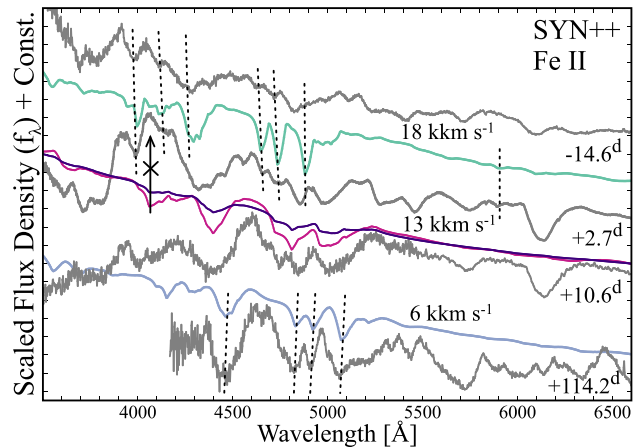
Figure 7. SYN++ single ion comparison for Fe II at 6000 , 13\,000 , and 18\,000 \text{ km s}^{-1} . At post-maximum light phases (after day +10.6 ), Fe II overlaps nicely with the observed spectrum as a species formed near the photospheric line-forming region. At early epochs (day -14.6 ), high-velocity Fe II is a promising match. The arrow marked with \times signifies that contributions from Fe II are restricted by the data at this wavelength for the given v_{\min} .
