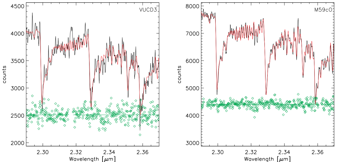
FIG. 2.— Integrated spectra of VUCD3 (left) and M59cO (right) are shown here in black. In both spectra the red lines indicate the best kinematic fit and the residuals are shown in green. For visibility, the zero points of the residuals are given as the green lines at 2510 counts and 4406 counts for VUCD3 and M59cO, respectively. A portion of the VUCD3 fit had to be masked due to bad sky subtraction. The integrated dispersion was determined to be \sigma = 39.7 \pm 1.2 km s -1 with a median S/N = 42 per pixel and \sigma = 31.3 \pm 0.5 km s -1 with a median S/N = 69 per pixel for VUCD3 and M59cO, respectively.
