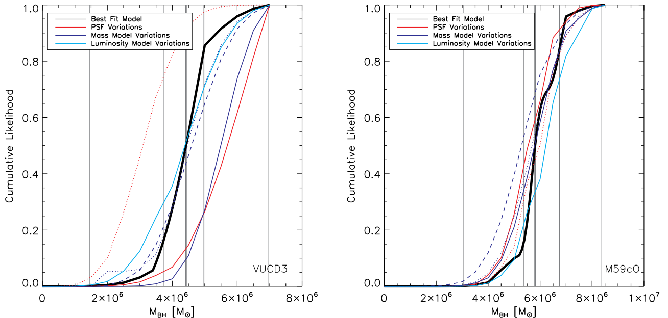
FIG. 5.— Cumulative likelihood, assuming isotropy, of the BH mass in VUCD3 (left) and M59cO (right). In both figures, the black solid line represents the best-fit model. The red, blue, and cyan lines indicate PSF, mass, and luminosity model variations, respectively. The grey vertical lines indicate the best-fit, one \sigma , and three \sigma BH mass estimates. See Section 4 for further explanation of the individual red, blue, and cyan lines.
