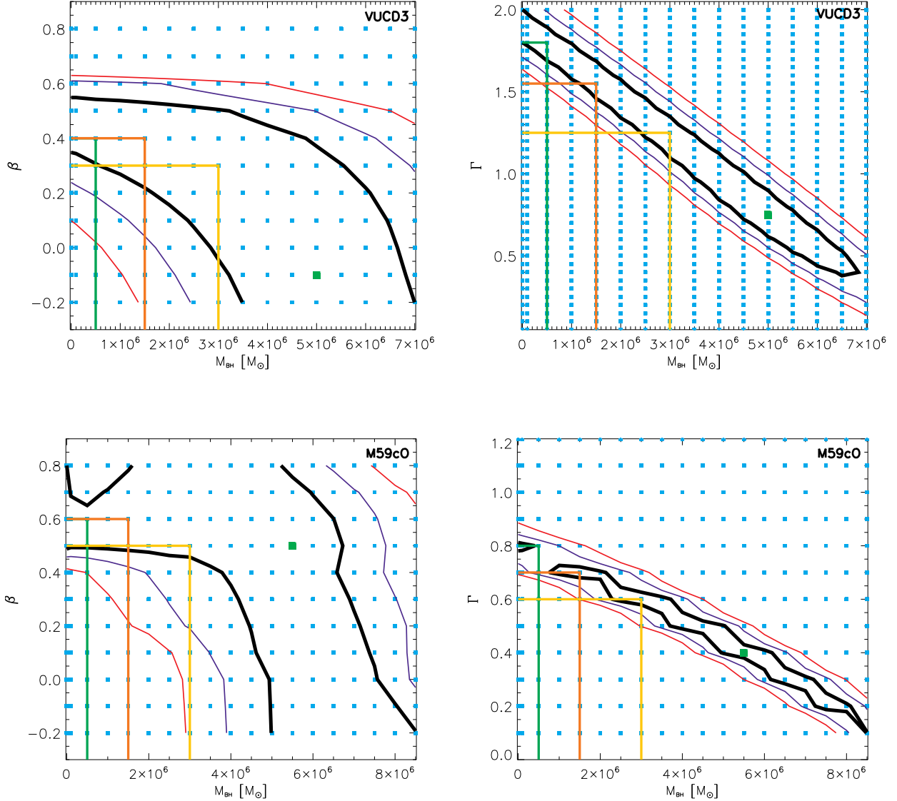
FIG. 7.— Contour plots showing the degeneracy between \beta_z , M_{BH} , and \Gamma , where VUCD3 is shown in the top panel figures and M59cO in the bottom. Data in the left panels have been marginalized over \Gamma ( \equiv (M/L)_{dyn}/(M/L)_* ), while data in the right panels are marginalized over \beta_z . The blue points represent the extent of our grid over these parameters and the green point represents the best fit determined for all free parameters. The black, blue and red contours represent the one, two, and three \sigma confidence levels, respectively, corresponding to \Delta\chi^2 values of 2.3, 6.2, and 11.8 (assuming two degrees of freedom). The green, orange and yellow lines correspond to the best fit \Gamma and \beta_z assuming the BH mass makes up 1%, 5%, and 10% of the total dynamical mass, respectively. We note that the M/L_* used corresponds to a M/L_V of 5.2 for VUCD3 and 4.1 for M59cO.
