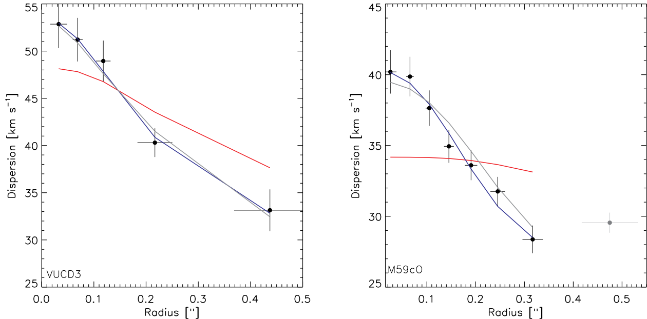
FIG. 6.— Dispersion profiles of VUCD3 (left) and M59cO (right) where black points are the measured velocity dispersions. The blue and red lines represent the best-fit isotropic models to the dispersion profile with and without a BH, respectively. The grey line represents the best-fit dynamical model without a BH, but including anisotropy. The grey point in the M59cO dispersion profile was not fitted.
