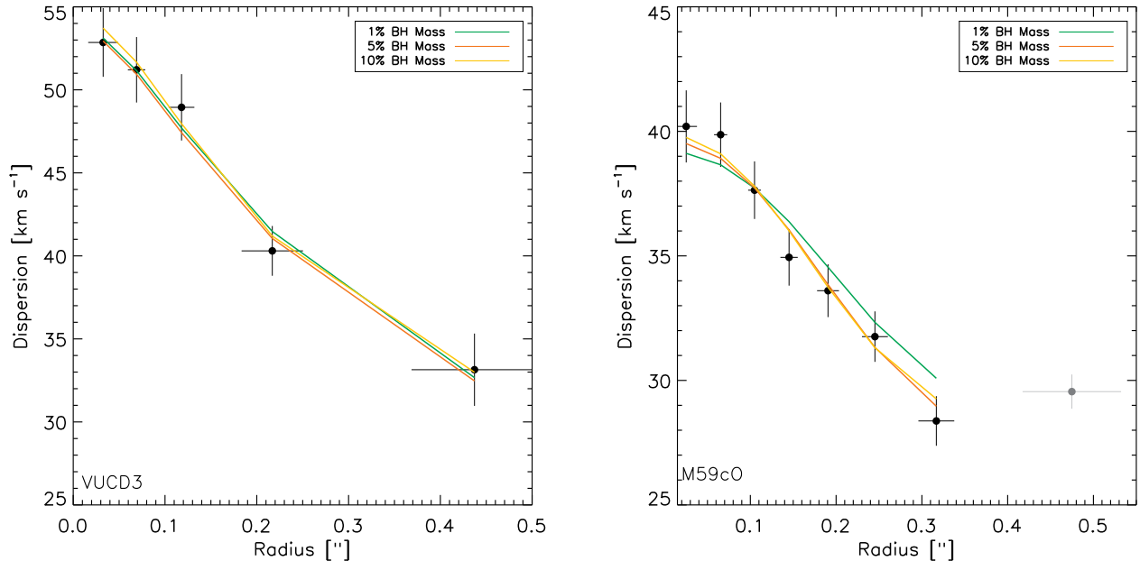
FIG. 8.— Dispersion profiles of VUCD3 (left) and M59cO (right) where black points are the measured velocity dispersions. The green, orange, and yellow lines represent the best-fit anisotropic models to the dispersion profile assuming the mass of the BH is 1%, 5%, and 10% of the total dynamical mass, respectively. For VUCD3, the best-fit \beta_z and \Gamma values are 0.4 and 1.8 (green), 0.4 and 1.55 (orange), 0.3 and 1.25 (yellow). For M59cO, the best-fit \beta_z and \Gamma values are 0.6 and 0.8 (green), 0.6 and 0.7 (orange), 0.5 and 0.6 (yellow). The grey point in the M59cO dispersion profile was not fitted.
