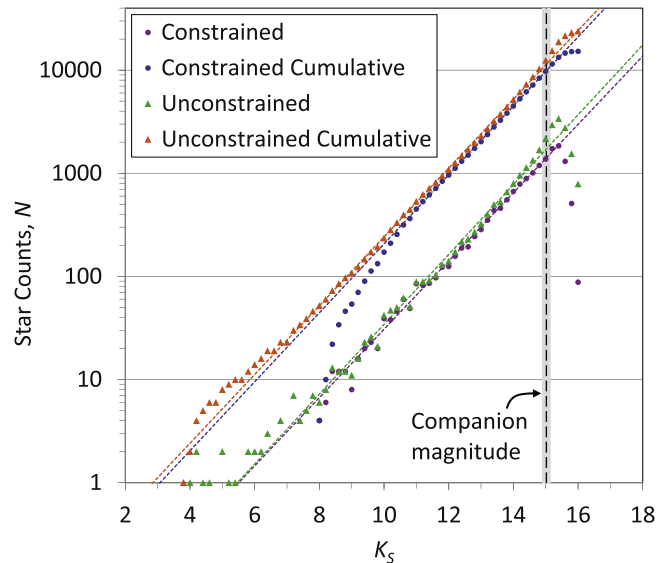
Figure 11. Absolute and cumulative stellar number density observed by 2MASS as a function of K_S magnitude in a 1 \text{ deg}^2 circular region centered on KELT-16. Star counts are grouped in bins of 0.2 mag corresponding to the \pm 1\sigma uncertainty of the companion star’s brightness. We include both the “unconstrained” case in which all 2MASS catalog entries are counted and the case in which counts are constrained by excluding those entries having quality flags (see the text). The black vertical dashed line and gray swath mark the K_S = 15.0 \pm 0.1 brightness of the companion. The colored dashed lines are model fits to the data of the form y = ae^{bx} , excluding the brighter data points due to low number statistics and excluding the fainter tails due to incompleteness.
