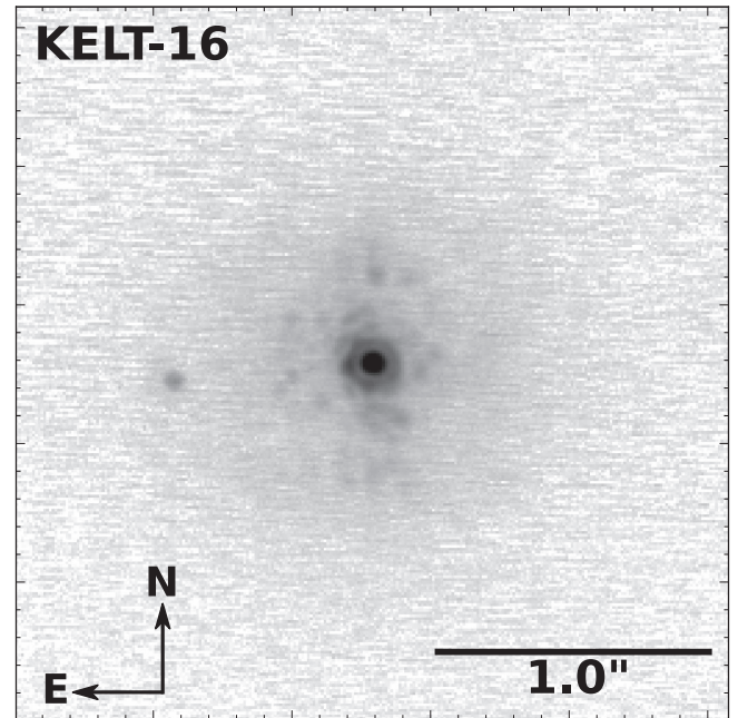
Figure 7. NIRC2/Keck II AO K_S stacked image of KELT-16 on a logarithmic scale. A stellar companion can be seen \sim 0.7'' to the east of the primary star. This image is for display purposes and includes only the three best frames; all 12 frames are used in the analysis.
