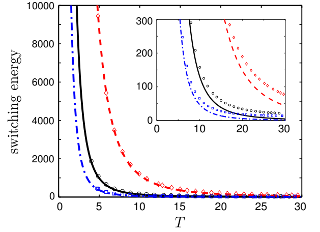
FIG. 2. (color online) Dependence of the switching energy in units of \int_0^T j^2(t) dt on the switching time T for \sigma = 0.01 (red dashed line), \sigma = 0.03 (black solid line) and \sigma = 0.05 (blue dot-dashed line). The inset shows the same dependence for smaller range of the switching energies. One can clearly see the deviations of the simulated data from the analytical solution for the small T limit.
