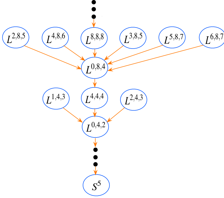
Figure 3: Chain of RG flows due to global deformations of L^{a,b,c} fixed points
