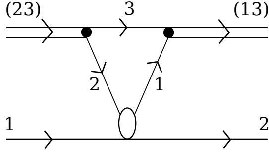
FIG. 9: The triangular diagram describing the exchange processes in the reaction 1 + (23) \rightarrow 2 + (13) . The four-ray vertex is the off-shell 1 + 2 Coulomb scattering amplitude.
