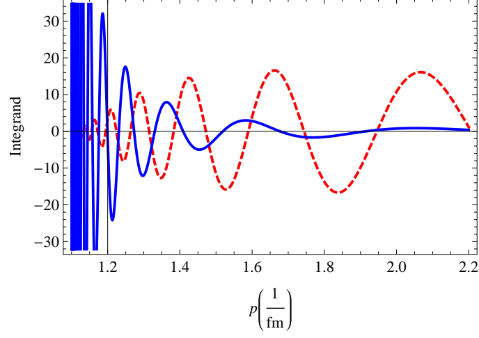
FIG. 12: (Color online) The same as in Fig. 11 but for p \geq p_\alpha .
