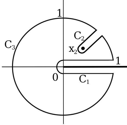
FIG. 13: Integration contour C = C_1 + C_2 + C_3 .
