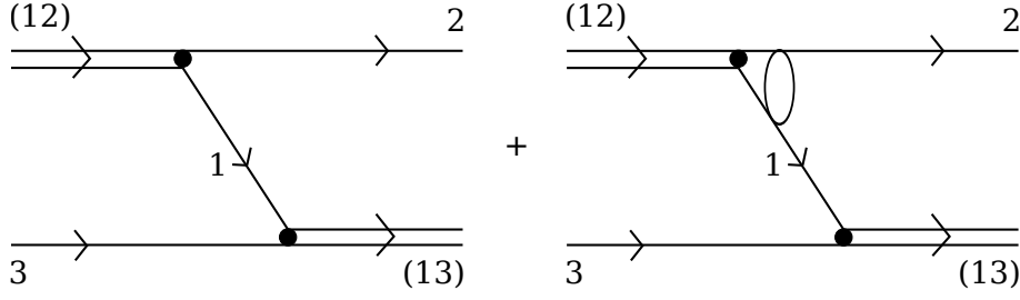
FIG. 3: The pole diagram describing the proton transfer in the reaction 3 + (12) \rightarrow 2 + (13) , which contains the Coulomb-modified form factor (12) \rightarrow 1 + 2 . Because this form factor consists of two terms, see Eq. (84), the diagram is also represented by the sum of two diagrams. In the first diagram in the vertex form factor (12) \rightarrow 1 + 2 no Coulomb interaction is included, but it is included in the second diagram. Bubble shows the off-shell Coulomb scattering amplitude of proton 1 and nucleus 2.
