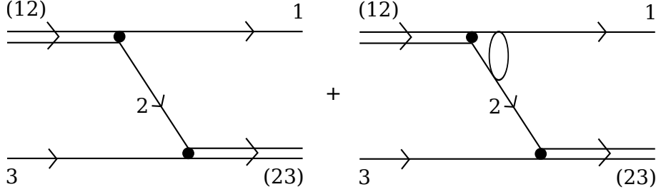
FIG. 4: The pole diagram describing the nucleus transfer in the reaction 3 + (12) \rightarrow 1 + (23) , which contains the Coulomb-modified form factor (12) \rightarrow 1 + 2 . Because this form factor consists of two terms, the diagram is also represented by the sum of two diagrams. In the first diagram in the vertex form factor (12) \rightarrow 1 + 2 no Coulomb interaction is included, but it is included in the second diagram. Bubble shows the off-shell Coulomb scattering amplitude of proton 1 and nucleus 2.
