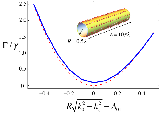
Figure 3. Solid line shows the average decay rate \bar{\Gamma} of \beta_{0,k_z} state for periodic distribution of atoms on cylindrical surface sketched on the top. The cylinder consists of 1000 atoms in 100 layers with 10 atoms per each layer. Radius of the cylinder is R = 0.5\lambda and the distance between adjacent layers is 0.1\pi\lambda . Analytical result (14) for an infinitely long cylindrical shell with 100/\pi\lambda atoms per unit length is plotted as dashed line. The horizontal axis is deviation of the R\sqrt{k_0^2 - k_z^2} from the root A_{01} of the Bessel function J_0(x) . \bar{\Gamma} = -\gamma \ln[P(1/\gamma)] is defined as average decay rate for time scale of 1/\gamma .
