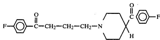
4-(p-fluorobenzoyl-piperidino)-4'-fluorobutyrophenone lenperone
