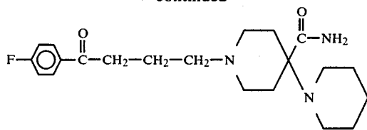
4-[4-(piperidyl)-4-carbamyl]-4'-fluorobutyrophenone floropipamide
