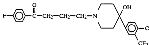
4-[4-(m-trifluoromethyl)-p-chlorophenyl]-4-hydroxypiperidino]-4'-fluorobutyrophenone clofluperol
