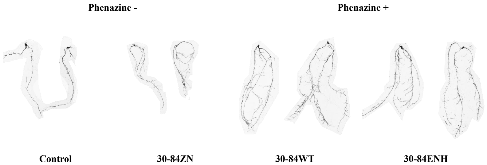
Figure 2.4: Effect of phenazine-producers on seedling root architecture. Winter wheat seedling were either grown in bacterial inoculated soil (30-84ZN, 30-84WT, and 30-84ENH) or non-inoculated soil (control) for 3 weeks (well-watered), and then exposed to two water stress cycles. After 7 days of recovery from the second water-stress cycle roots were harvested and scanned with EPSON Perfection V700. Pictures are representative samples of each treatment.
