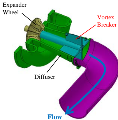
Fig.11 Vortex Breaker
