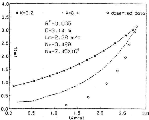
FIGURE 2 Prantl-Von Karman velocity distribution.
