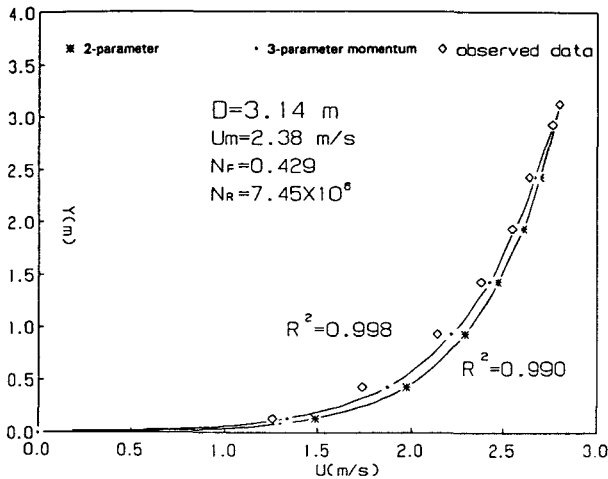
FIGURE 4 Entropy-based velocity distribution.
