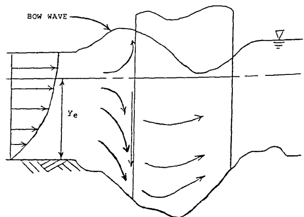
FIGURE 1 Hydrodynamics of flow in vortex.
