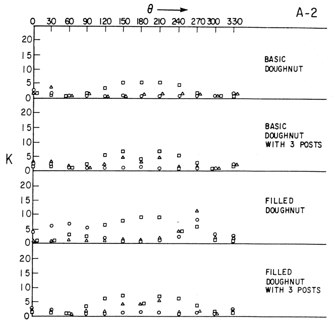
Figure 9. Total Pressure Loss Coefficient K VS Angular Position \theta —Intake A-2 ( \circ inner probe, \Delta middle, \square outer).
