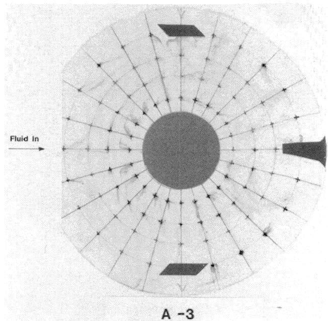
Figure 19. Wall Streamline Traces on Flat Face of Doughnut. Intake A-3 with posts at 90^\circ and 270^\circ .
