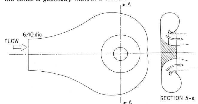
Figure 5. Intake B-1 (All dimensions in inches). See Table 1 for other dimensions.
