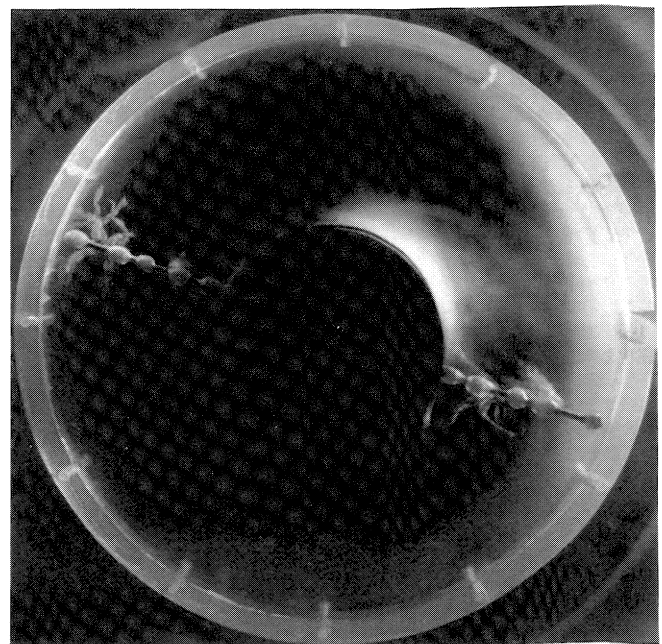
Figure 14. Observation of Wool Tufts at Pump Entry Plane for Intake A-1. Probes at \theta = 165^\circ and 345^\circ . Multiflash photo with eight flashes at 60 Hz.
