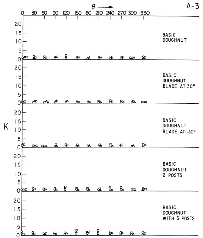
Figure 10. Total Pressure Loss Coefficient K VS Angular Position \theta —Intake A-3 ( \circ inner probe, \Delta middle, \square outer).
