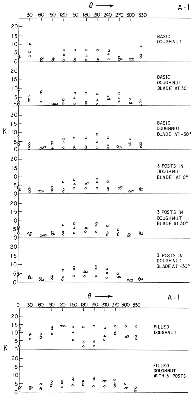
Figure 8. Total Pressure Loss Coefficient K VS Angular Position \theta —Intake A-1 ( K based on velocity head at pump inlet plant) ( \circ inner probe, \Delta middle, \square outer).
