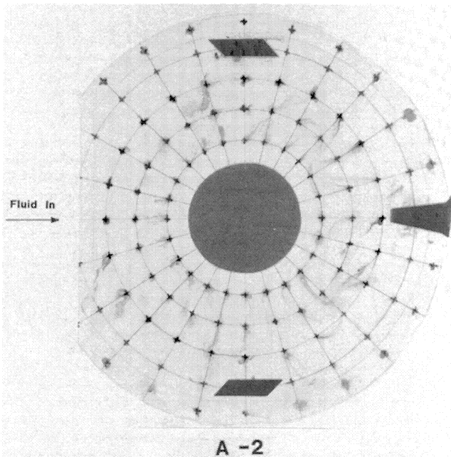
Figure 17. Wall Streamline Traces on Flat Face of Doughnut. Intake A-2 with posts at 90^\circ and 270^\circ .
