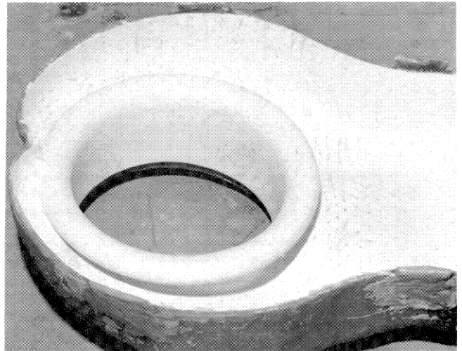
Figure 24. Wall Streamline Traces on Interior of Intake B-2. View of intake half-section including pump entry plane. Flow enters from the right.
