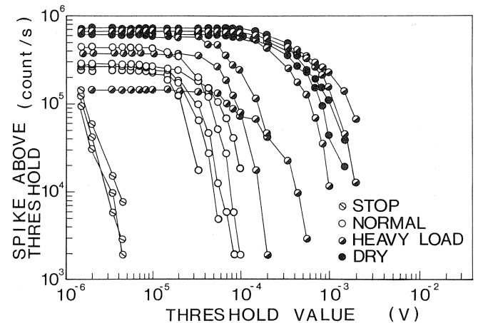
Figure 10. Amplitude Distribution Diagram of AE Waveforms.
