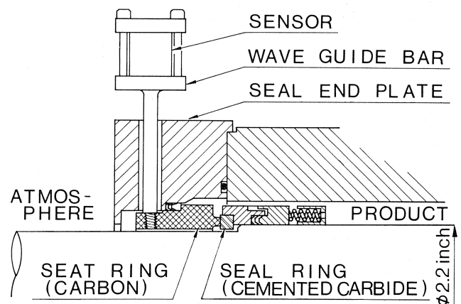
Figure 4. Mounting of a Sensor on a Mechanical Seal.
