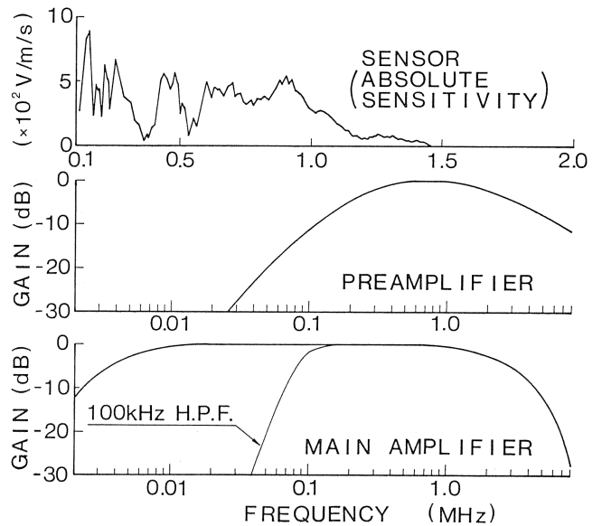
Figure 2. Frequency Response Characteristics of AE Measuring Instruments.
