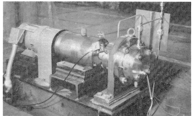
Figure 18. Measurement on Experiment Apparatus.
