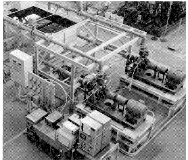
Figure 3. Test Apparatus.
