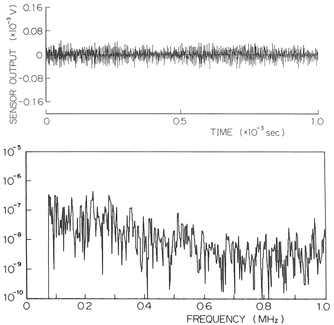
Figure 6. Typical AE Waveform and its Spectra under the NORMAL Condition.
