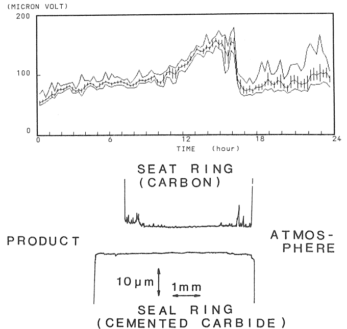
Figure 22. Typical AE Trend and Surface Configuration of Mechanical Seal on a Process Pump Operated with LPG.
