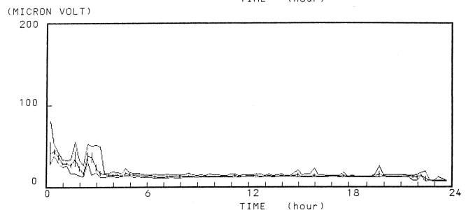
Figure 26. Low Level AE Trend During Leakage Following an Abnormal AE Trend.
