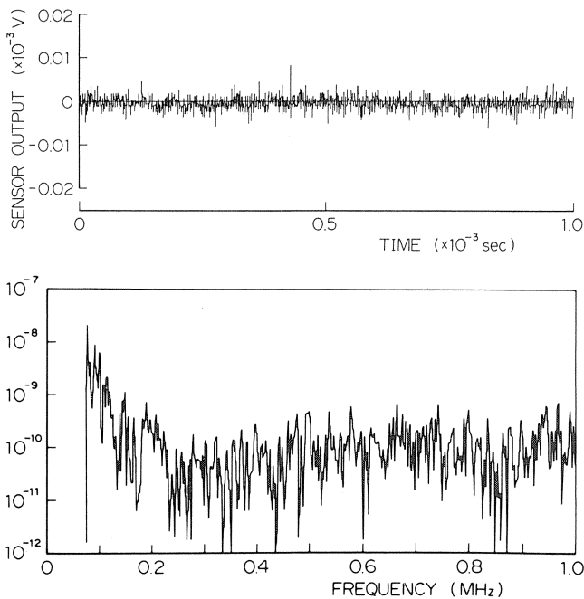
Figure 5. Typical AE Waveform and its Spectra under the STOP Condition.
