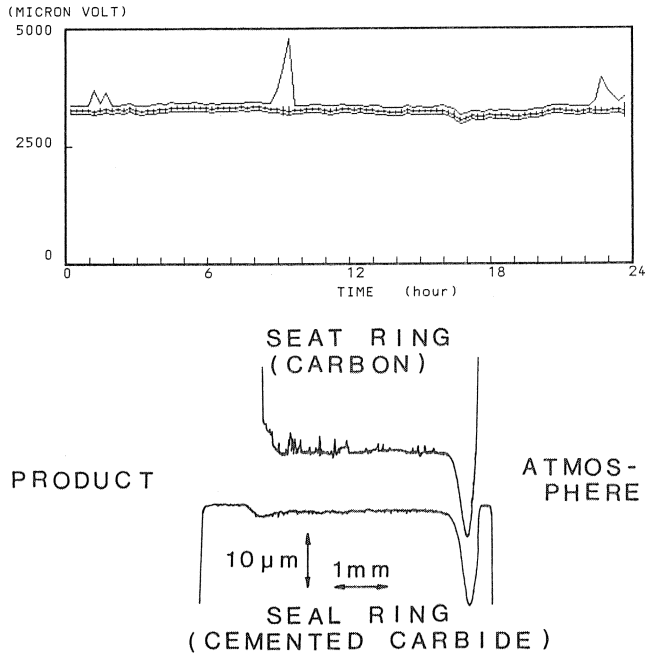
Figure 20. Typical AE Trend and Surface Configuration of Mechanical Seal on a Process Pump Operated with LPG.
