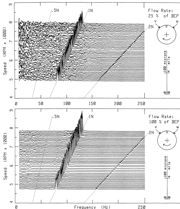
Figure 11. Uncompensated Shaft Vibrations (Vector V) with Two \times Nominal Clearance at Impellers and Balance Piston.
