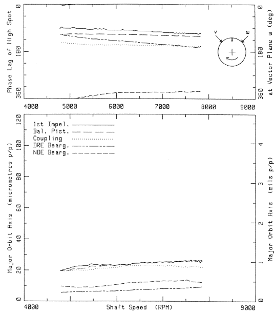
Figure 5. Shaft Vibrations with Nominal Clearances (Pump as Built).
