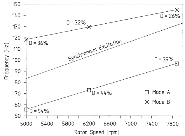
Figure 12. Campbell Diagram for Case 2.
