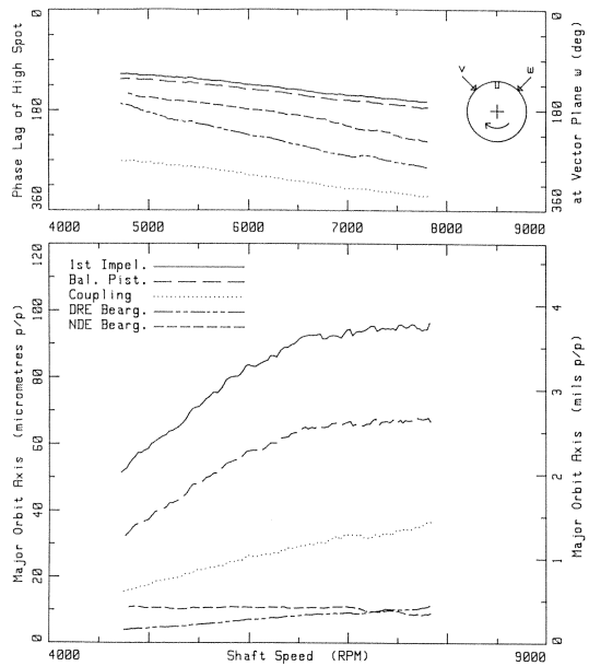
Figure 6. Shaft Vibrations with Two \times Nominal Clearance at Impellers and Balance Piston.
