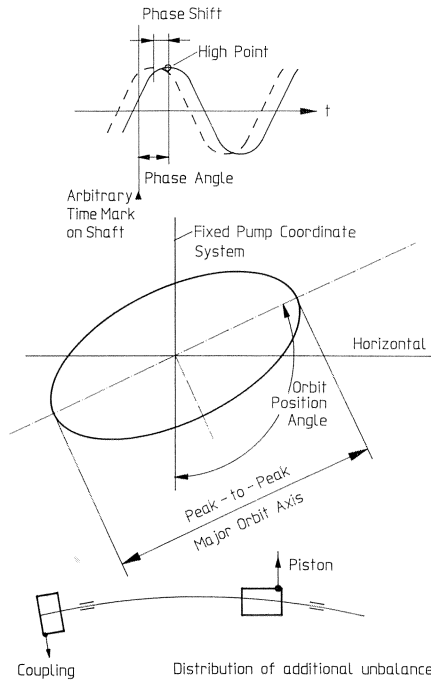
Figure 4. Definition of Vibration Parameters.
