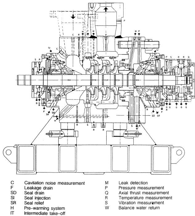
Figure 1. Pump Longitudinal Section.
