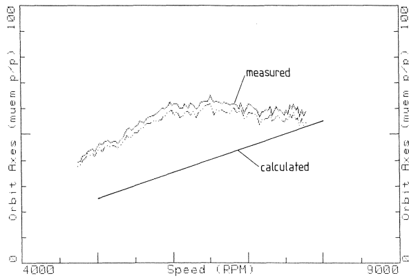
Figure 15. Comparison Test/Analysis, Case 2: Impeller.
