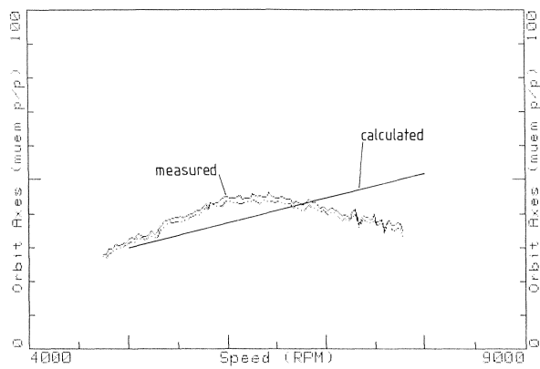
Figure 16. Comparison Test/Analysis, Case 2: Balance Piston.
