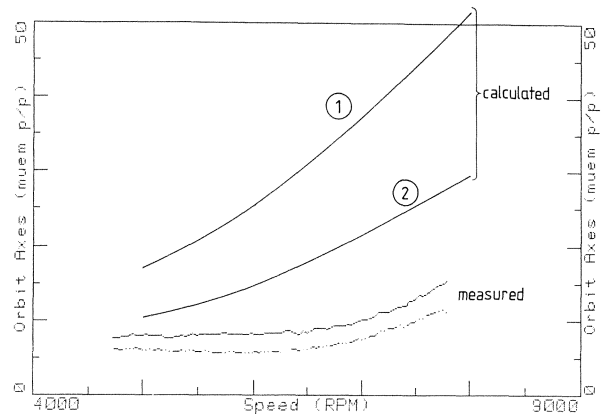
Figure 14. Comparison Test/Analysis, Case 2: Drive End Bearing.
