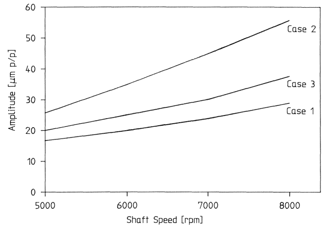
Figure 13. Calculated Unbalance Response at the Impeller.
