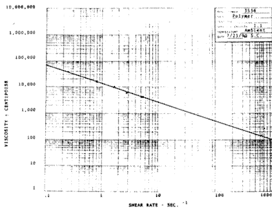
Figure 5. A Plot of Fluid Viscosity Vs Shear Rate is Required in Order to Accurately Size Pumps and Equipment for Non-Newtonian Fluid Applications.
