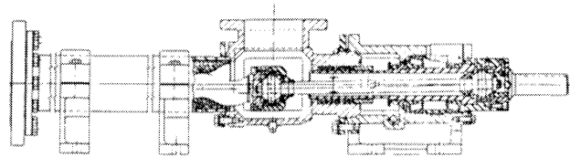
Figure 1. Cross Sectional View of a Typical Progressing Cavity Pump.
