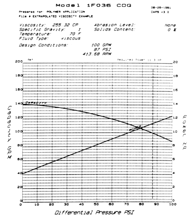
Figure 6. The Performance Data for a Pump Selected to Handle the Viscous Fluid Shown in Figure 5 Indicates the Viscosity of the Fluid As It Passes through the Pump Will Be Relatively Low.
