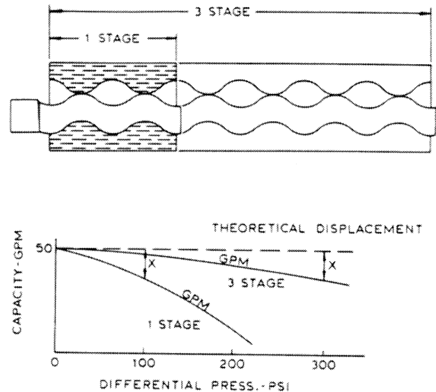
Figure 3. The Number of Stages Determines the Pressure Capability of a Progressing Cavity Pump.
