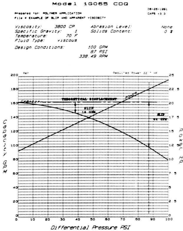
Figure 4. As the Differential Pressure Increases in a Progressing Cavity Pump, the Internal Leakage or Slip Also Increases.
