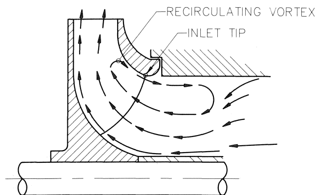
Figure 5. Suction Recirculation.
