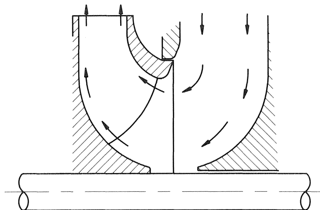
Figure 3. Radial Suction Impeller.
