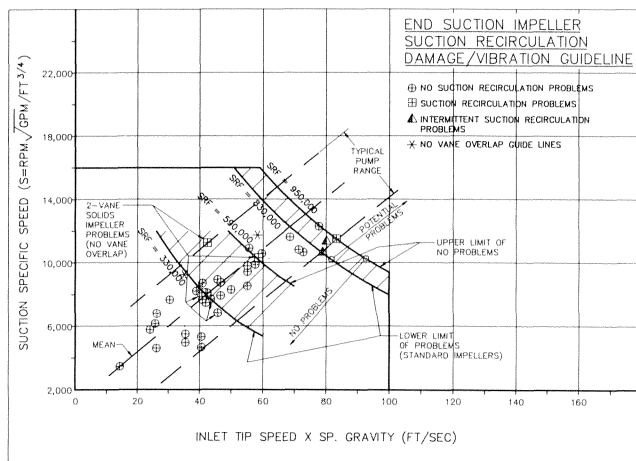
Figure 7. End Suction Impeller, Suction Recirculation Damage/Vibration Guide Line.
