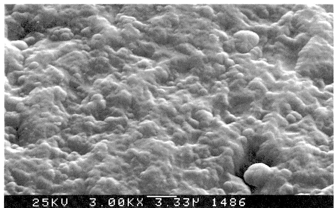
Figure 2. SEM Micrograph of Topography of DLC Coating on SSiC, Coating DLC4.
