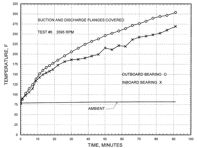
Figure 7. Bone-Dry Run Test with Flanges Covered—SiC(P) ADLC Stationary and Rotating Bearings.
