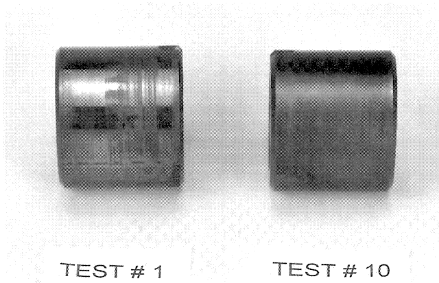
Figure 12. Comparison of Outboard Sleeve Bearing Condition-Tests 1 and 10.
