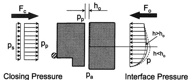
Figure 4. Operating Principle of Spiral Groove Hydrodynamic Seal.
