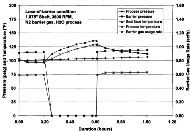
Figure 16. Twin Hybrid Seal Test Results at Abnormal Condition.
