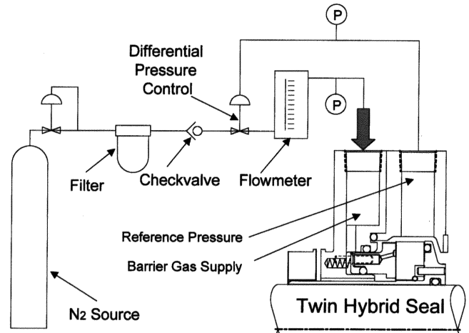
Figure 14. Barrier Gas Control Schematic for Laboratory Tests.
