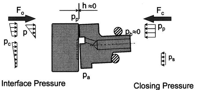
Figure 11. Principle of Operation—Loss-of-Barrier Condition.
