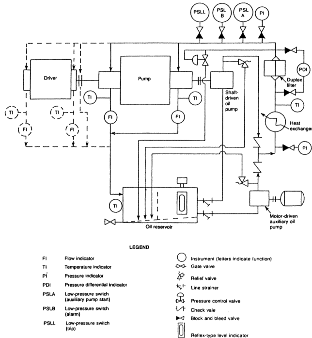
Figure 1. API 610, Eighth Edition, Lube Oil System Schematic. (Used with permission of API)
