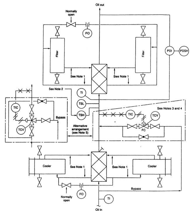
Figure 6. Duplex Filter with Transfer Valve.
