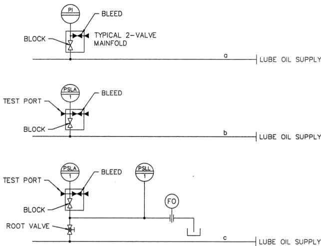
Figure 10. Instrument Valving.
