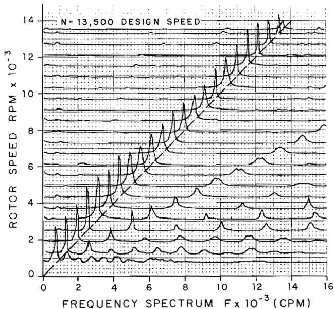
Figure 5-3. Frequency Spectrum Speed vs Speed with Squeeze Film Dampers — Stabilized System.
