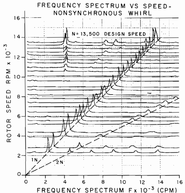
Figure 5-2. Frequency Spectrum vs Speed — Nonsynchronous Whirl.
