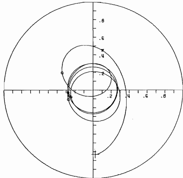
Figure 4-8. Vertical Unbalanced Rotor in Squeeze Film Bearing — Effect of Unbalance Magnitude — Unbalance Eccentricity — 1.75 Mil.
