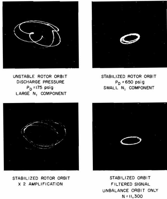
Figure 5-1. Rotor Orbits of a Turbo Compressor Before and After Stabilization by Damper Supports.
