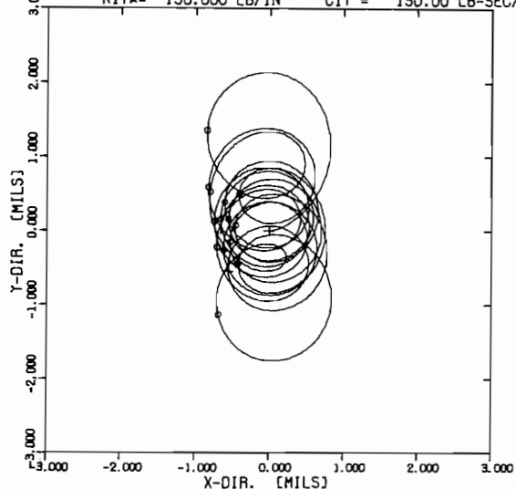
Figure 4-3. Stabilized Motion with Damper Support at 10,000 RPM ( C_i=20 , K_1=130,000 lb/in, C_1=150 lb-sec/in).
