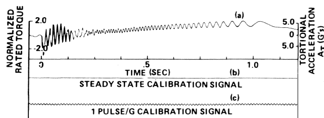
Figure 12. Measured Air Gap Torque During Start-up.
