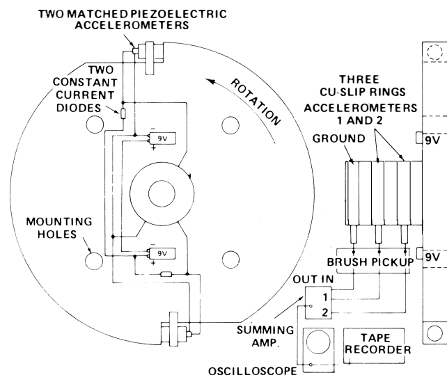
Figure 8. Torsional Acceleration Monitor.
