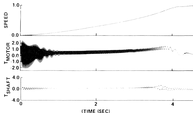
Figure 11. Simulation of Start-up.
