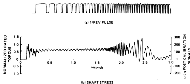
Figure 13. Measured Main Drive Shaft Stress During Start-up.
