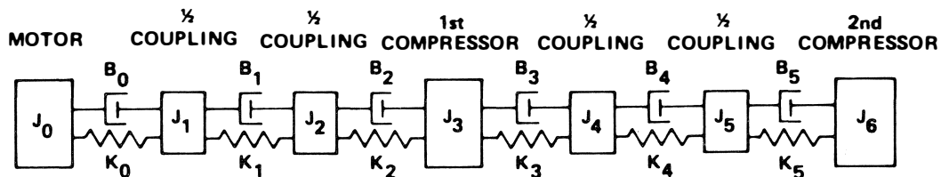
Figure 4. Mass-Elastic System.
