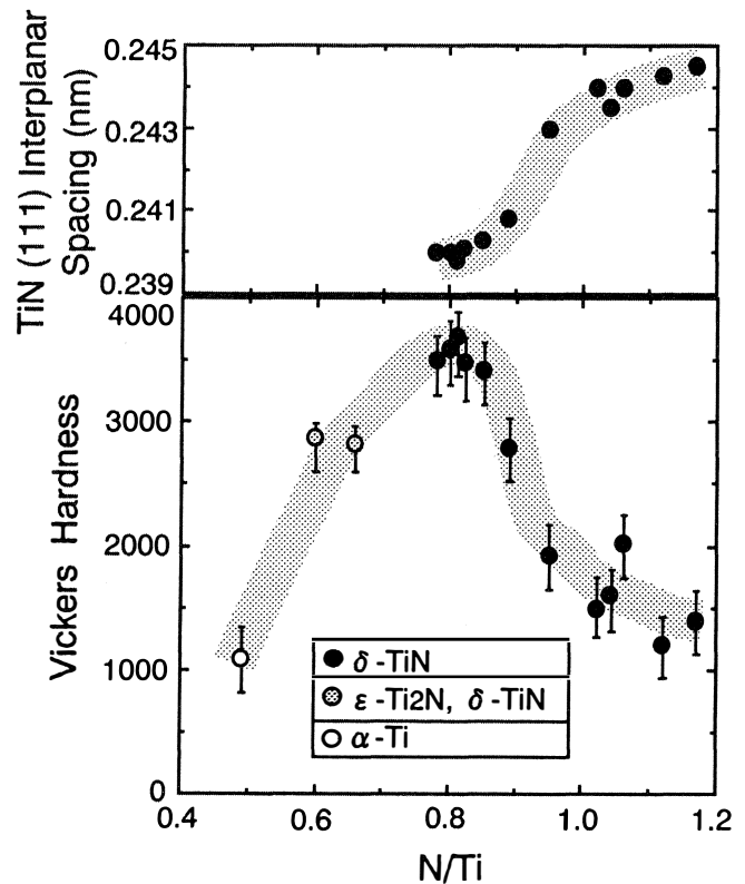
Figure 4. Relationship Between Compositional Ratio N/Ti and Vickers Hardness, TiN (111) Interplanar Spacing.
