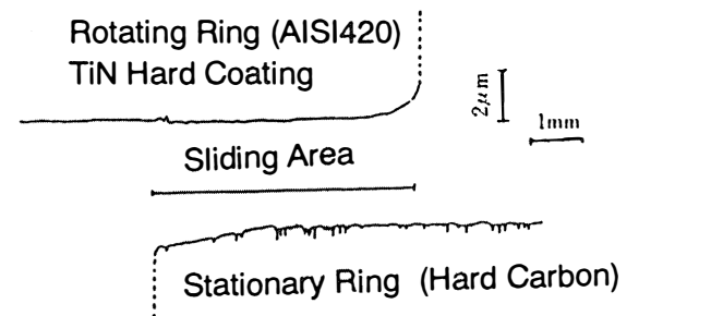
(a) TiN hard coating by Dynamic Ion Beam Mixing
