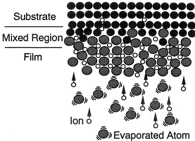
Figure 2. Schematic Diagram of Film Formation Mechanism by Dynamic Ion Beam Mixing Process.
