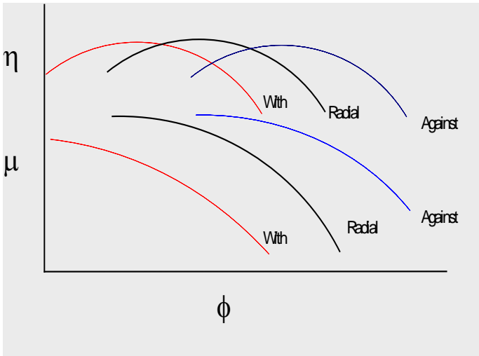
Figure 12. Effect of Prewhirl on Stage Performance
