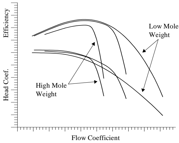
Figure 23. Variation in Stage Characteristics with Mole Weight (Fixed Stage Geometry at Constant Speed)
