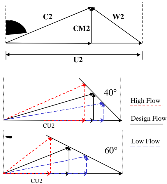
Figure 9. Impeller Exit Velocity Triangles – (a) nomenclature; (b) 40° backsweep; (c) 60° backsweep
