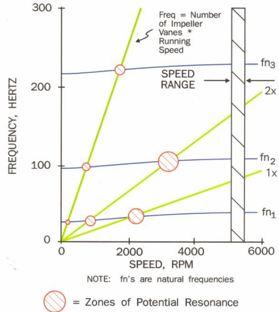
Figure 15. Typical Campbell Diagram, Showing Torsional Stiffness Increase with Load
