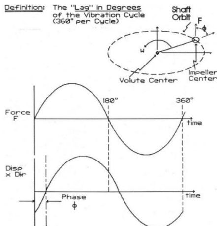
Figure 2. Definition of Phase Angle
