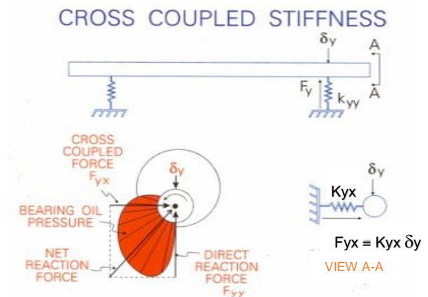
Figure 10. Cross-Coupled Stiffness
