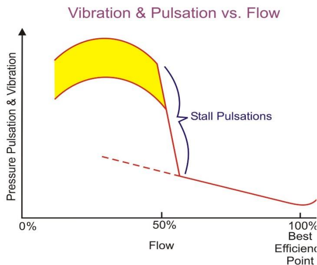
Figure 11. Effect on Vibration on Off-BEP Operation
