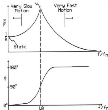
Figure 3. Relationship of Phase Angle to Frequency
