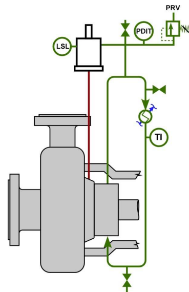
Figure 4. Plan 53C
