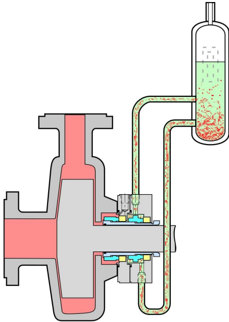
Figure 8. Process Fluid SG Greater Than Buffer Fluid
