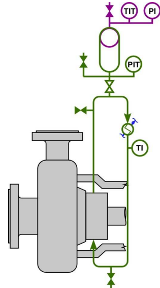
Figure 3. Plan 53B
