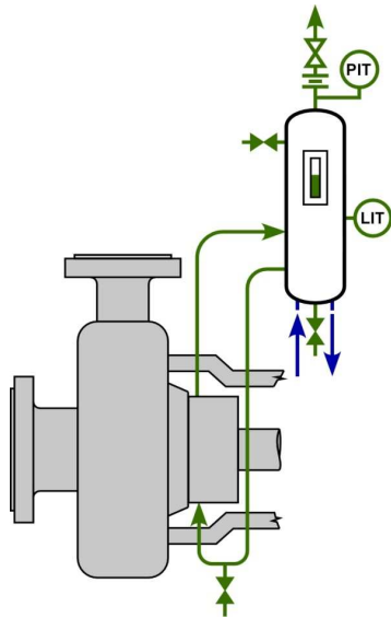
Figure 1. Plan 52
