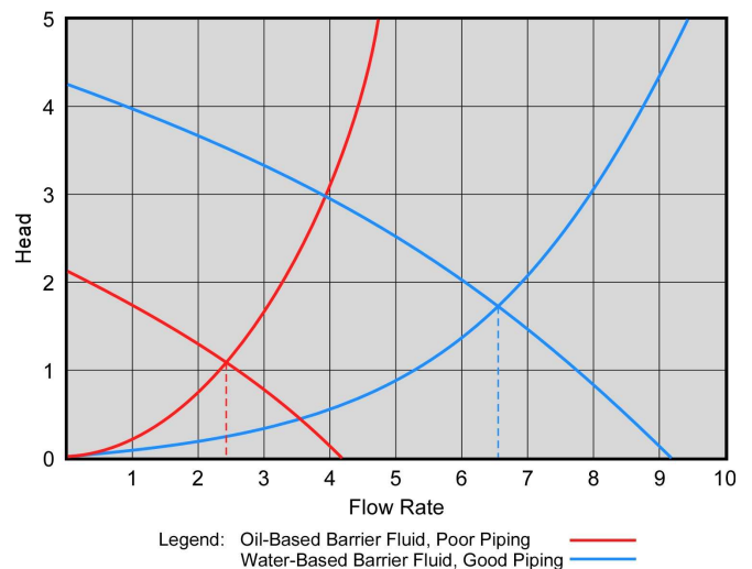
Figure 14. Combined Pumping Ring and System Curves
