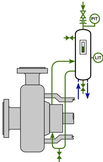
Figure 2. Plan 53A
