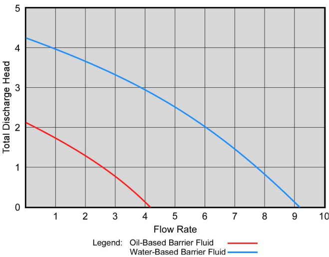
Figure 12. Representative Pumping Ring Curve
