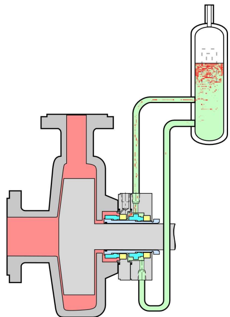
Figure 7. Process Fluid SG Less Than Buffer Fluid
