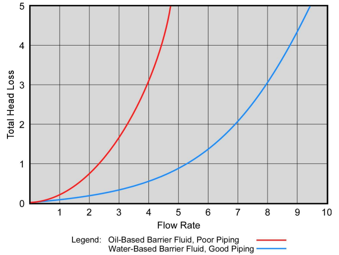
Figure 13. Representative Dual Liquid Seal System Curve
