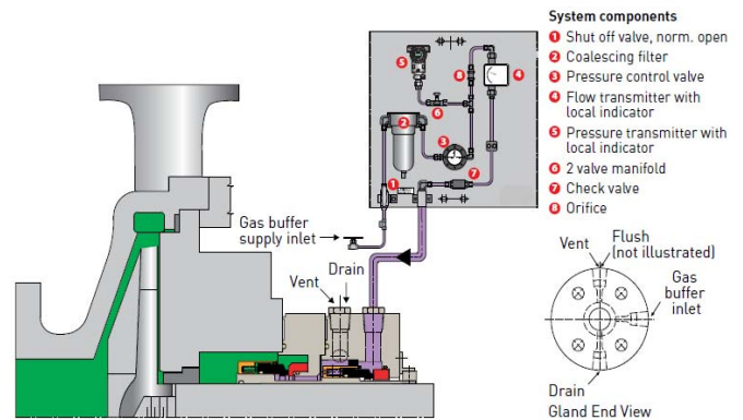
Figure 5 – API Plan 72 Panel Layout
