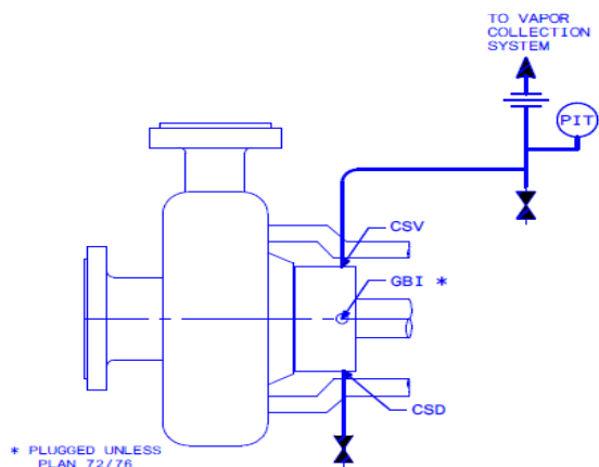
Figure 8 – Plan 76 Schematic
