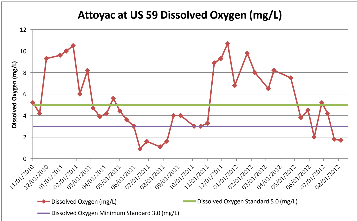
Figure C-12. Attoyac at US 59 Dissolved Oxygen (mg/L) measurements from 7/26/2010 through 8/20/2012.
