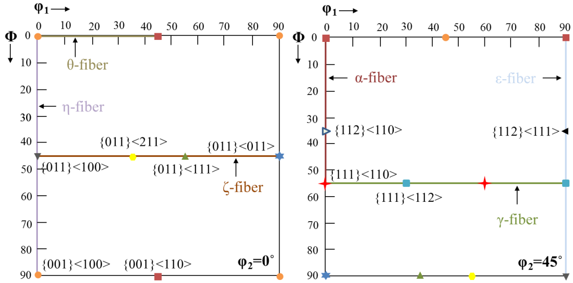
Figure 6.6 Schematic illustration of the important texture components in bcc materials (Reproduced from Ref [257]).
