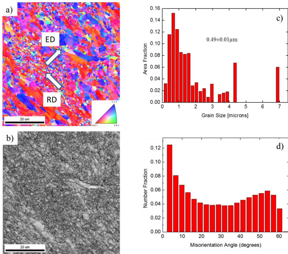
Figure 6.8 EBSD characterization of the intermediate tube alloy condition showing (a) an orientation map of the crystallographic distribution of the grains; (b) a band contrast map of the grain structure in gray scale; (c) the grain area distribution as a function of size; and, (d) the grain boundary misorientation angle distribution.
