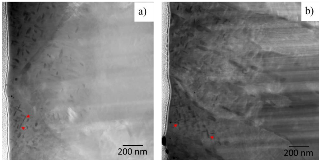
Figure 5.6 HAADF images of (a) as-received (b) as-shocked samples after 600 dpa irradiation. Arrows show the needle-like precipitate formation as a result of irradiation.
