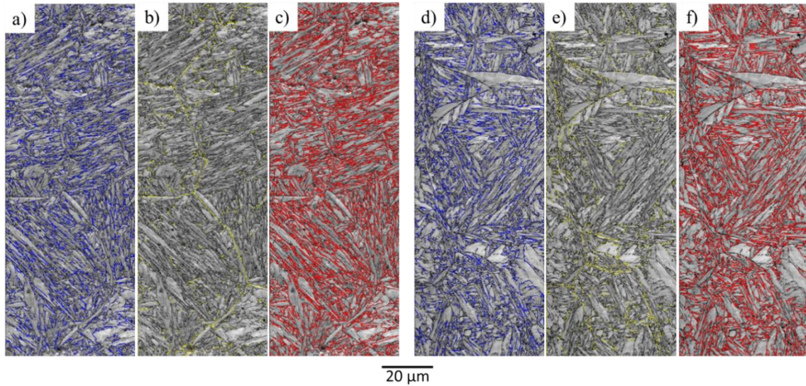
Figure 4.6 EBSD images of the as-received HT-9 steel showing the misorientation angles of (a) 2^{\circ} - 15^{\circ} (LAB), (b) 15^{\circ} - 50^{\circ} (RGB) and (c) 50^{\circ} - 65^{\circ} (special boundaries); as-shocked HT-9 steel showing the misorientation angles of (d) 2^{\circ} - 15^{\circ} (LAB), (e) 15^{\circ} - 50^{\circ} (RGB) and (f) 50^{\circ} - 65^{\circ} (special boundaries).
