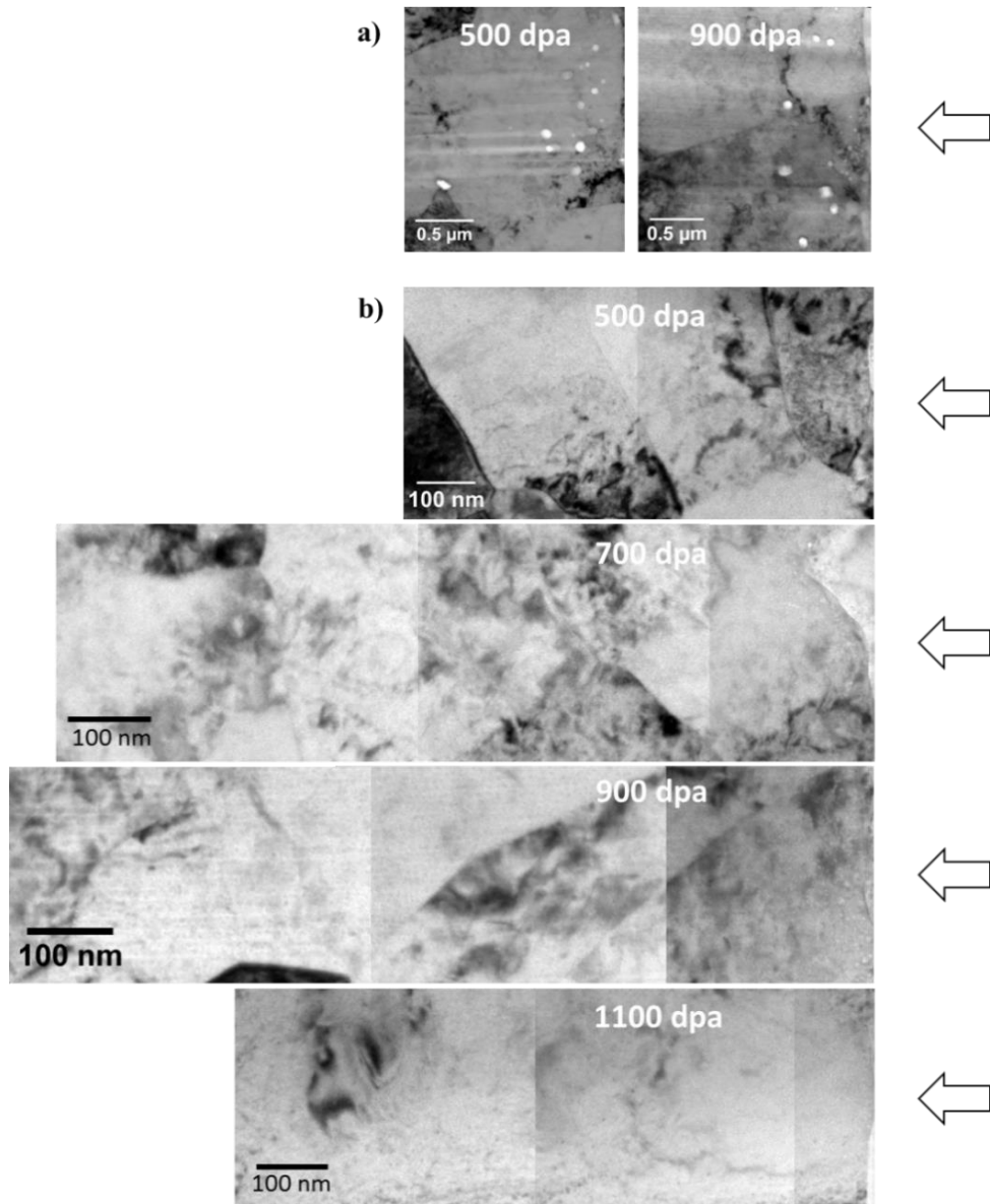
Figure 7.14 Microstructures of (a) Process I tube after 500 and 900 dpa (b) Process II tube after 500, 700, 900 and 1100 dpa irradiations with \text{Fe}^{2+} at 450 °C. Arrows indicate the direction of ion beam. Images were taken at 1 μm under focus condition.
