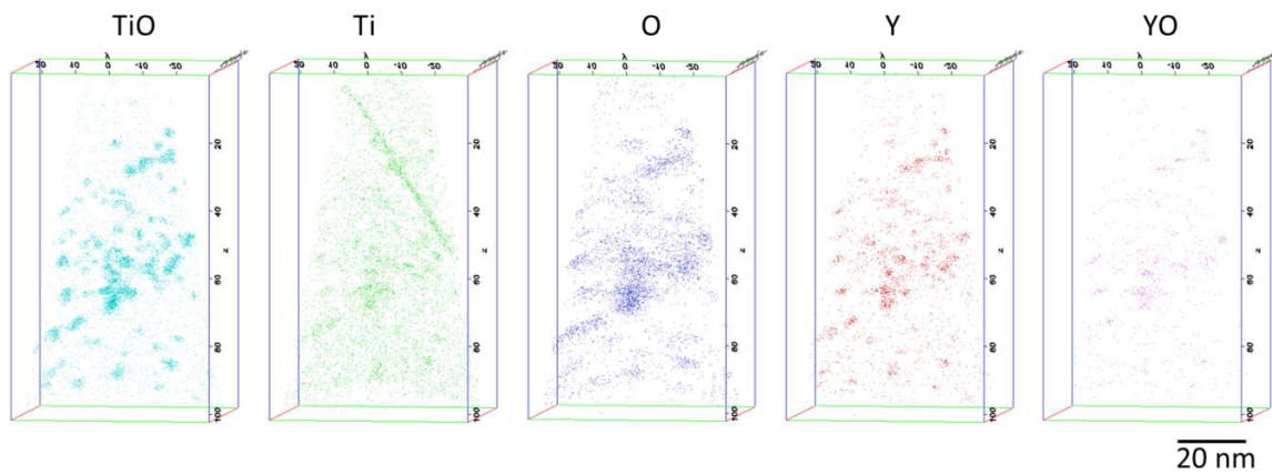
Figure 8.7 APT 3D reconstruction of unirradiated 14YWT samples showing distribution of various elements and ions.
