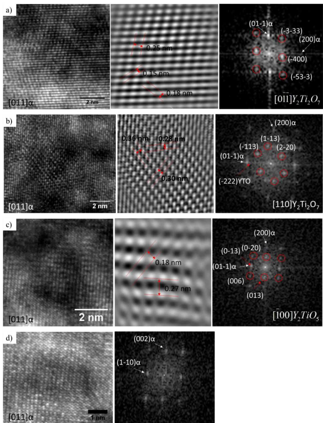
Figure 8.6 (a) HRTEM micrographs and corresponding FFT diagrams of (a) Y 2 Ti 2 O 7 particle having OR of (\bar{4}00)\alpha \parallel (200)Y_2Ti_2O_7 and [011]\alpha \parallel [01\bar{1}]Y_2Ti_2O_7 ; (b) Y 2 Ti 2 O 7 particle having OR of (01\bar{1})\alpha \parallel (\bar{2}22)Y_2Ti_2O_7 and [011]\alpha \parallel [110]Y_2Ti_2O_7 ; (c) Y 2 TiO 5 particle having OR of (002)\alpha \parallel (\bar{2}10)Y_2TiO_5 and [110]\alpha \parallel [001]Y_2TiO_5 ; (d) an unknown particle with no extra diffractions.
