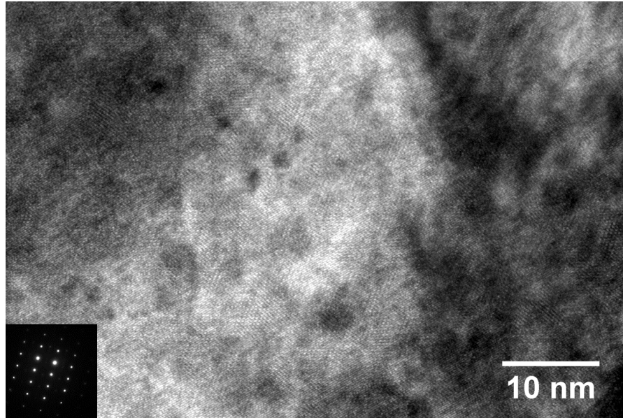
Figure 8.9 HRTEM image showing the NF distribution along [110] zone axis of the matrix after 480 dpa irradiation.
