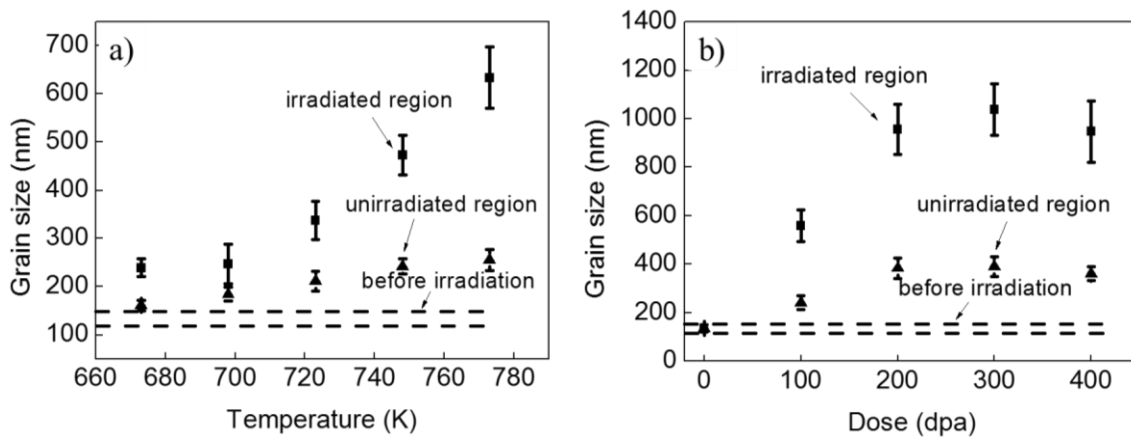
Figure 3.10 (a) Temperature dependence of mean grain size at 100 peak dpa (b) dose dependence of mean grain size at 475 °C in irradiated and unirradiated regions of severely deformed EK-181 samples.
