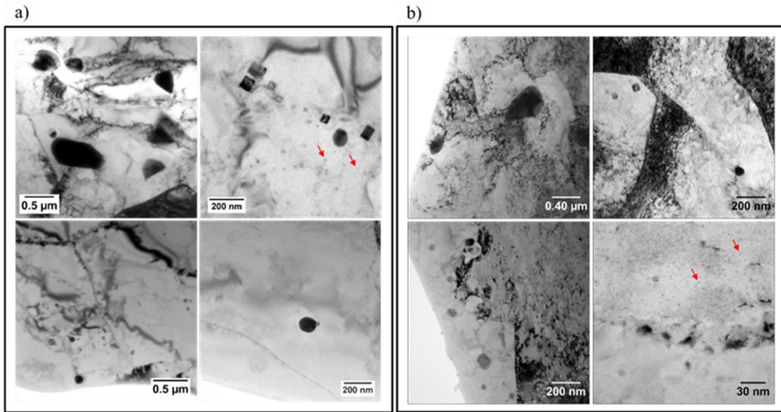
Figure 7.2 Bright field TEM images showing the second phase particle size and distribution in 14YWT tubes produced by (a) Process I and (b) Process II.
