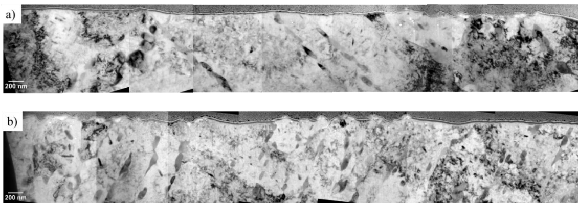
Figure 5.4 Stitched BFTEM images of (a) as-received (b) as-shocked samples irradiated to 600 dpa. Images were taken at \sim 1 \mu\text{m} under-focus condition.
