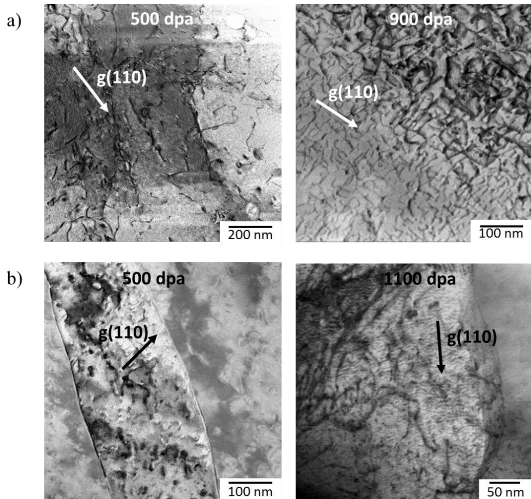
Figure 7.18 BF-STEM images showing dislocation loop distribution in two-beam condition ( g=(110) ) for (a) Process I tube irradiated up to 500 and 900 peak dpa doses (b) Process II tubes irradiated up to 500 and 1100 peak dpa dose.
