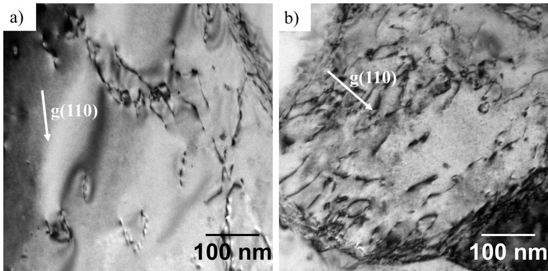
Figure 7.13 TEM bright field images of (a) Process I and (b) Process II tubes along g(110) direction showing the distribution of dislocations.
