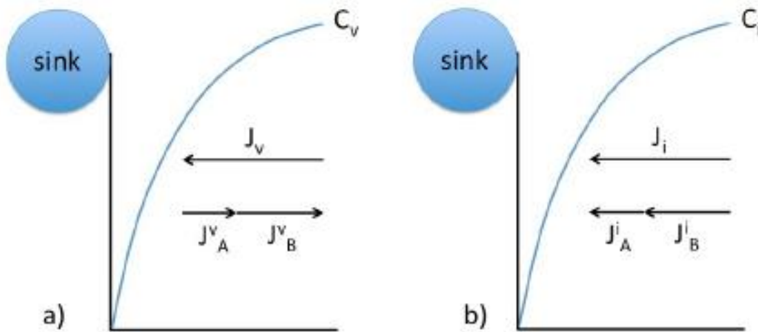
Figure 1.4 RIS by (a) vacancy mechanism and (b) interstitial mechanism. The length of the arrows represent the magnitude of the fluxes for A and B atoms [21].
