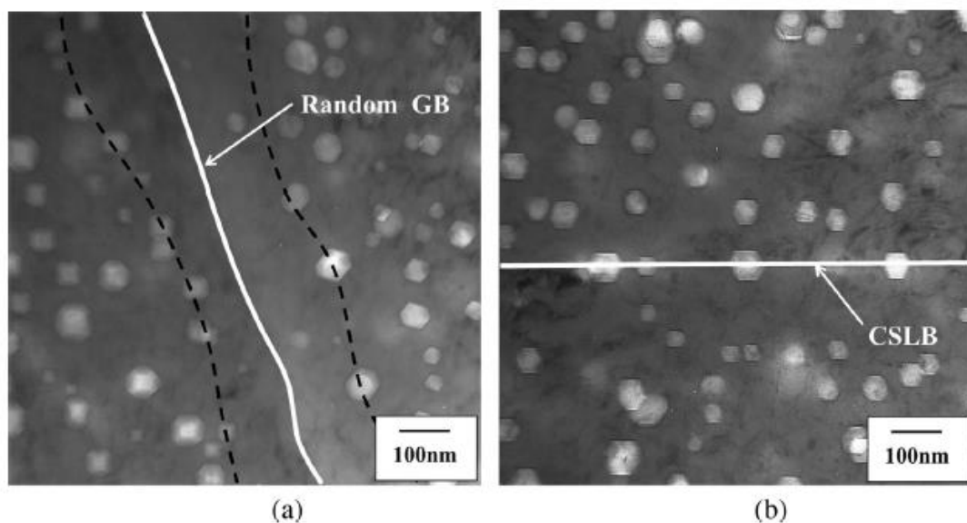
Figure 1.14 Void distributions in the Fe–15Cr–15Ni steel neutron-irradiated at 749 K to 18 dpa near the (a) random GB (b) CSLB. The black dashed lines represent the region of void denuded zone [63].
