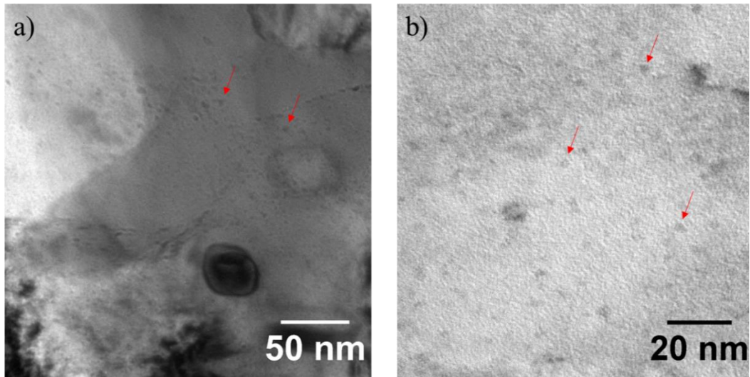
Figure 8.2 Distribution of particles before irradiation. (a) Low magnification BF TEM image showing both larger particles together with NFs (b) high magnification image showing the NF distribution.
