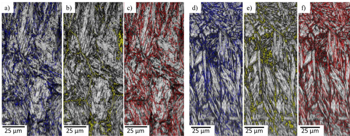
Figure 5.1 EBSD images of the as-received HT-9 steel showing the misorientation angles of (a) 2^\circ - 15^\circ (LAB), (b) 15^\circ - 50^\circ (RGB) and (c) 50^\circ - 65^\circ (special boundaries); as-shocked HT-9 steel showing the misorientation angles of (d) 2^\circ - 15^\circ (LAB), (e) 15^\circ - 50^\circ (RGB) and (f) 50^\circ - 65^\circ (special boundaries) after irradiation to 600 dpa.
