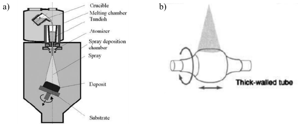
Figure 1.18 (a) A typical spray forming set up and principle [81] (b) tubular preform produced by spray forming [83].
