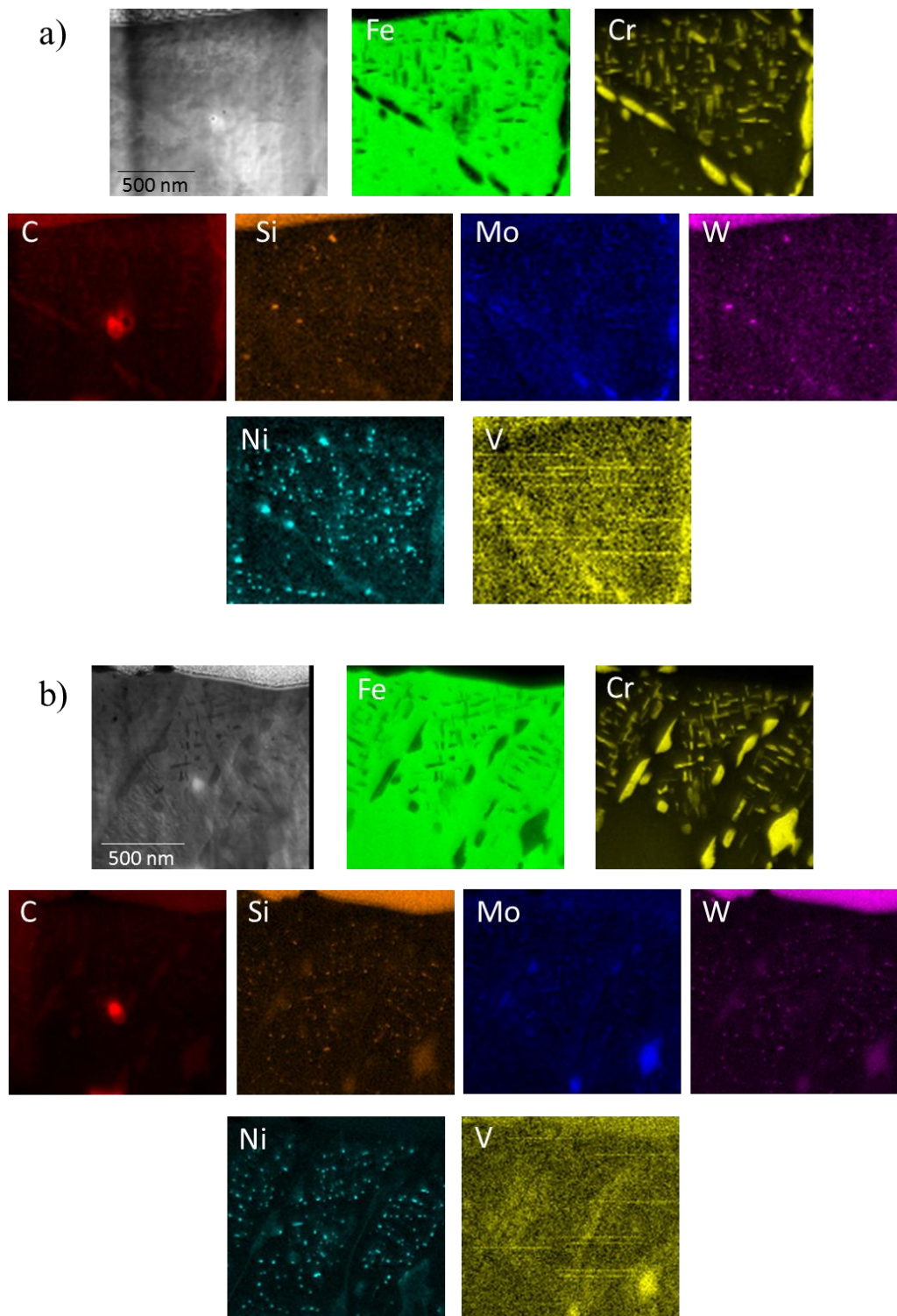
Figure 5.7 STEM EDS mapping of (a) as-received (b) as-shocked HT-9 samples irradiated to 600 dpa.
