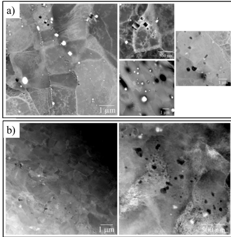
Figure 7.3 High-angle annular dark field (HAADF) scanning transmission electron microscopy (STEM) image showing large, medium and small size particles in 14YWT tubes produced by (a) Process I and (b) Process II.
