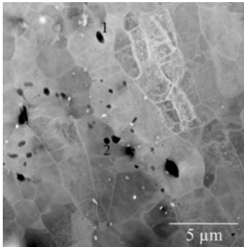
Figure 7.6 Composition analysis of ellipsoidal or polygonal dark particles having sizes between 10 nm and up to 1 μm in Process I tube.
