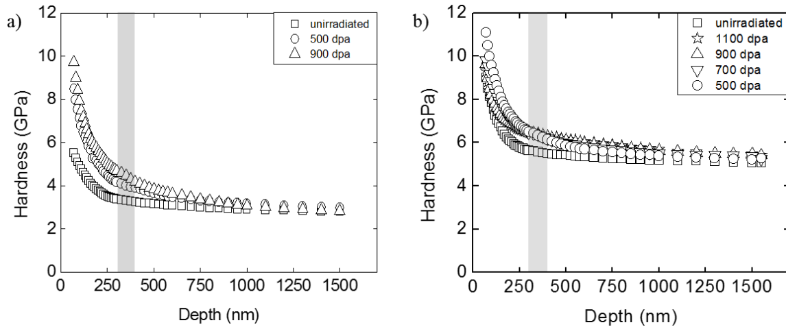
Figure 7.17 Hardness as a function of penetration depth for (a) Process I tube after 500 and 900 dpa (b) Process II tube after 500, 700, 900 and 1100 dpa irradiations with \text{Fe}^{2+} at 450^\circ\text{C} . Shaded regions between 300-400 nm depth shows the region of investigation.
