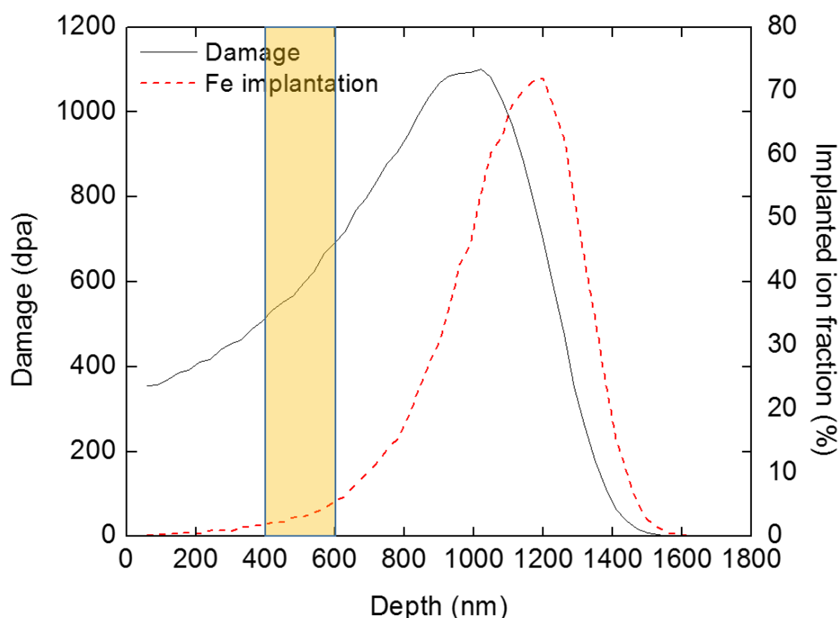
Figure 8.1 SRIM-calculated depth profiles of damage and implanted Fe atoms for 1100 peak dpa irradiation in pure Fe.
