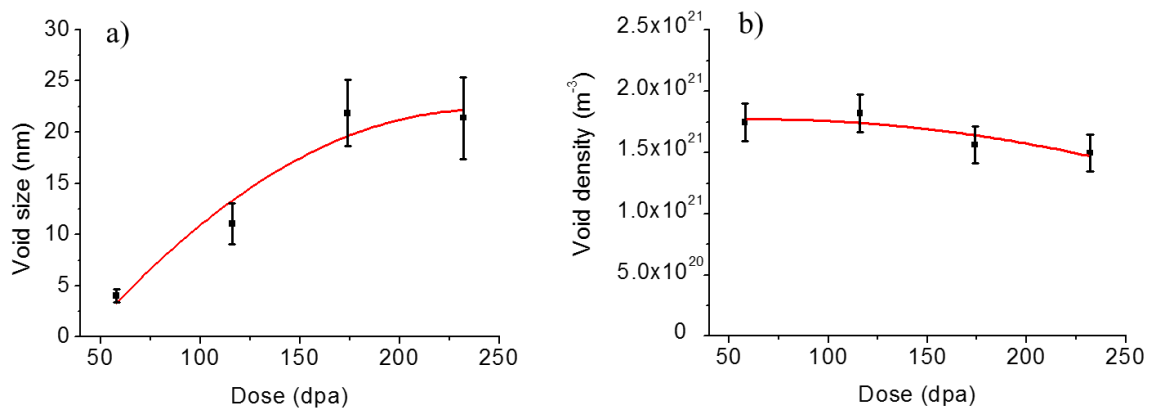
Figure 3.6 Plots of (a) void size and (b) void density as a function of local dpa for severely deformed EK-181. Measurements were performed at a depth region between 400 to 700 nm.
