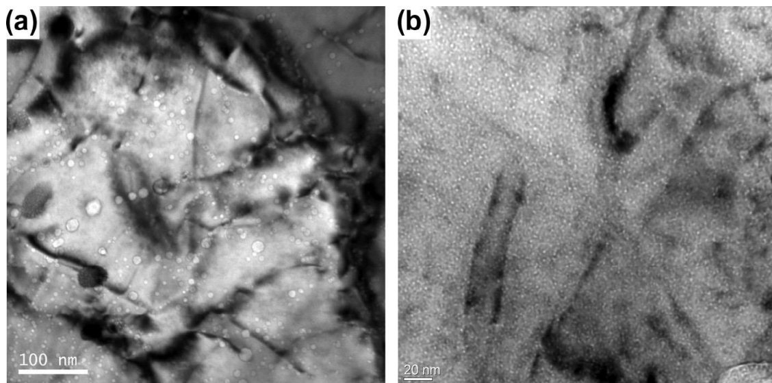
Figure 1.15 Under-focused bright field TEM images of the dual ion beam irradiated cavity structures in (a) F82H and (b) MA957 irradiated to 42 dpa and 2100 appm He at 500 °C (at 1000 nm from the surface) [64].
