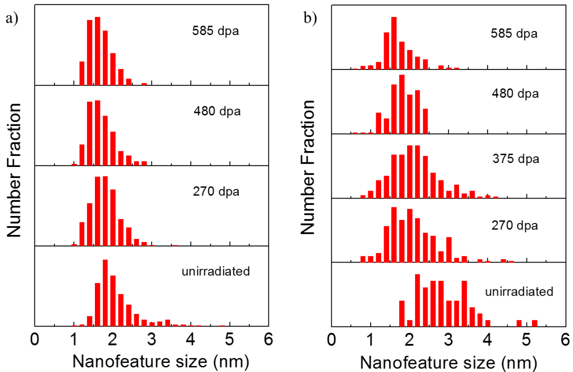
Figure 8.13 NF size distribution in unirradiated and various dose irradiated samples obtained by (a) APT and (b) TEM analyses.
