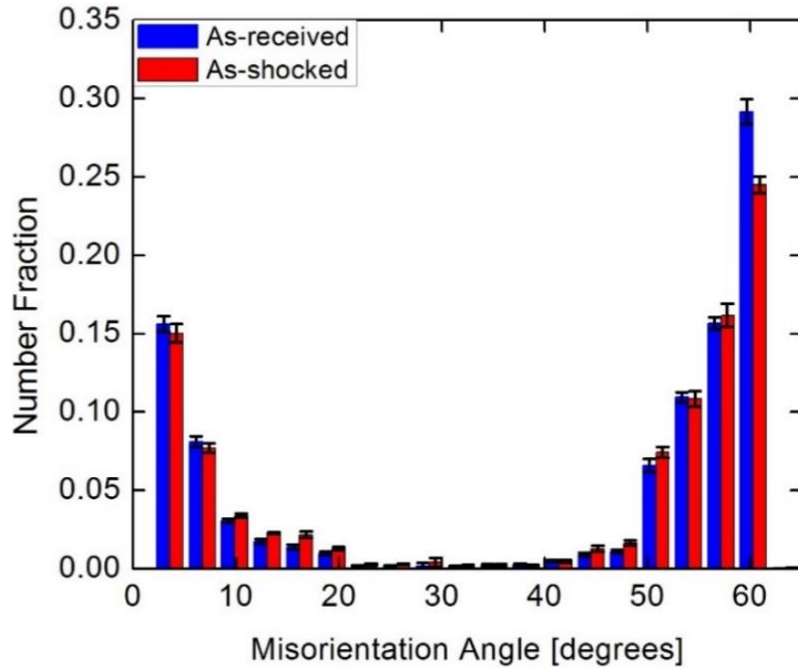
Figure 4.7 Histogram of misorientation fraction inside single primary austenite grains for the as-received and as-shocked HT-9 samples.
