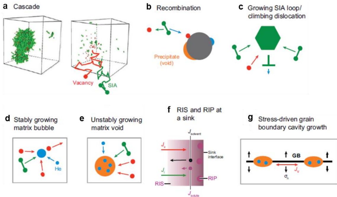
Figure 1.3 (a) Displacement cascade and generation of vacancies and self-interstitial atoms (SIAs) (b-e) Annihilation of defects either by recombination or at sinks (f) Radiation-induced segregation (RIS) and radiation-induced precipitation (RIP) at sinks. J_v : flux of vacancies, J_i : flux of SIAs, J_{\text{solute}} : flux of solutes and J_{\text{solvent}} : flux of solvents (g) Growth of the bubbles at the grain boundaries under stress-driven creep conditions [19].
