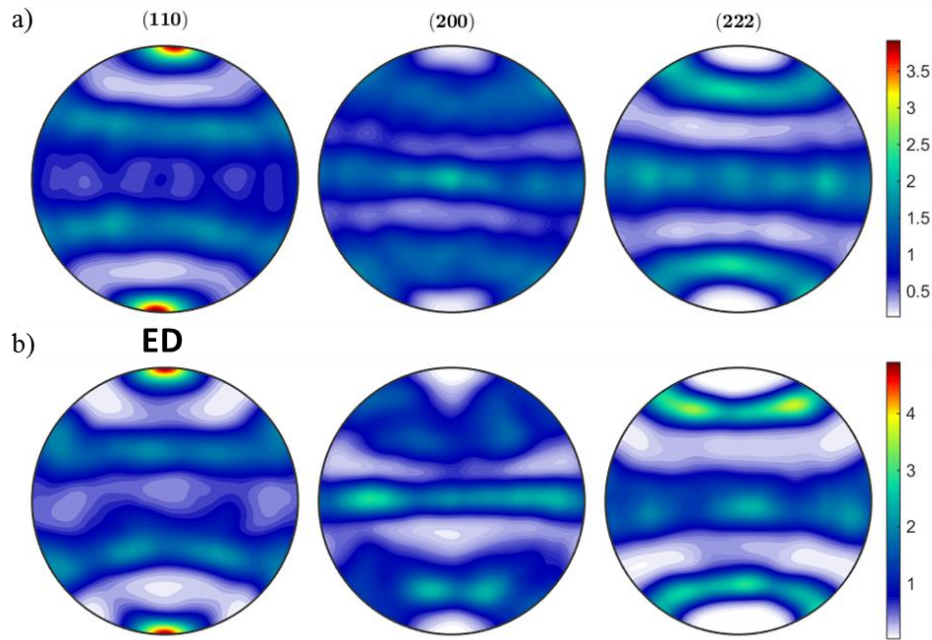
Figure 6.5 Pole figures of 14YWT samples produced by Process I and obtained by (a) Neutron diffraction and (b) EBSD techniques. (ED: extrusion direction)
