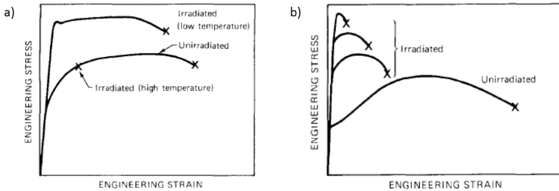
Figure 1.10 Effect of neutron irradiation on stress-strain curves of (a) fcc structure (austenitic steels) (b) bcc structure (ferritic steels) [17].
