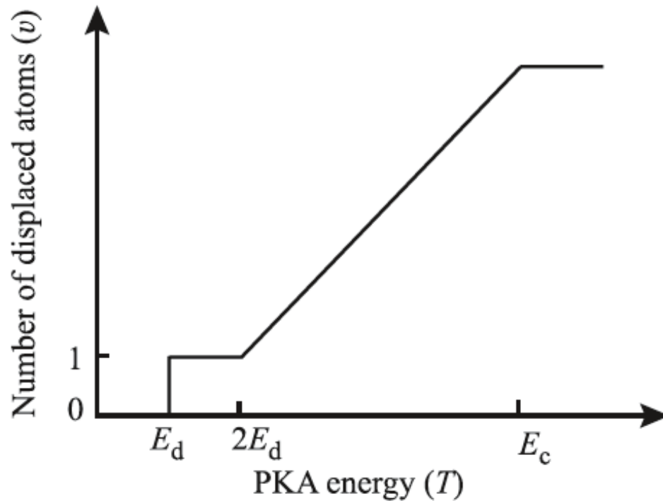
Figure 1.2 Graphical representation of Kinchin-Pease model [13].
