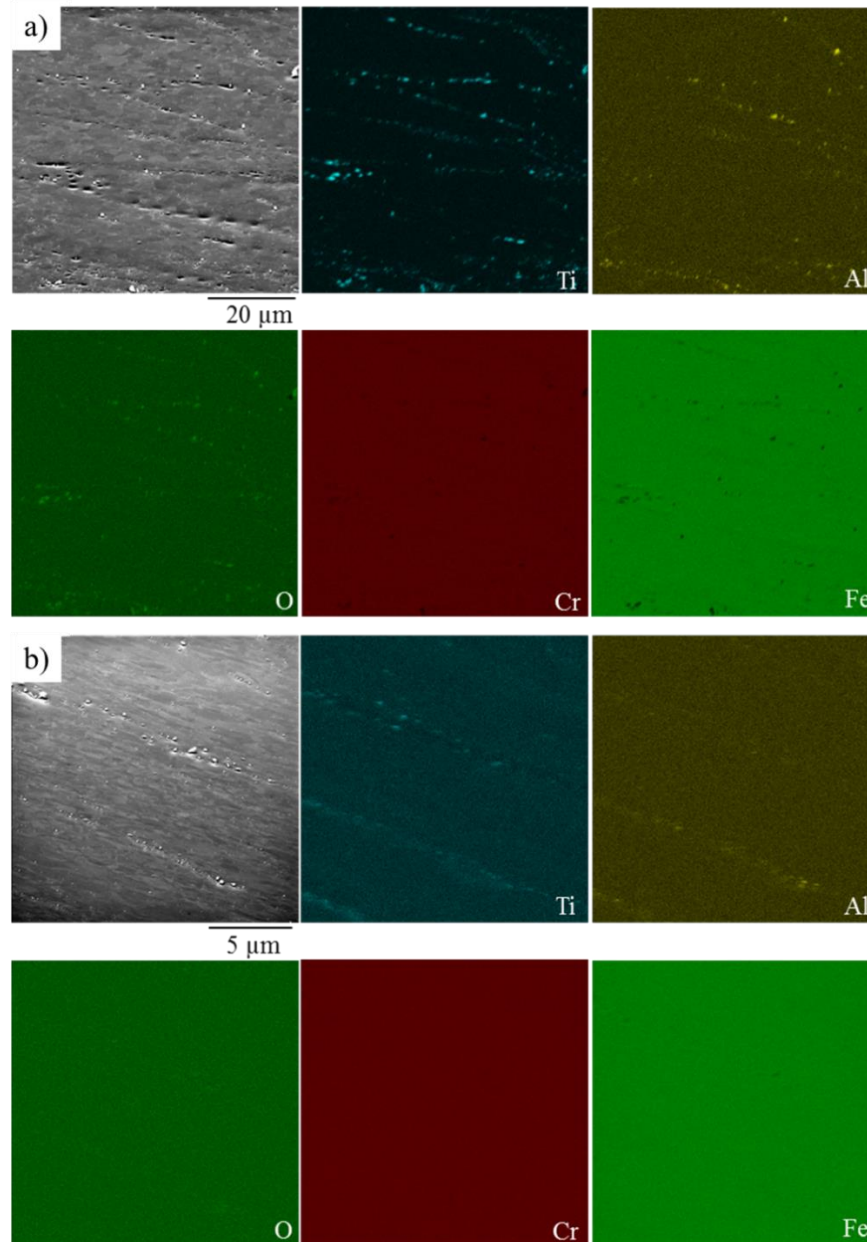
Figure 7.4 SEM-EDS mapping of various elements in 14YWT tubes produced by (a) Process I and (b) Process II. Large oxide particles are located at the grain boundaries and elongated in extrusion direction.
