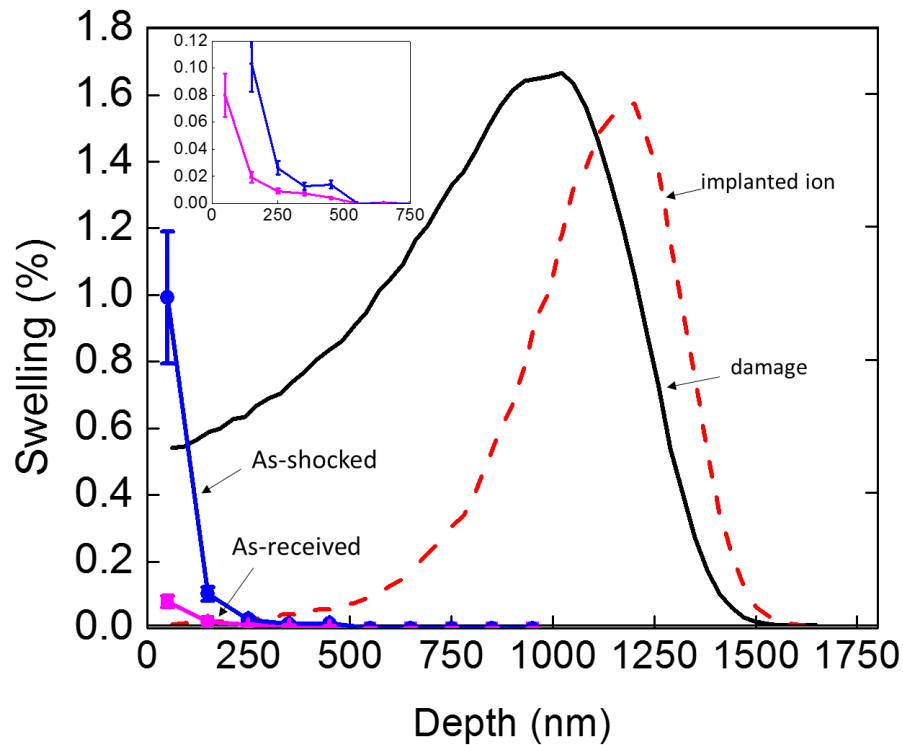
Figure 5.5 Swelling vs. depth profiles of the as-received and as-shocked HT-9 steels after 600 dpa irradiations. Swelling curves were superimposed on the SRIM-calculated dpa and injected Fe ion profiles.
