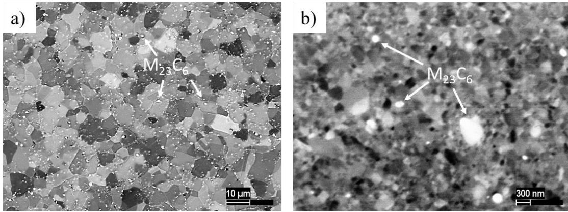
Figure 3.1 SEM images of (a) annealed EK-181 (b) HPT processed, severely deformed EK-181, showing the non-homogenous distribution of carbides along the grain boundaries on both variants. Typical M_{23}C_6 type carbides in bright contrast along the grain boundaries are shown by arrows. Note difference in scale of the two micrographs.
