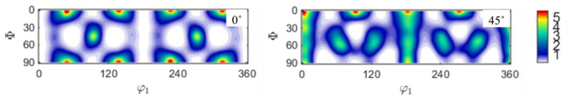
Figure 6.7 The neutron diffraction produced ODF, represented as sections in Euler space, for the 14YWT tube produced by process I at \varphi_2 values of 0^\circ and 45^\circ .
