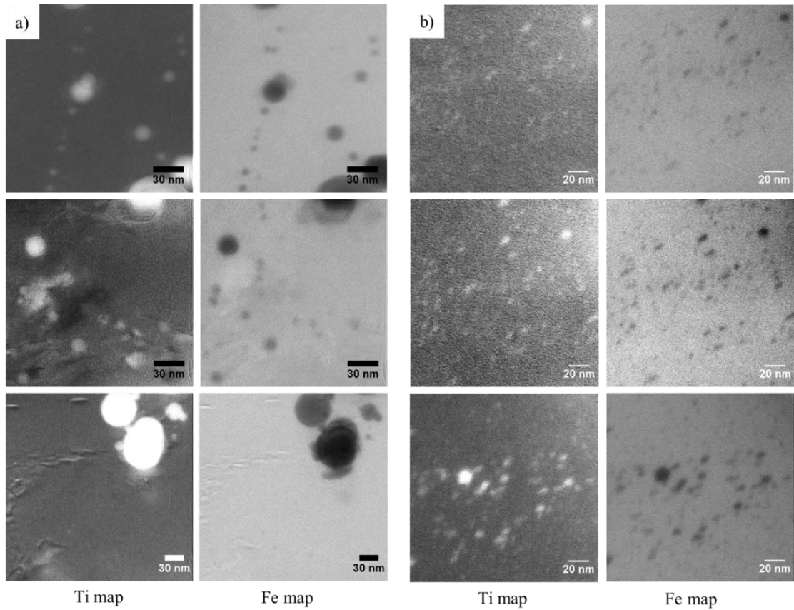
Figure 7.11 EFTEM Ti and Fe elemental maps obtained from the tubes produced by (a) Process I and (b) Process II.
