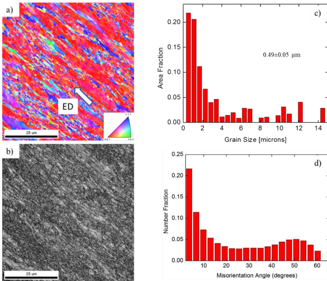
Figure 6.12 (a) Orientation map showing the crystallographic distribution of the grains; (b) band contrast map showing the microstructure in gray scale; (c) grain size distribution plot; and, (d) grain boundary misorientation angle distribution in 14YWT final tube produced by Process II.
