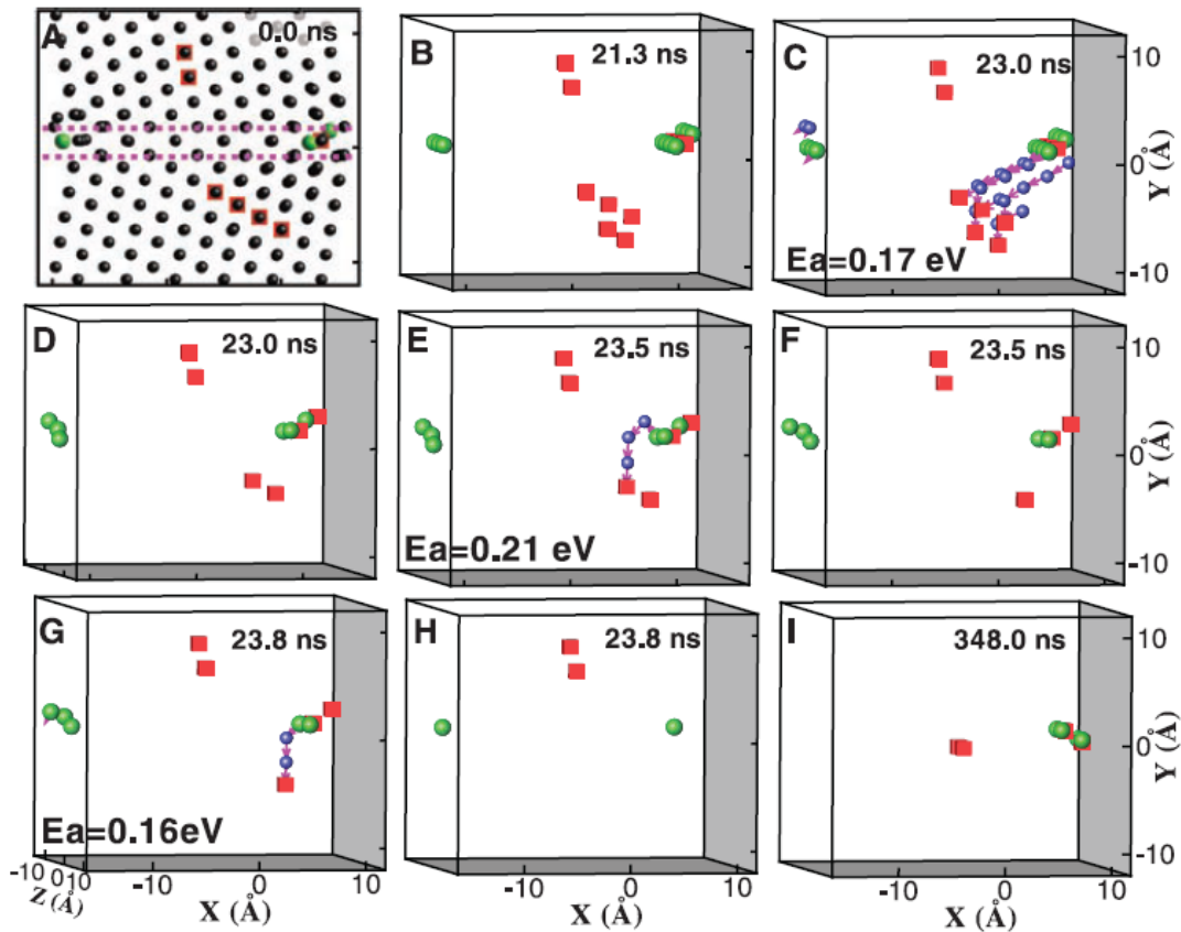
Figure 1.13 Temperature accelerated dynamics simulations of damage self-healing near the GB (within 10 \text{ \AA} of the GB). Smaller black spheres in A: nondefective atoms; larger green spheres: interstitials; red cubes: vacancies; smaller blue spheres: atoms that move more than 1 \text{ \AA} during an event; purple vectors: the moving directions and distances of moving atoms [59].
