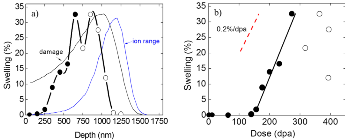
Figure 3.8 (a) Depth dependent swelling of annealed specimen after 400 peak dpa irradiation and (b) swelling of the same sample as a function of its local dpa values.
