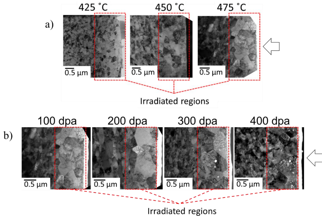
Figure 3.9 TEM micrographs showing extensive grain growth in the irradiated regions (a) for 100 peak dpa irradiation at different temperatures, and (b) for different dose levels at 475 °C. Arrows refer to the beam bombardment direction.
