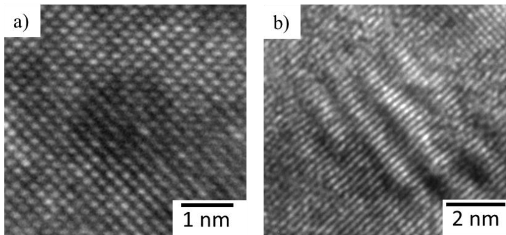
Figure 8.3 HRTEM images of (a) coherent small NF having the size \sim 1.5 nm (b) semicoherent larger \sim 5 nm NF showing misfit Moiré fringes.
