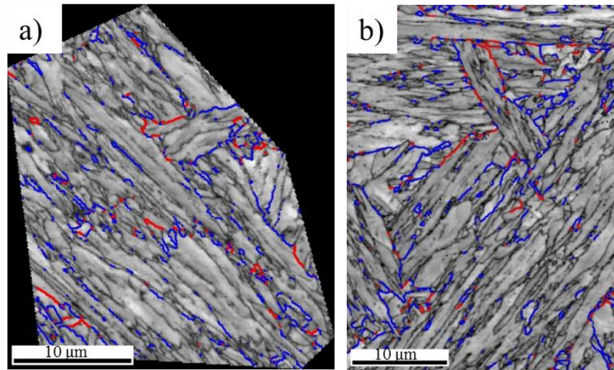
Figure 4.8 Misorientation angles between the packets of (a) as-received (b) as-shocked HT-9 samples (— 10°-20°; — 47°-50°).
