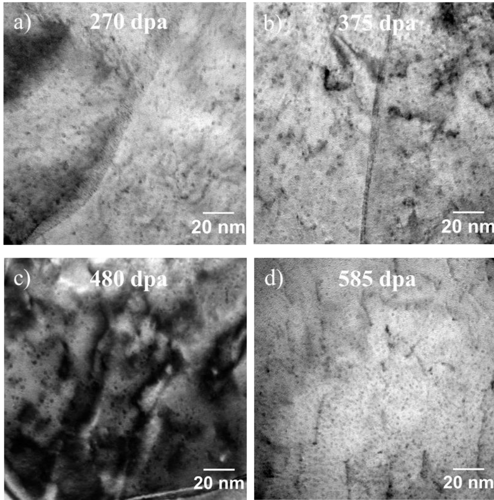
Figure 8.8 TEM images of samples collected from the depth region of 400 nm to 600 nm, after irradiation to (a) 270 dpa (b) 375 dpa (c) 480 dpa and (d) 585 dpa at 450 °C.
