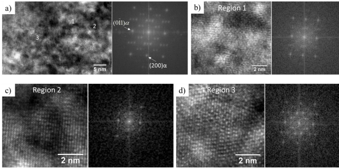
Figure 8.5 (a) HRTEM micrograph of a region and its corresponding FFT diagram along [110]\alpha ; HRTEM images and corresponding FFTs from (b) region 1, (c) region 2, (d) region 3 as labelled in (a).
