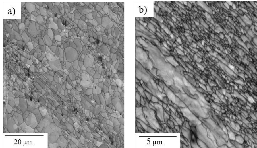
Figure 7.1 Band contrast maps showing the grain distribution for 14YWT tubes produced by (a) Process I and (b) Process II.
