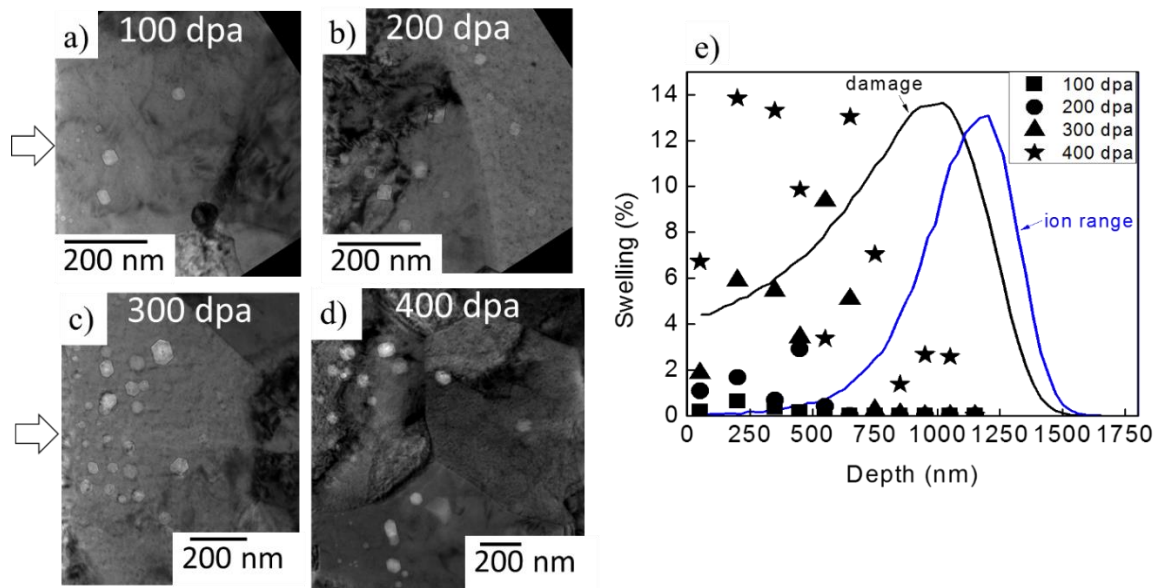
Figure 3.5 TEM micrographs of severely deformed EK-181 after irradiation to (a) 100 peak dpa, (b) 200 peak dpa, (c) 300 peak dpa, and (d) 400 peak dpa at 475 °C, and (e) corresponding depth profiles of swelling. Arrows refer to the beam bombardment direction.
