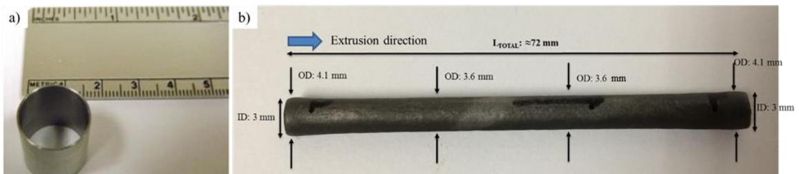
Figure 6.3 Photos showing the final dimensions of the tubes produced by (a) Process I, and (b) Process II.
