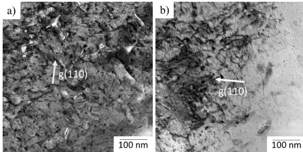
Figure 5.3 Bright field STEM images of (a) as-received (b) as-shocked conditions after 600 dpa irradiation along g=(110) direction.
