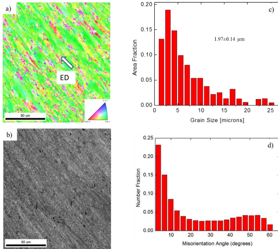
Figure 6.4 An OIM showing (a) the crystallographic orientation of the grains; (b) the corresponding band contrast gray scale map of the grain structure; (c) the grain area distribution as a function of the grain size; and, (d) the grain boundary misorientation angle distribution in 14YWT samples produced by Process I.
