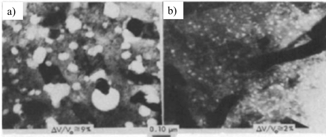
Figure 1.12 Micrographs illustrating the microstructures of (a) solution annealed austenitic stainless steel irradiated to 36 dpa at 520 °C and (b) 20% cold worked stainless steel irradiated to 54 dpa at 550 °C in HFIR [55].
