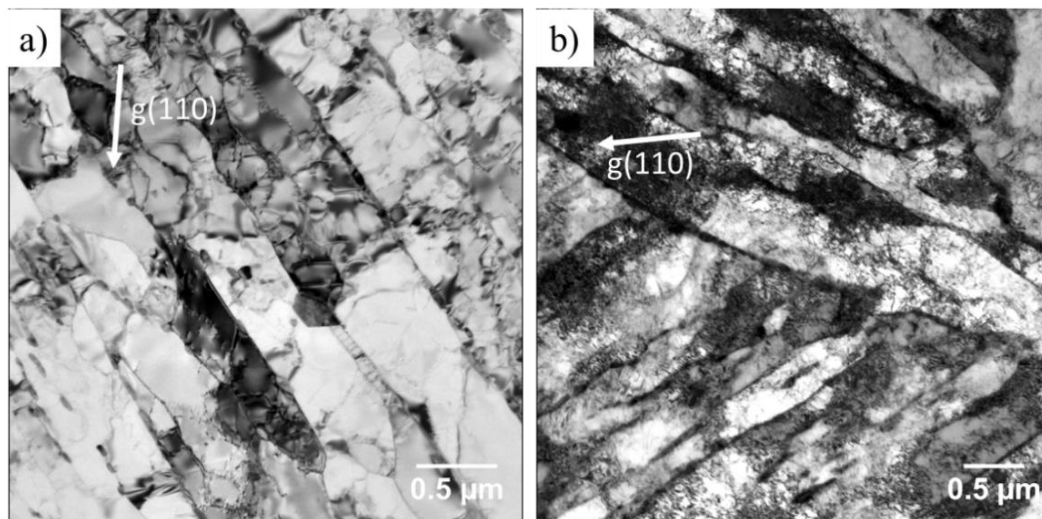
Figure 4.1 TEM bright field images of the (a) as-received sample (b) shocked loaded sample with the peak pressure of 11 GPa at room temperature.
