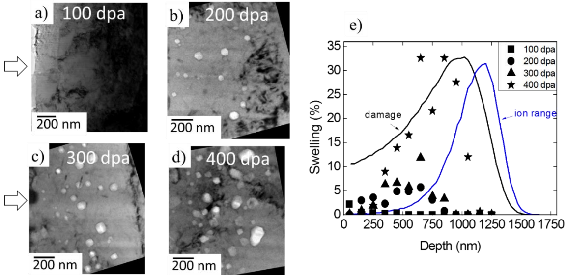
Figure 3.3 TEM images of annealed EK-181 samples irradiated to (a) 100 peak dpa, (b) 200 peak dpa, (c) 300 peak dpa, and (d) 400 peak dpa at 475 °C; and (e) swelling vs. depth profiles. Arrows refer to the beam bombardment direction.
