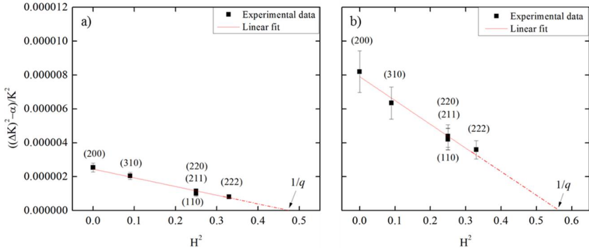
Figure 4.5 The modified Williamson–Hall plots of the FWHM for (a) as-received (b) as-shocked specimens. The Miller indices of the reflections are also indicated.
