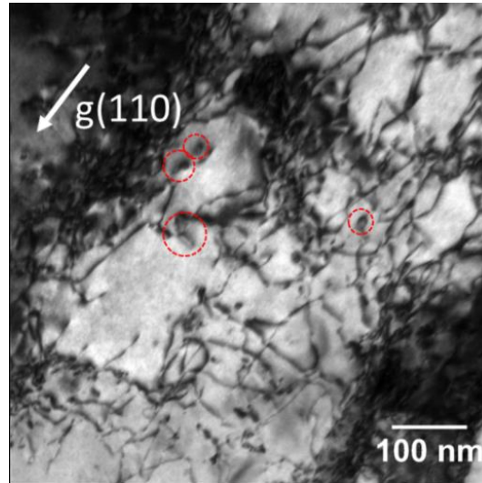
Figure 4.3 TEM bright field image of the as-shocked sample showing the dislocation structure and dislocation loops (red dashed circles) on g=(110) .
