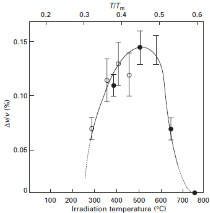
Figure 1.9 Swelling vs. irradiation temperature curve in nickel for a neutron fluence of 5 \times 10^{23} \text{ n/m}^2 [30].
