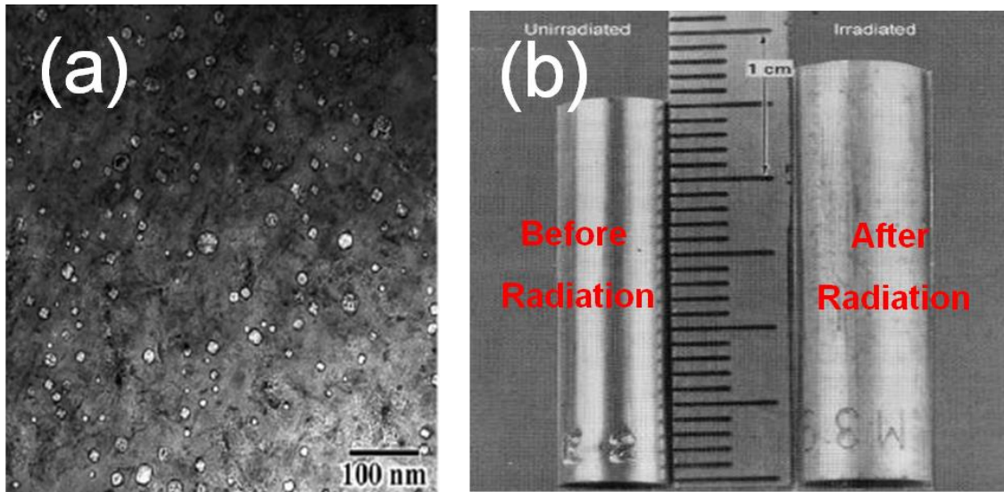
Figure 1.8 (a) Void formation in 304 austenitic stainless steel after neutron irradiation at 500 °C up to 10 dpa [27]. (b) Volume change in 316 stainless steel rods irradiated at 533 °C to a fluence of 1.5 \times 10^{23}/\text{m}^2 in the EBR-11 reactor [28].
