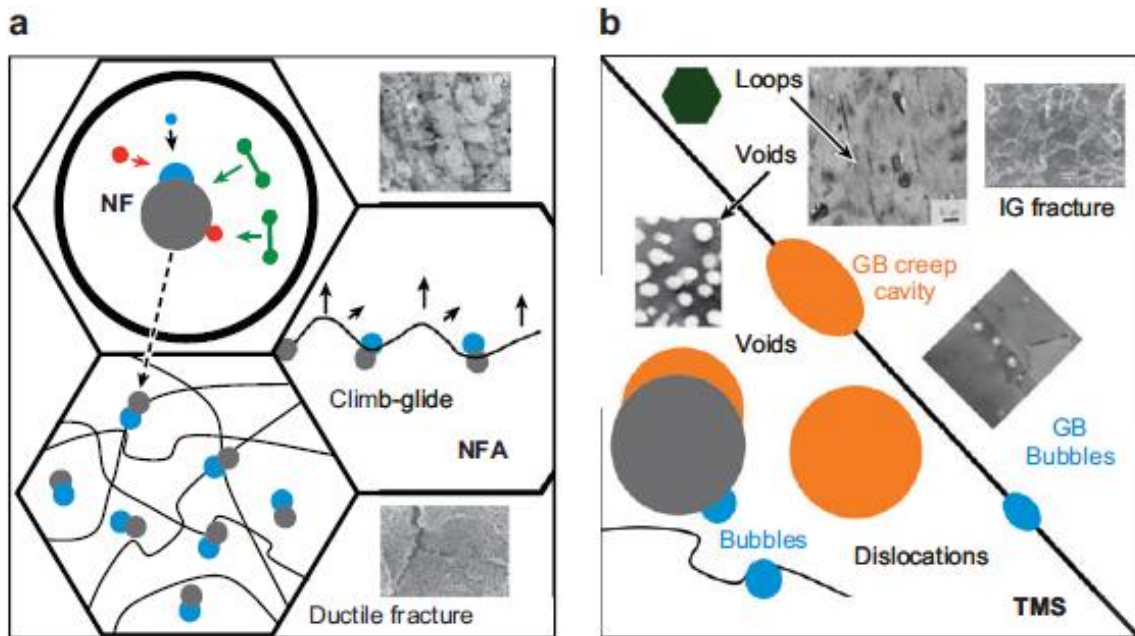
Figure 1.16 Schematic of irradiation effects in (a) nanostructured ferritic alloys (NFAs) (b) 9Cr normalized and tempered martensitic steels (TMSs) [19].
