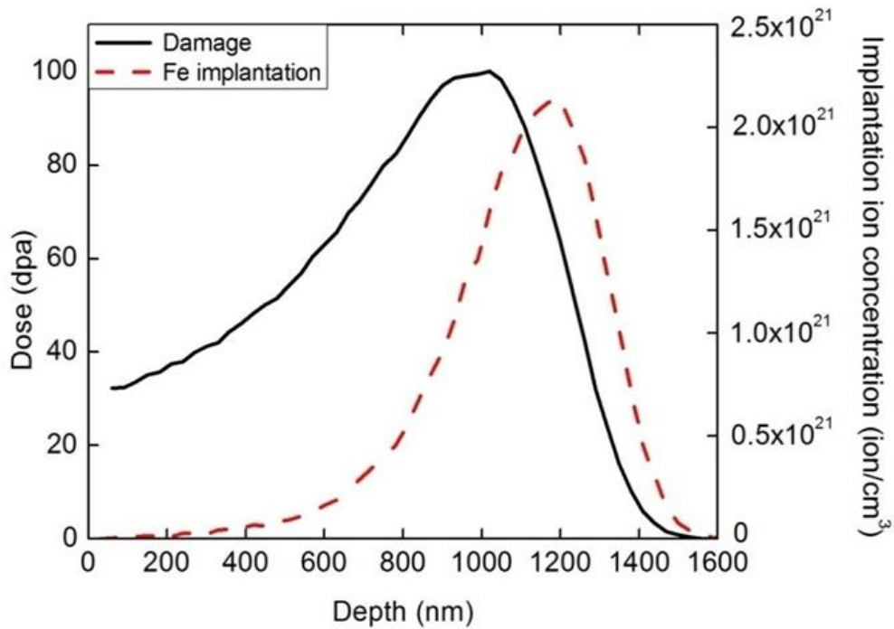
Figure 2.1 SRIM-calculated depth profiles of dpa and implanted atoms in pure Fe irradiated with 3.5 MeV \text{Fe}^{2+} ions for 100 peak dpa.
