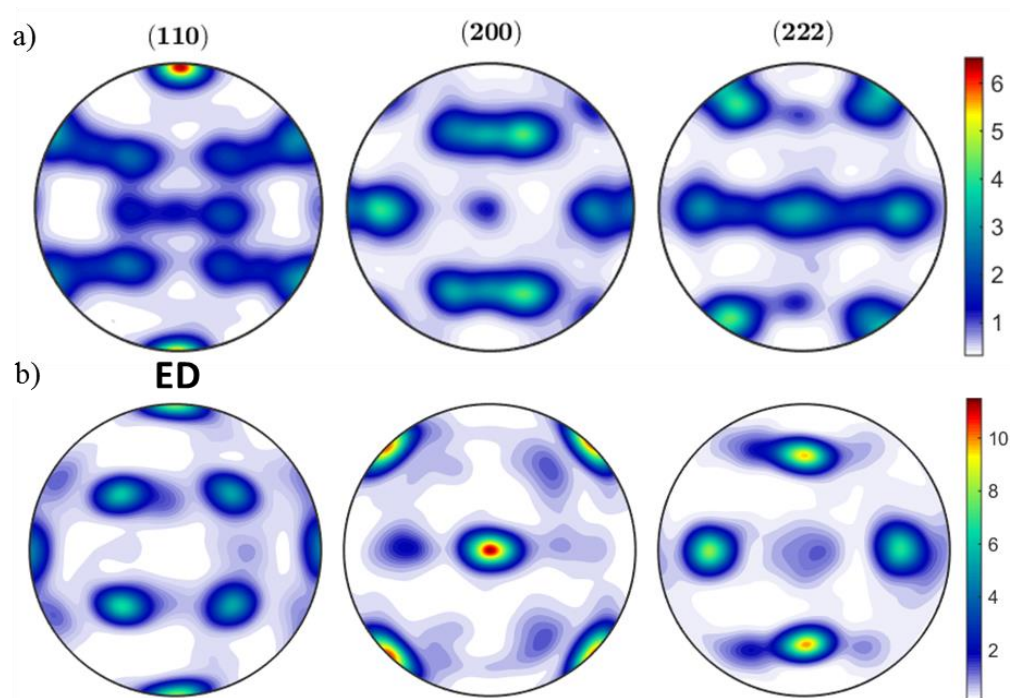
Figure 6.13 Pole figures of 14YWT final tube after hydrostatic extrusion obtained by (a) Neutron diffraction, and (b) EBSD techniques.
