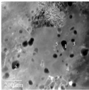
Figure 7.9 Composition analysis of polygonal shaped dark particles having a size ranging between 10-250 nm in Process II tube.
