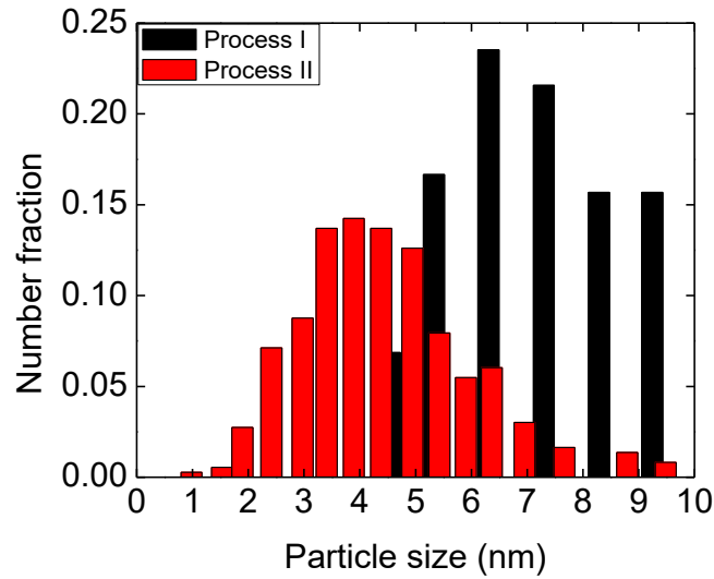
Figure 7.12 NF size (<10 nm) distribution of (a) Process I and (b) Process II alloys.
