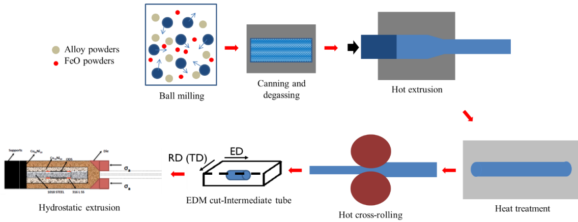
Figure 6.2 Processing steps of Process II (RD: rolling direction, TD: transverse direction, ED: extrusion direction)
