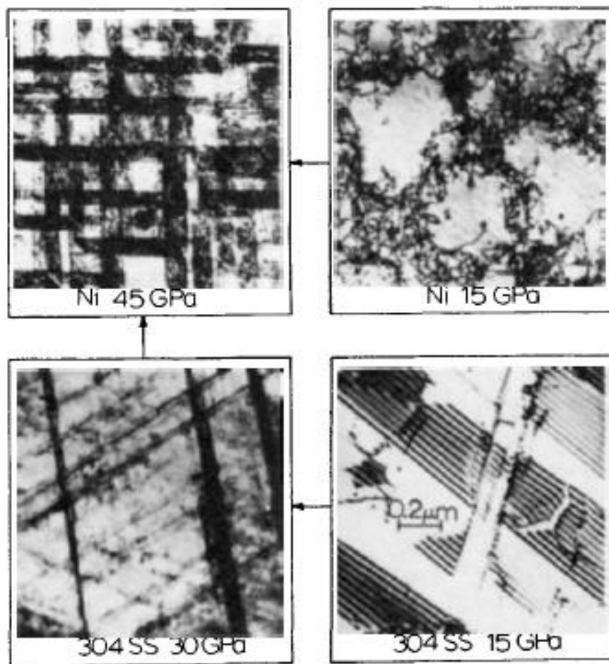
Figure 1.20 Micrographs showing the evolution of microstructure with increasing shock loading pressures in Nickel and 304 stainless steel [95].
