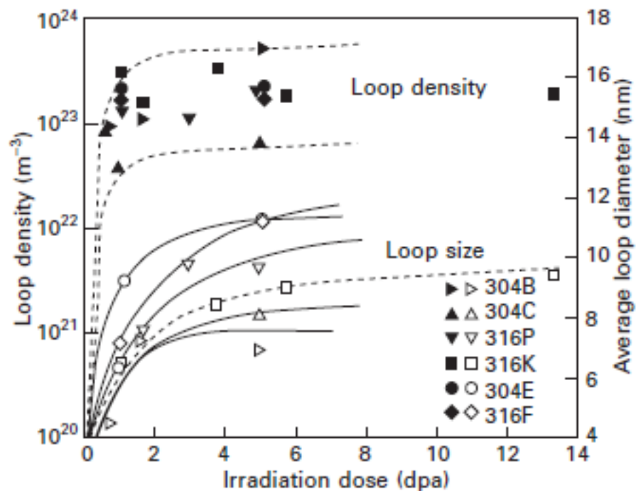
Figure 1.6 Dislocation loop size and density with increasing irradiation dose up to 13 dpa at 300 °C in various austenitic steels [25].
