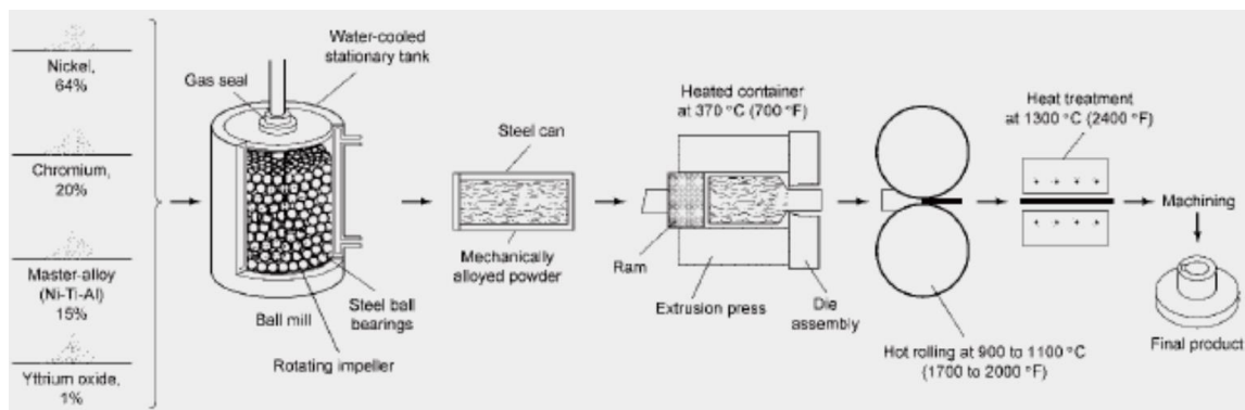
Figure 1.17 Typical mechanical alloying process for the production of ODS alloys [72].
