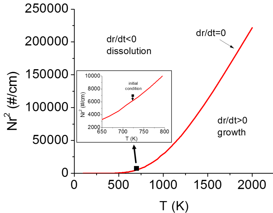
Figure 8.14 Nr^2 vs. T plot showing the behaviour of the dispersoids in the present study.
