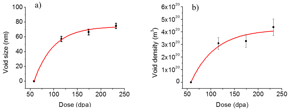
Figure 3.4 Plots of (a) void size and (b) void density as a function of local dpa for annealed EK-181. Measurements were performed at the depth region between 400 to 700 nm.
