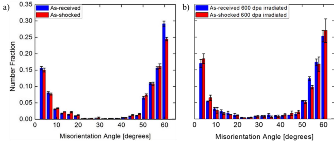
Figure 5.2 Misorientation angle distribution of as-received and as-shocked samples (a) before irradiation (b) after 600 dpa irradiation.
