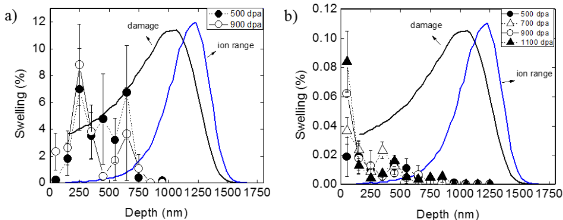
Figure 7.16 Swelling vs. depth profiles of the (a) Process I tube after 500 and 900 dpa (b) Process II tube after 500, 700, 900 and 1100 dpa irradiations with \text{Fe}^{2+} at 450 °C. Note the difference in the scale of swelling (%).
