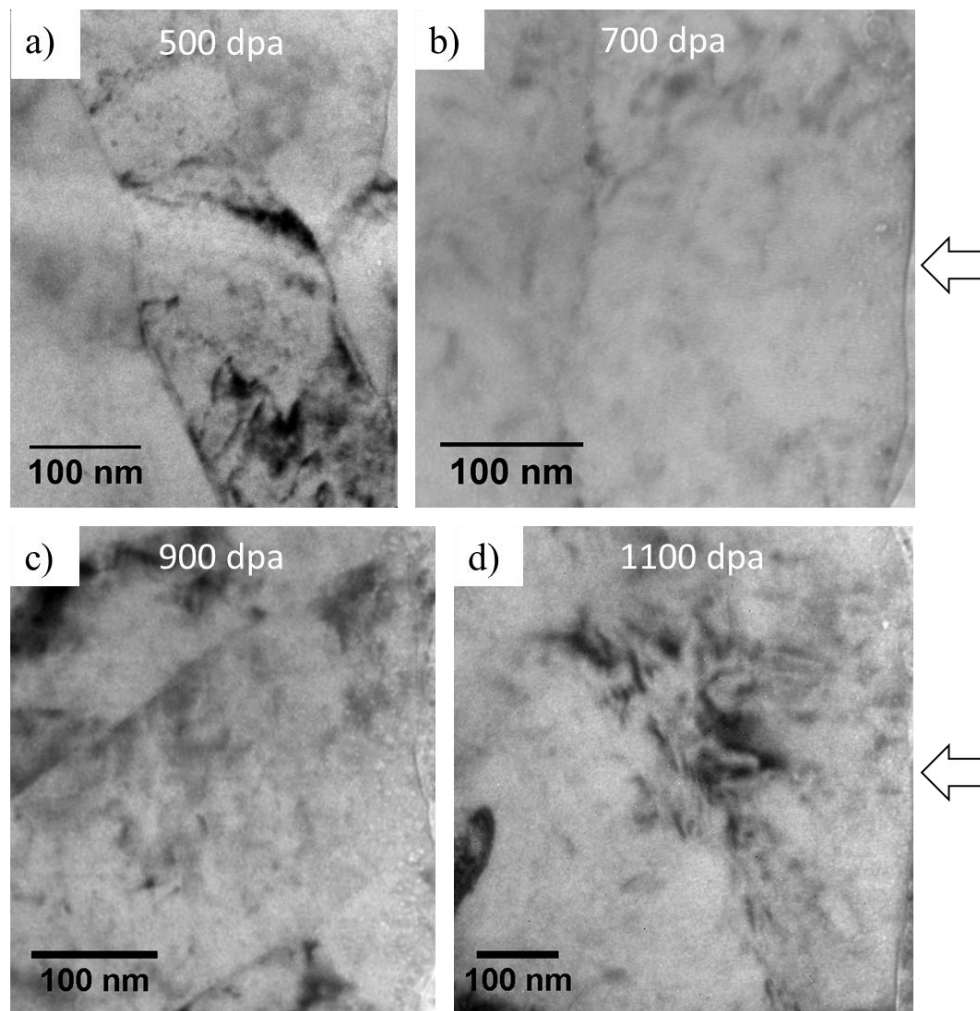
Figure 7.15 BFTEM images of Process II tube after (a) 500 dpa (b) 700 dpa (c) 900 dpa and (d) 1100 dpa irradiations. Arrows indicate the direction of ion beam. Images were taken at \sim 3 \mu\text{m} under focus condition.
