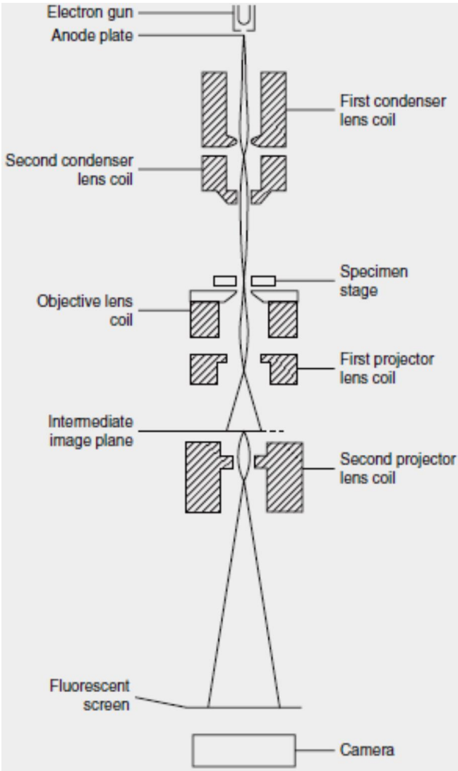
Figure 2.3 Schematic illustration of optics of transmission electron microscopy [107].
