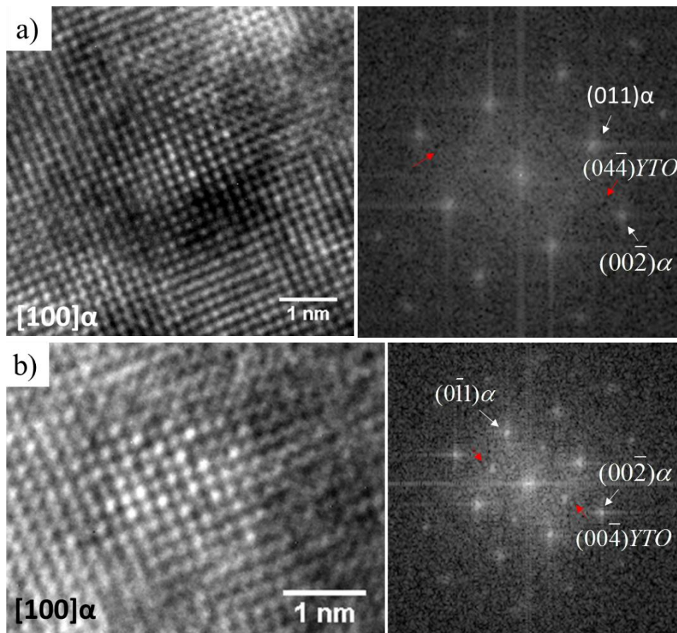
Figure 8.4 HRTEM micrographs and their corresponding FFTs along [100]_{\alpha} in particles having the OR of (a) (00\bar{2})_{\alpha} \parallel (04\bar{4})_{Y_2Ti_2O_7} and (b) (00\bar{2})_{\alpha} \parallel (00\bar{4})_{Y_2Ti_2O_7} .
