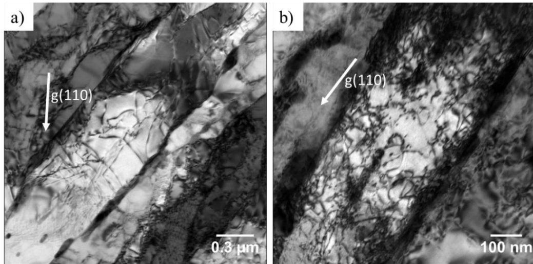
Figure 4.2 TEM bright field images of (a) as-received (b) as-shocked conditions along (110) direction showing the structure of dislocations.
