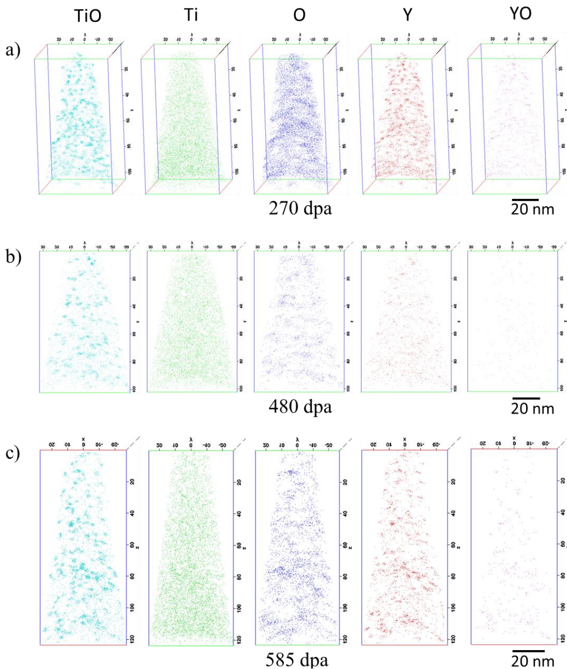
Figure 8.12 APT 3D reconstructions showing the distribution of various elements and ions in 14YWT samples irradiated to (a) 270 dpa (b) 480 dpa and (c) 585 dpa at 450 °C.
