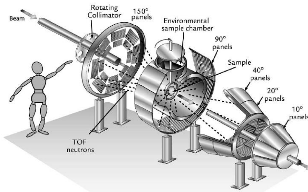
Figure 2.2 Schematic view of the HIPPO diffractometer showing the structure of the instrument and arrangement of detectors panels. A person is used for a scale. The distance between 10° and 150° panel is 3 m [104].
