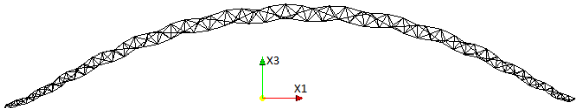
Figure 5.11: Arc shape produced in the tetrahedral beam like truss
