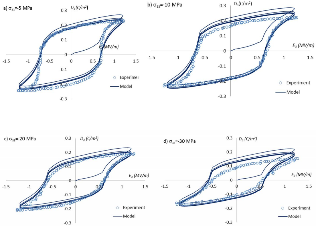
Figure 2.5: Hysteresis polarization responses under constant compressive stresses
