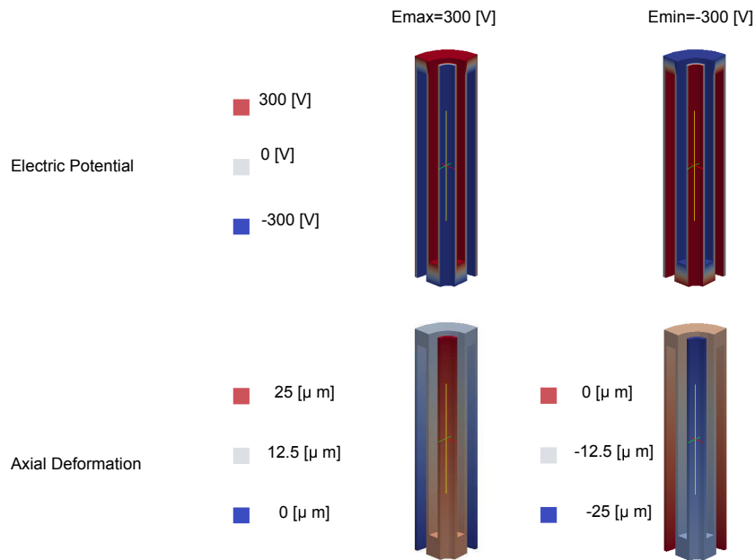
Figure 3.10: Electric potential and deflection contour of PZT-586 telescopic actuator
