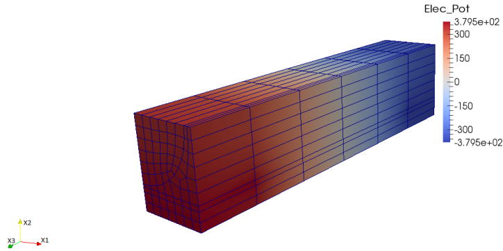
Figure 4.10: Distribution of electric potential in its unit cell of AFC (Electrode Voltage is 380V)
