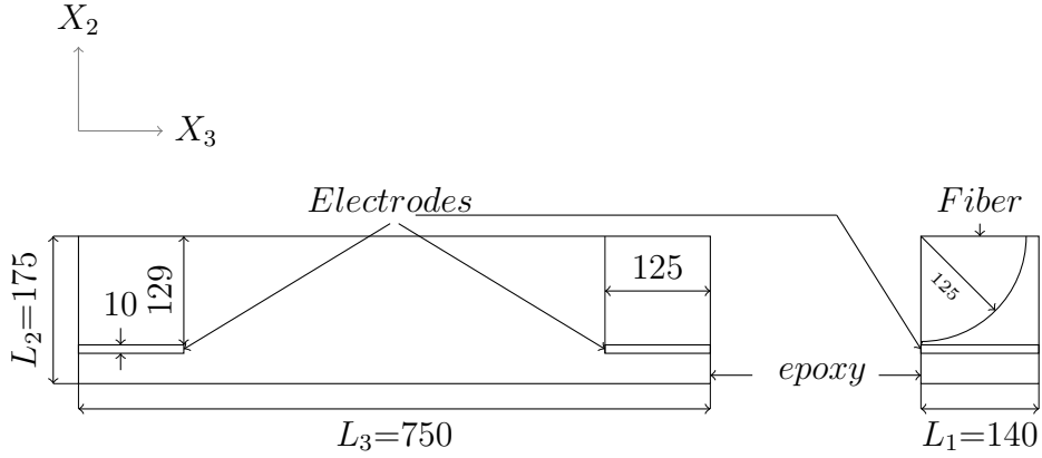
Figure 4.9: Geometry of AFC unit cell (dimensions are in \mu m )
