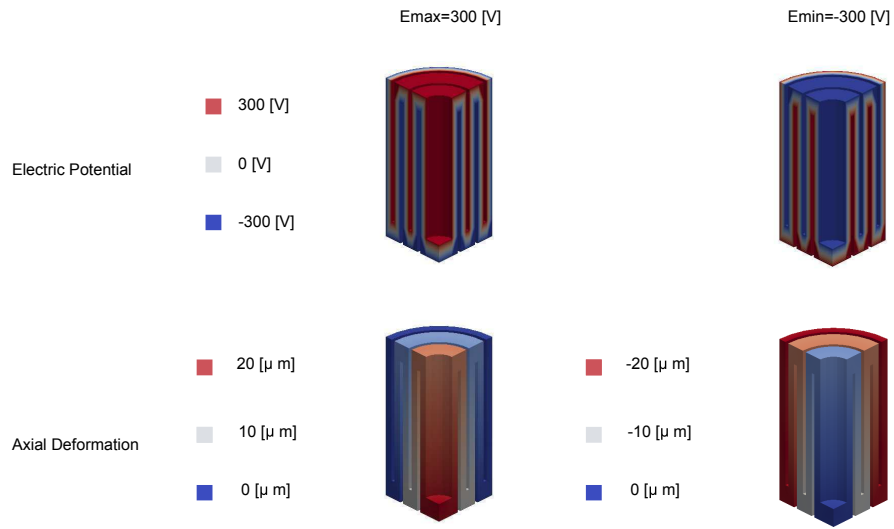
Figure 3.13: Electric potential and deflection contour of MSI-53 Telescopic Actuator
