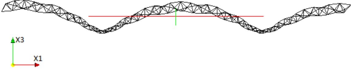
Figure 5.12: Cyclic shape produced in the tetrahedral beam like truss
