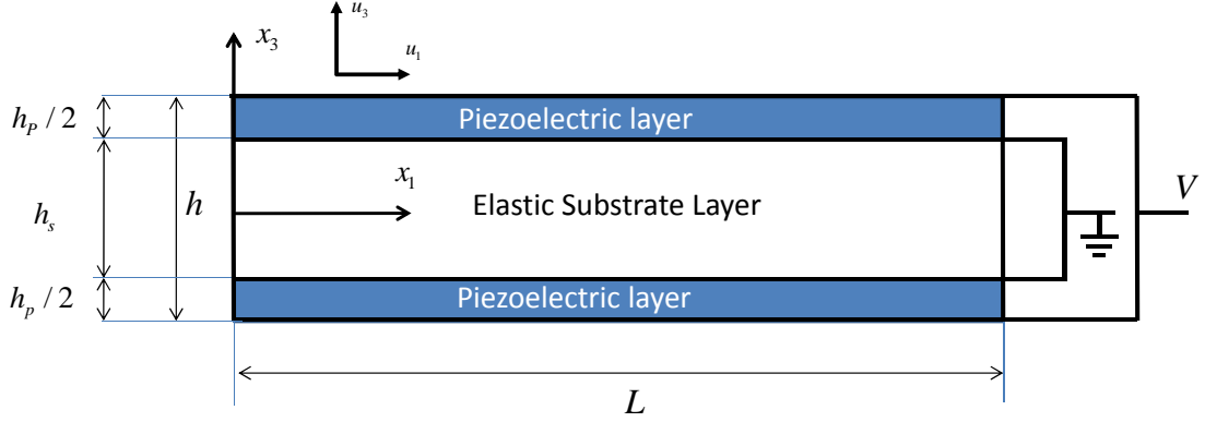
Figure 4.1: Substrated bimorph beam geometry
