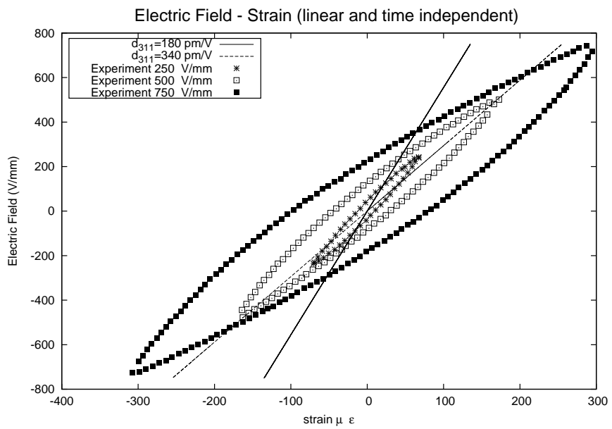
Figure 3.4: Linear time independent model compared with experimental strain ( \varepsilon_{11} ) response under electric field ( E_3 ) with frequency 0.1 Hz in [19]
