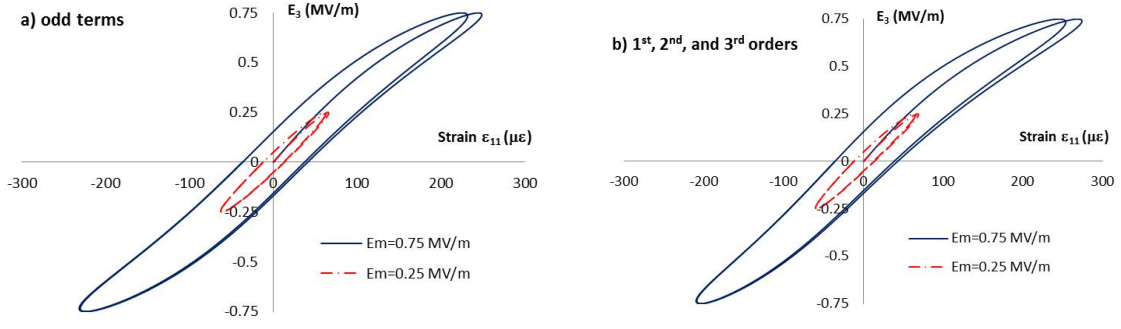
Figure 3.2: The effect of the higher order terms on the hysteretic response ( f=0.1 Hz)
