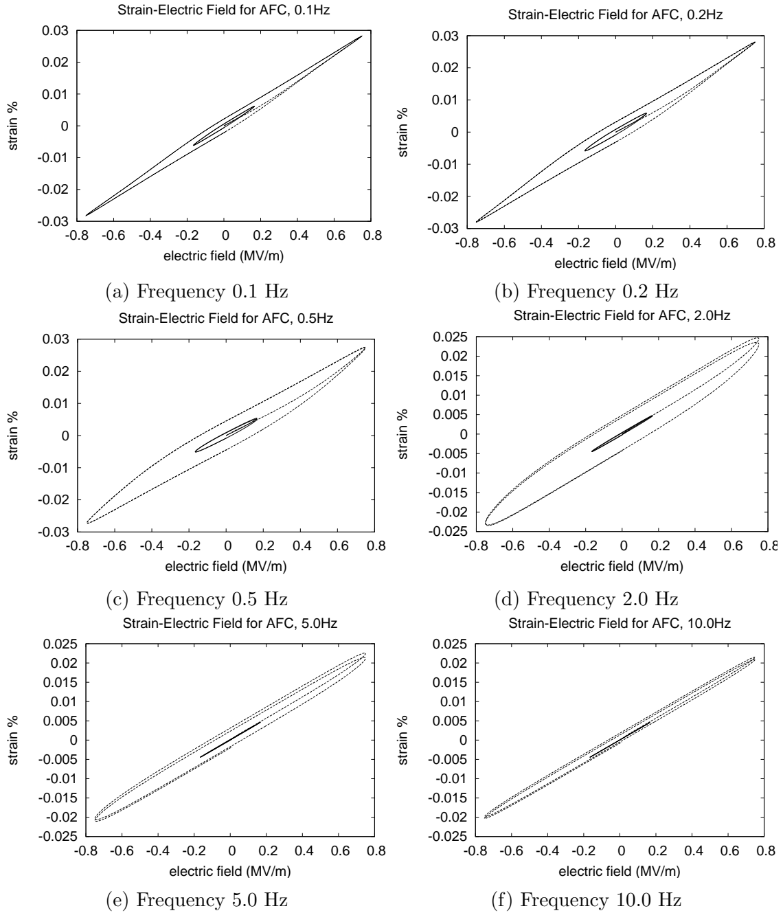
Figure 4.15: Effect of frequency of applied electric field on strain response of AFC
