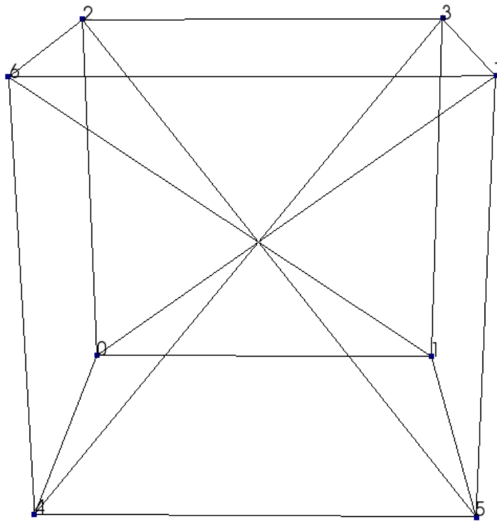
Figure 5.1: One element of space filler truss
