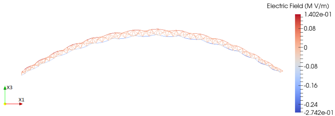
Figure 5.16: The electric field distribution in a beam like tetrahedral truss in the arc configuration
