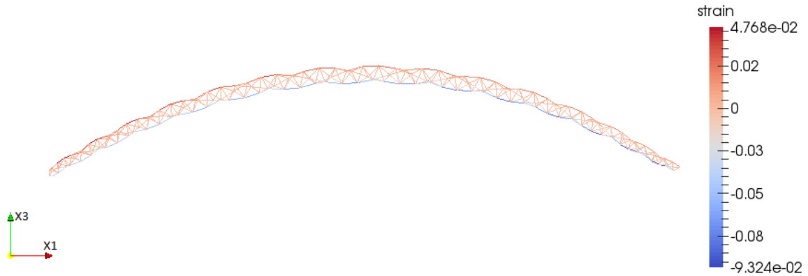
Figure 5.15: The strain distribution in a beam like tetrahedral truss in the arc configuration
