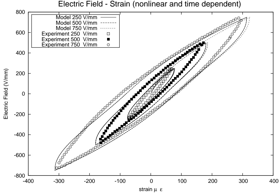
Figure 3.6: Nonlinear time dependent strain ( \varepsilon_{11} ) response under electric field ( E_3 ) with frequency 0.1 Hz compared with experiment [19].
