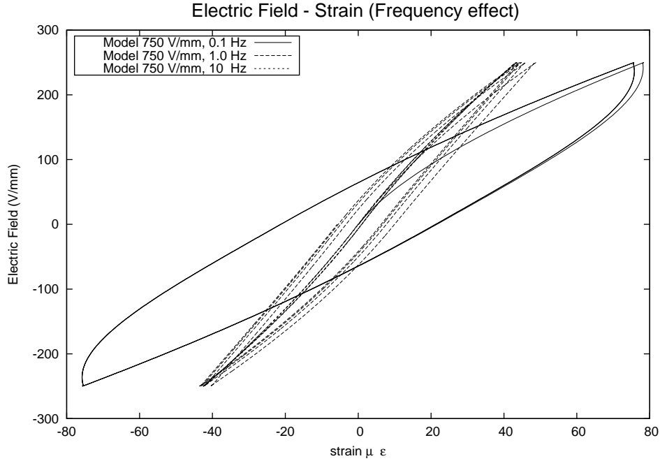
Figure 3.8: Effect of frequency of applied electric field ( E_3 ) on strain ( \varepsilon_{11} ) response
