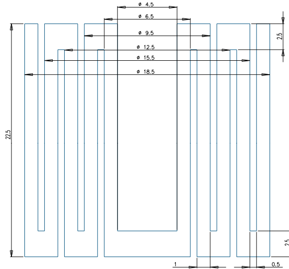
Figure 3.12: Geometry of MSI-53 (dimensions are in mm)
