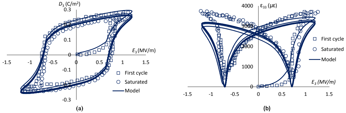
Figure 2.3: Hysteresis polarization and butterfly strain responses for PZT51 at zero stress
