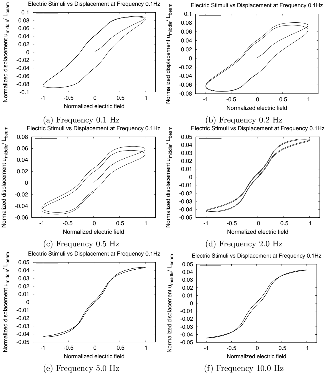
Figure 5.24: Effect of frequency of applied electric field on strain response of tetrahedral truss
