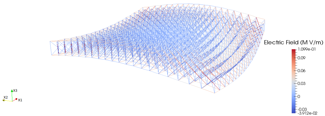
Figure 5.7: The electric field contour of planar space filler truss for the X_3 = X_1^2 - X_2^2 shape (displacement are scaled 20 times)
