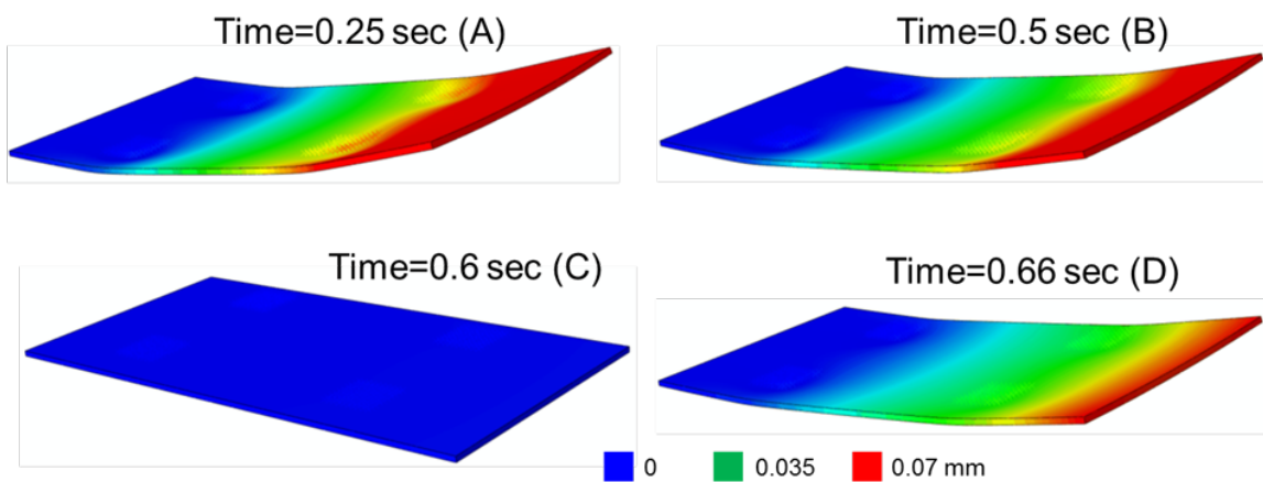
Figure 2.11: The corresponding deformed shape of an active cantilever plate due to a uniform cyclic electric field applied to the piezoelectric patches
