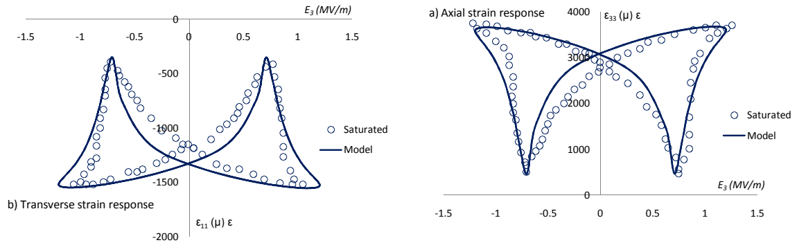
Figure 2.4: Saturated strain responses for PZT51 at zero stress
