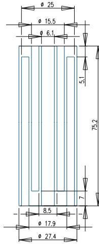
Figure 3.9: Geometry of PZT-586 telescopic actuator (dimensions are in mm)
