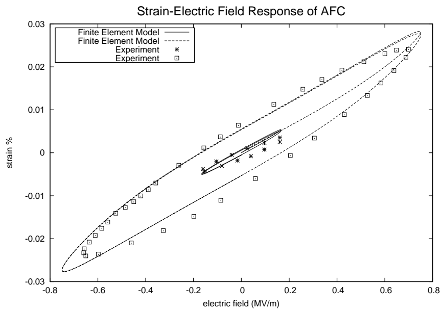
Figure 4.14: Linear electro-mechanical hysteresis response of AFC model with time shift for different electric fields at 1Hz compared with experiment
