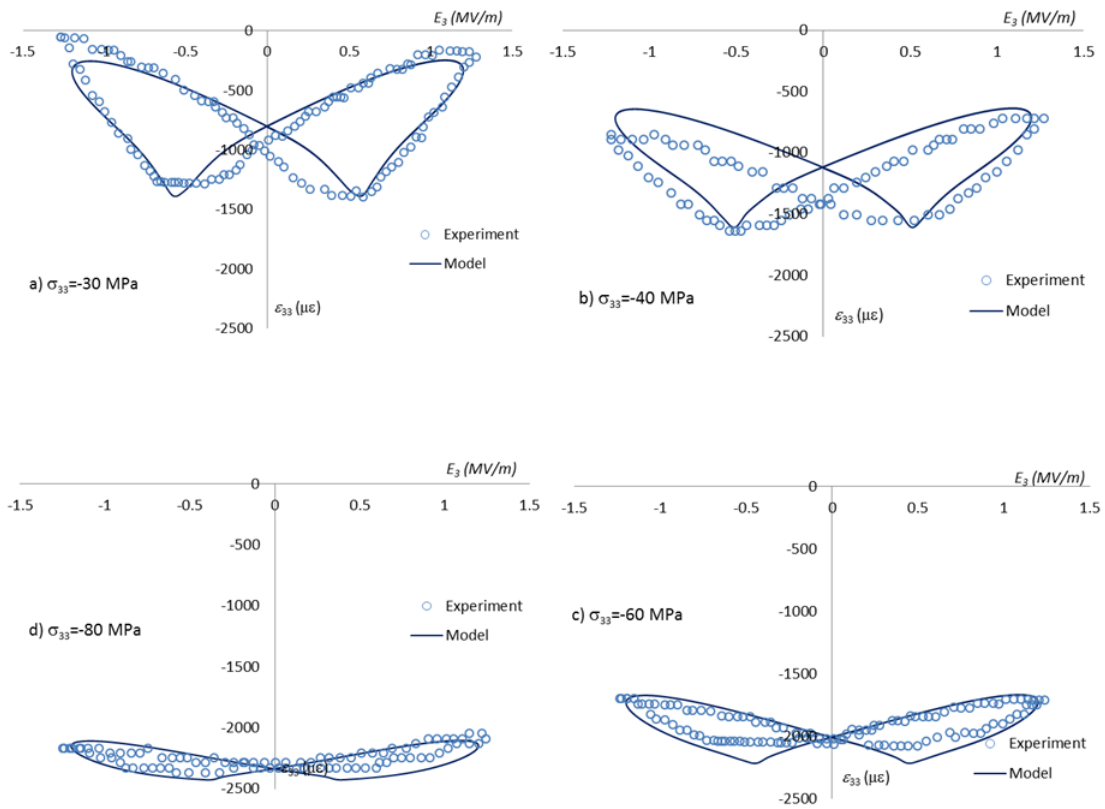
Figure 2.8: Butterfly strain responses under constant compressive stresses above the coercive stress
