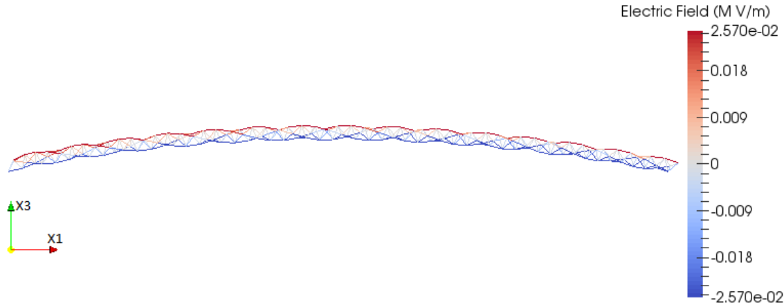
Figure 5.22: The electric field distribution in a beam like tetrahedral truss in the arc configuration with limiting strain 1%
