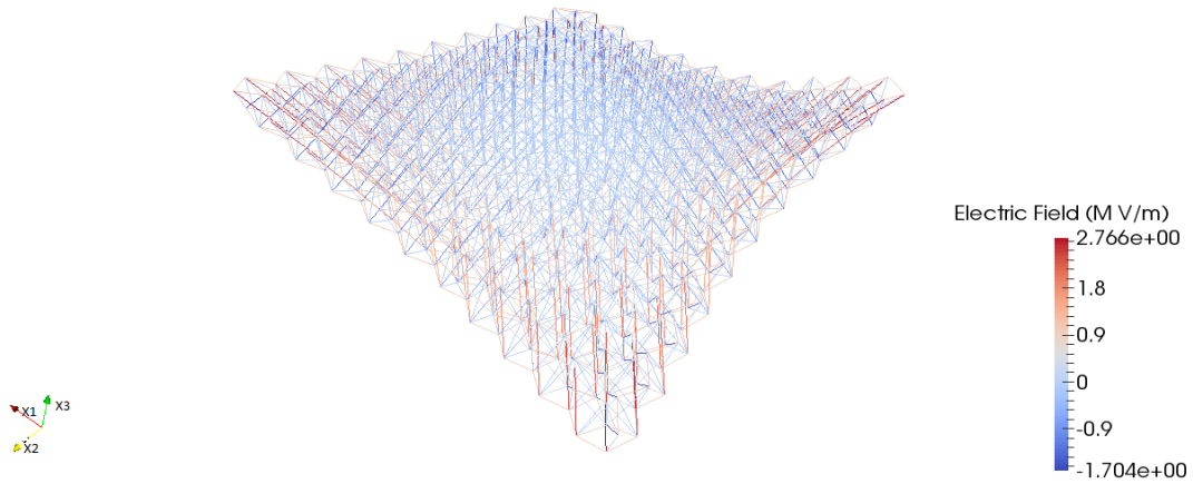
Figure 5.5: The deformed configuration for the planar truss under electric field
