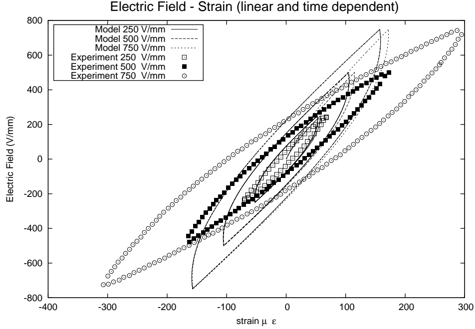
Figure 3.5: Linear and history dependent model compared with experimental strain ( \varepsilon_{11} ) response under electric field ( E_3 ) with frequency 0.1 Hz in [19]
