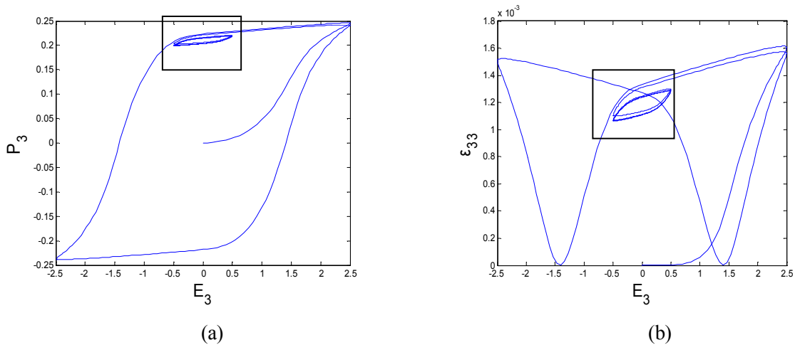
Figure 2.2: Minor hysteresis loops in a polarized piezoelectric sample: a) polarization response and b) corresponding strain response
