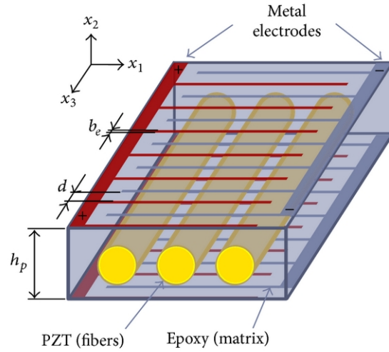
Figure 4.8: Schematic for placement of fibers and electrodes in the epoxy matrix* [33]
