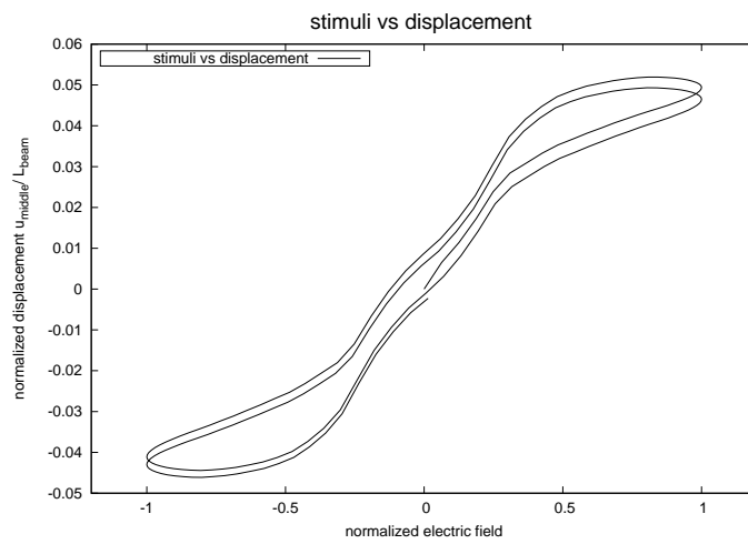
Figure 5.23: Nonlinear and time dependent response for deflection of beam like truss under frequency 1Hz with limiting strain
