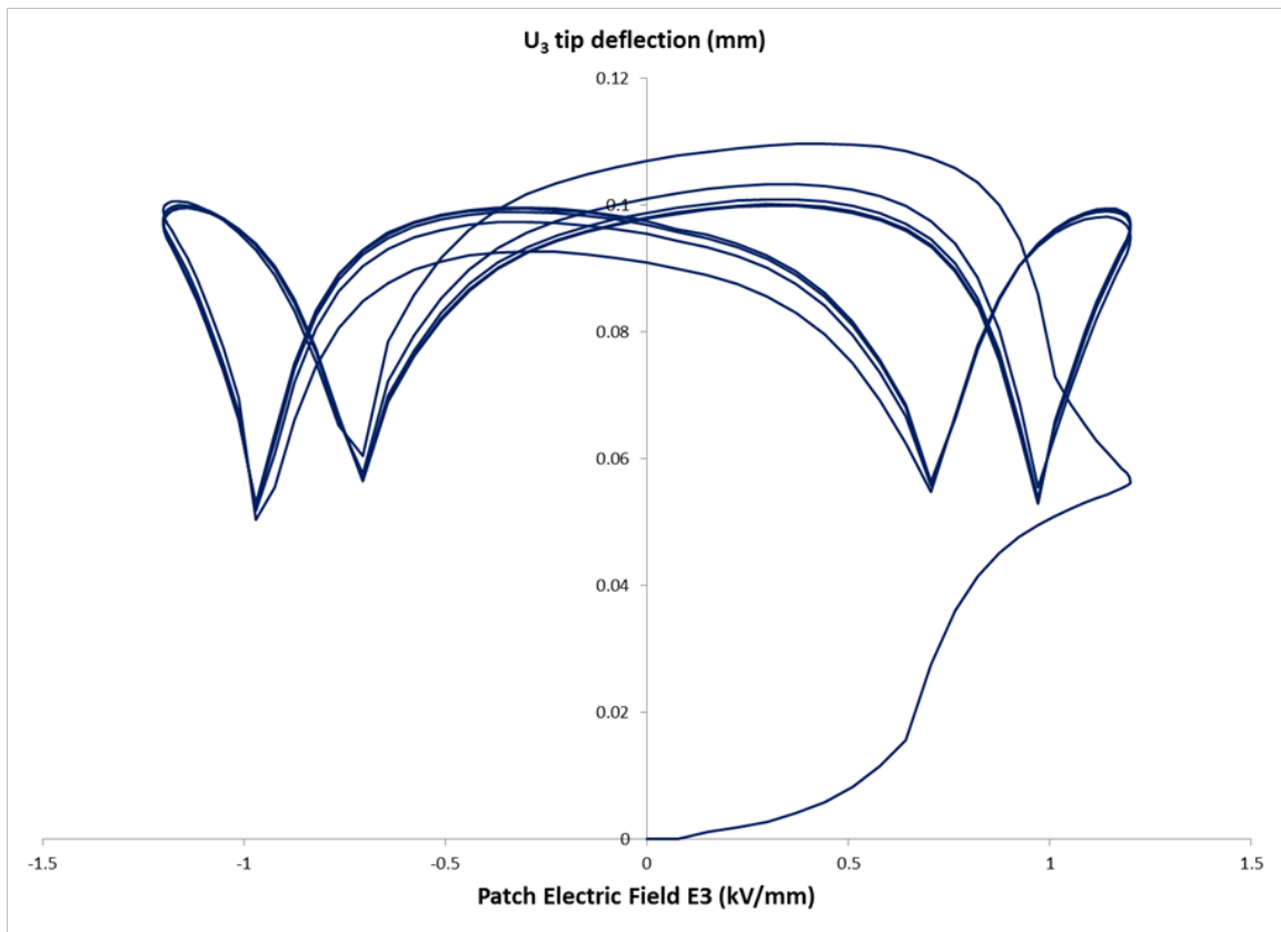
Figure 2.12: Tip deflection of the twisting cantilever plate due to a non-uniform cyclic electric field applied to the piezoelectric patches
