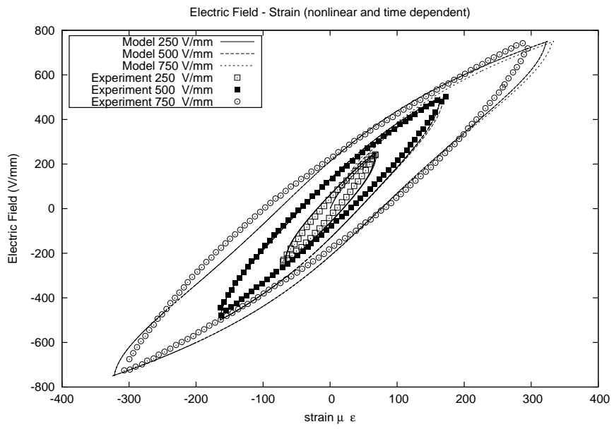
Figure 3.7: Nonlinear time dependent strain ( \varepsilon_{11} ) response under electric field ( E_3 ) with frequency 0.1 Hz for third order model compared with experiment [19]
