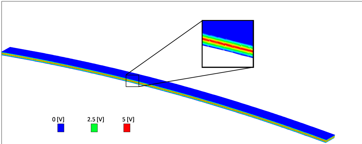
Figure 4.3: Bimorph PVDF beam electric potential distribution
