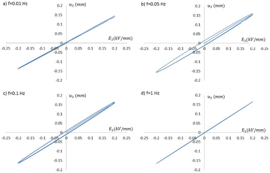
Figure 4.6: Tip deflection of bimorph beam, comparing observing effect of frequency of applied electric field
