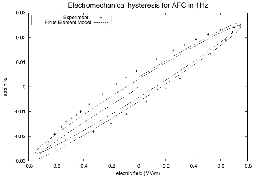
Figure 4.11: Electro-mechanical hysteresis at 1Hz compared with experiment
