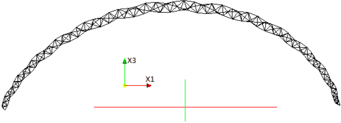
Figure 5.13: Shape produced in the tetrahedral beam like truss including the all normal strains
