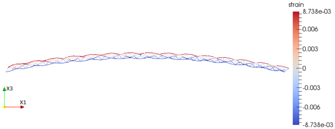
Figure 5.21: The strain distribution in a beam like tetrahedral truss in the arc configuration with limiting strain 1%
