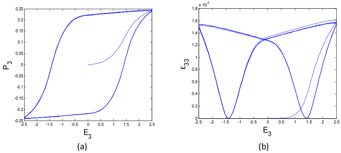
Figure 2.1: Major hysteresis loops in a piezoelectric sample: a) polarization response and b) corresponding strain response
