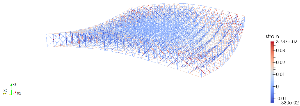
Figure 5.6: The strain contour of planar space filler truss for the X_3 = X_1^2 - X_2^2 shape (displacement are scaled 20 times)
