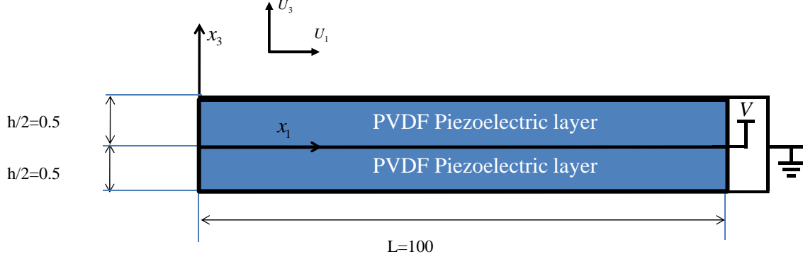
Figure 4.2: Bimorph PVDF beam geometry and placement of electrodes
