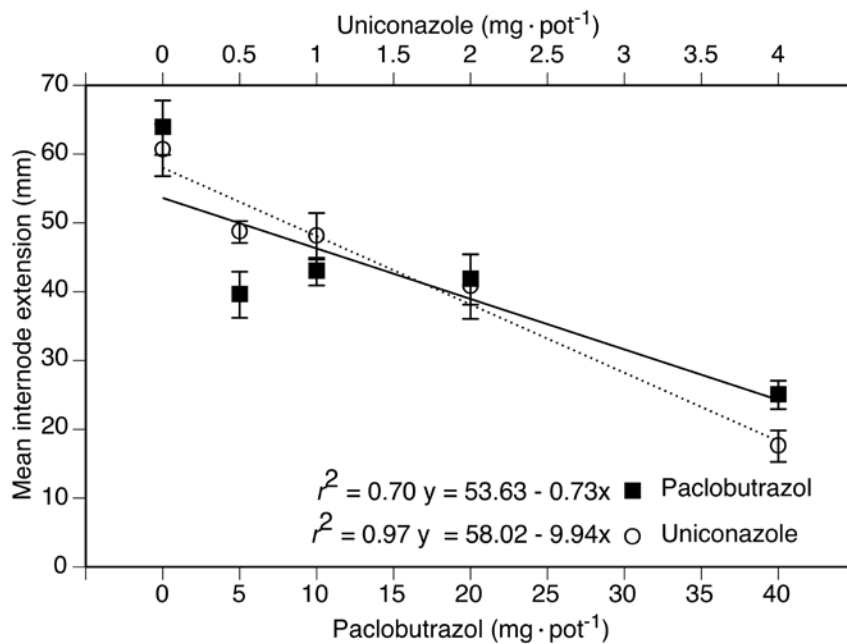
Fig. 3.15. Sesuvium portulacastrum internode extension in response to drench applied paclobutrazol or uniconazole. Main effects of drench applied paclobutrazol or drench applied uniconazole on mean internode extension ( n = 5 ) of Sesuvium portulacastrum . All regression equations were based on means. Solid lines indicate paclobutrazol treated plants and dashed lines indicate uniconazole treated plants.
