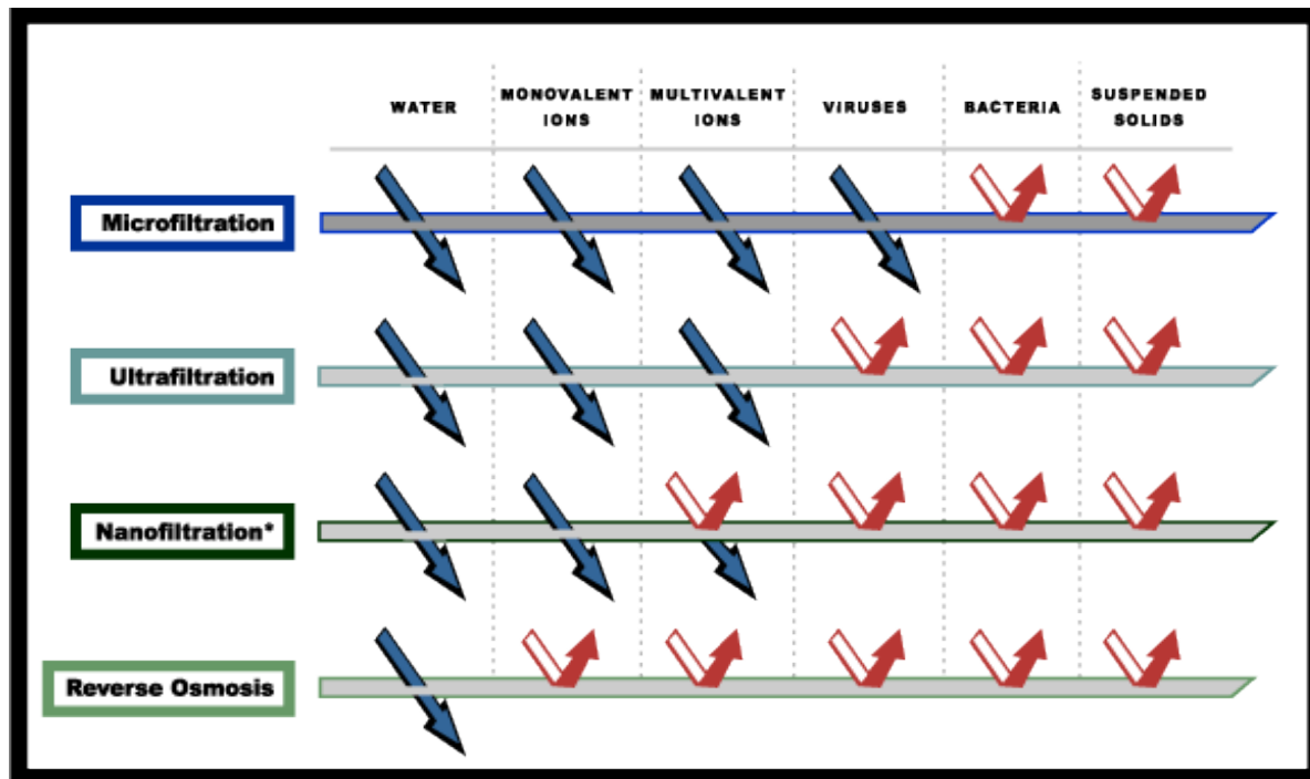
Figure 2-4. Different Levels of Membrane Filtration in Water Purification
