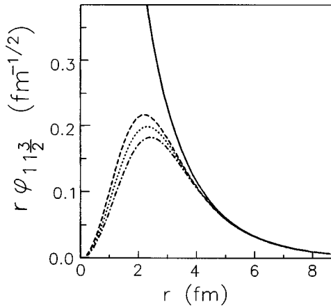
FIG. 10. The radial behavior of the single particle radial bound state proton wave functions r\varphi_{n_X l_X j_X}(r) , n_X=1, l_X=1, j_X=3/2 , in {}^{10}\text{B} calculated in the Woods-Saxon potentials with a=0.60 fm and r_0=1.00 fm, dashed line; r_0=1.25 fm, dotted line; r_0=1.50 fm, dashed-dotted line. The Coulomb radius r_C=1.20 fm. The solid line is the tail bW_{-\eta_X, 3/2}(2\kappa_Y a r) of the bound state wave function r\varphi_{n_X l_X j_X}(r) for r_0=1.00 fm, a=0.60 fm, with b=2.78 fm ^{-1/2} . The other two bound state wave functions are also normalized to that tail.
