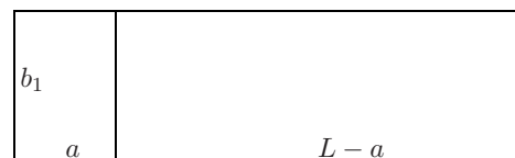
FIG. 1. A rectangular piston in two dimensions (see Ref. [3]). In three dimensions there is another length b_2 perpendicular to the plane of the figure.
