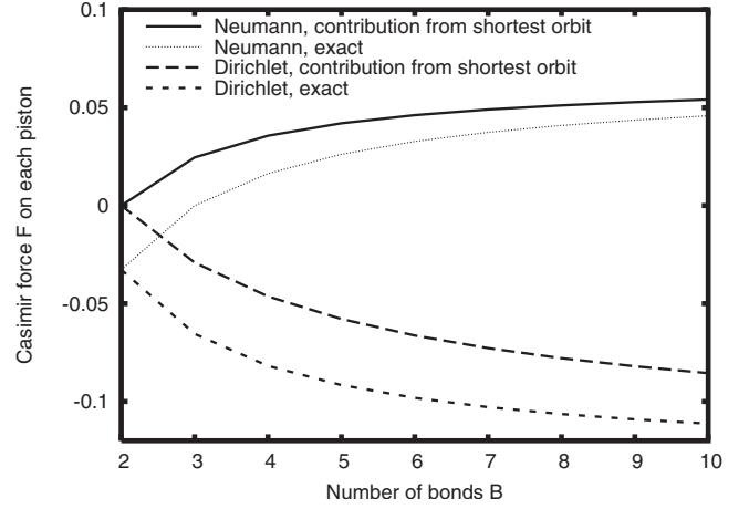
FIG. 3. The force on a piston in a star graph with B bonds of length 1, Kirchhoff boundary condition at the center, and either Neumann or Dirichlet boundary condition at each piston is computed using only the shortest periodic orbit [Eq. (24)] and compared with the exact answer. Positive values indicate repulsive forces. All quantities plotted in this and subsequent figures are dimensionless.
