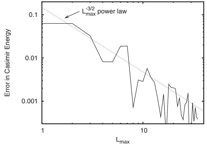
FIG. 5. The error |E_c^{L_{\max}} - E_c| is shown for the same quantum graph as in Fig. 4, but with a Dirichlet piston at the end of the first bond.
