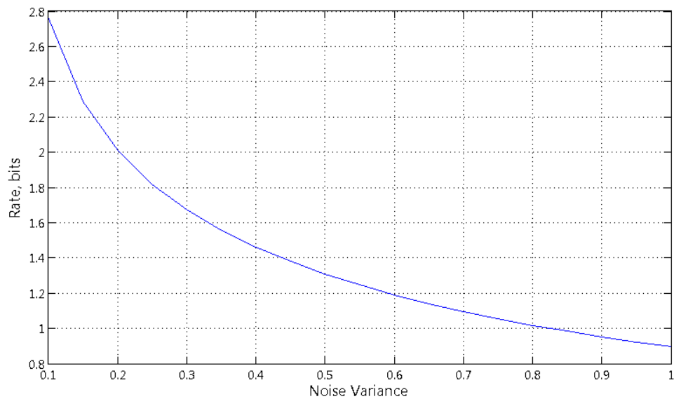
Fig. 18. Rate vs. noise variance for a Gaussian mixture signal with the relay at d=0.95 .
