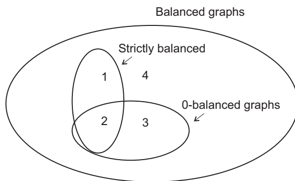
Fig. 5. Relationships between various notions of balanced graphs
