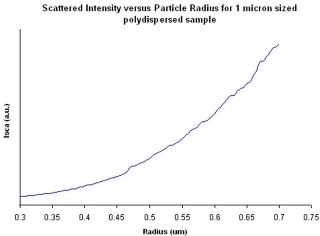
Figure 11 Scattered intensity in arbitrary units (a.u.) versus microsphere size of 1 \mu\text{m} polydispersed PS sample when excited by evanescent waves.
