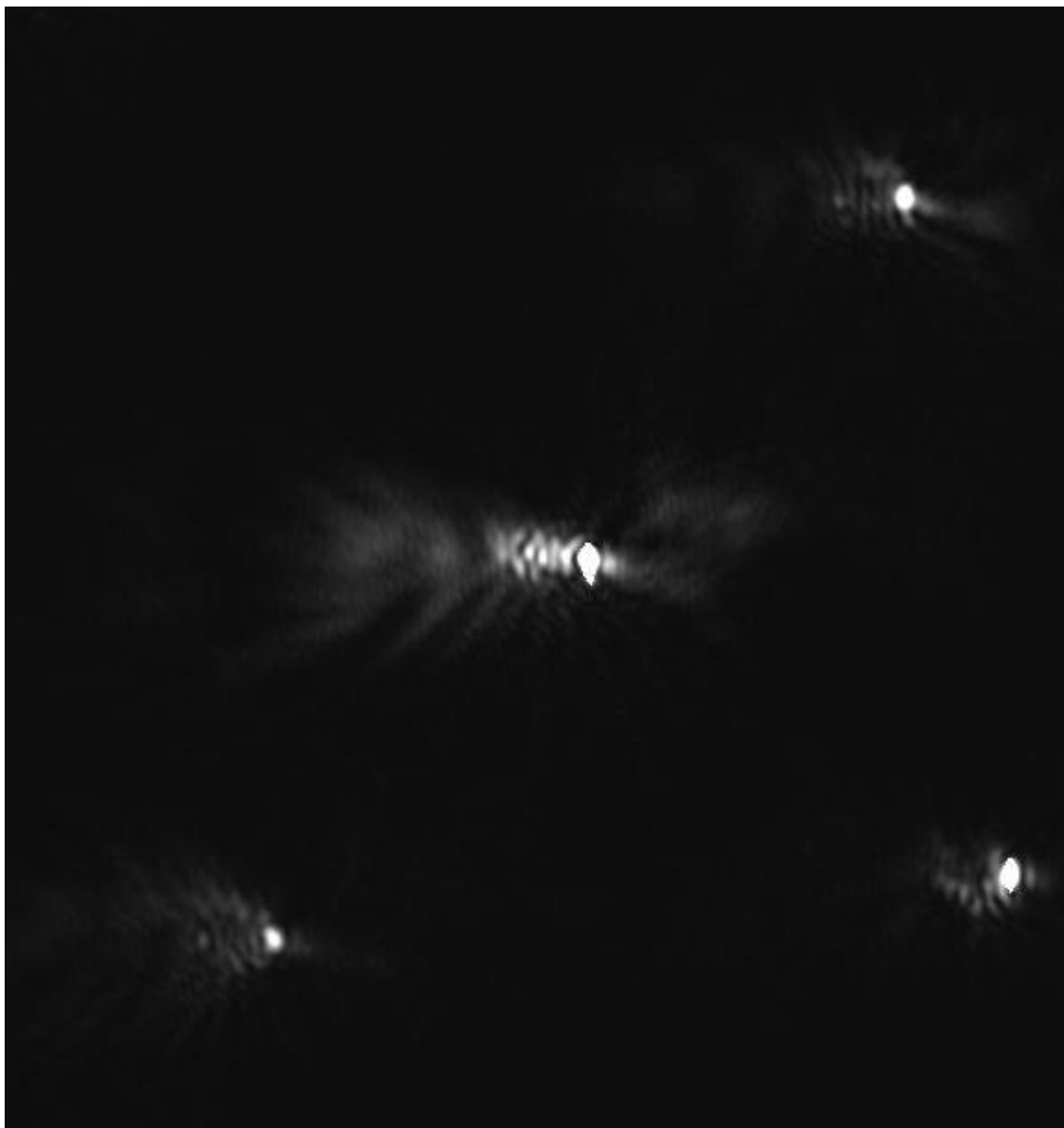
Figure 17 Scattering from approximately 6 micron polystyrene microspheres in air without any background light.
