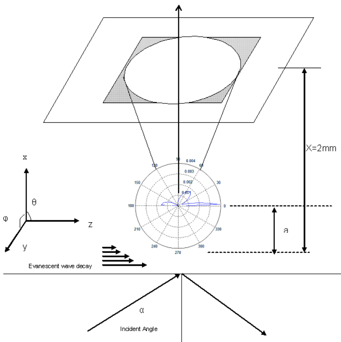
Figure 6 Model configuration for theoretical calculations showing the axis. Here evanescent waves travel along Z axis, the size of the microsphere chosen for the polar plot is 4\ \mu\text{m} diameters PS. The light is scattered more in the forward direction and hence higher values of scattered intensity at around 0^\circ . A weak lobe also occurs at the end near 180^\circ , which can be mainly attributed to backward scattering.
