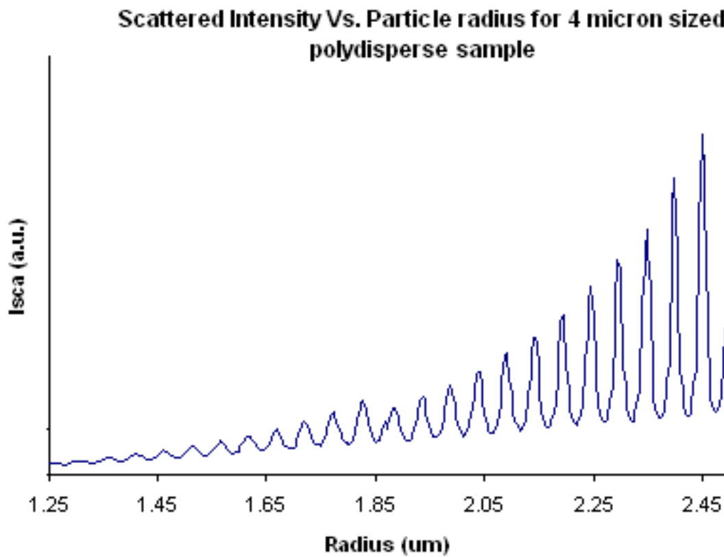
Figure 13 Scattered intensity in arbitrary units (a.u.) versus microsphere size of 4 \mu\text{m} polydispersed PS sample when excited by evanescent waves.
