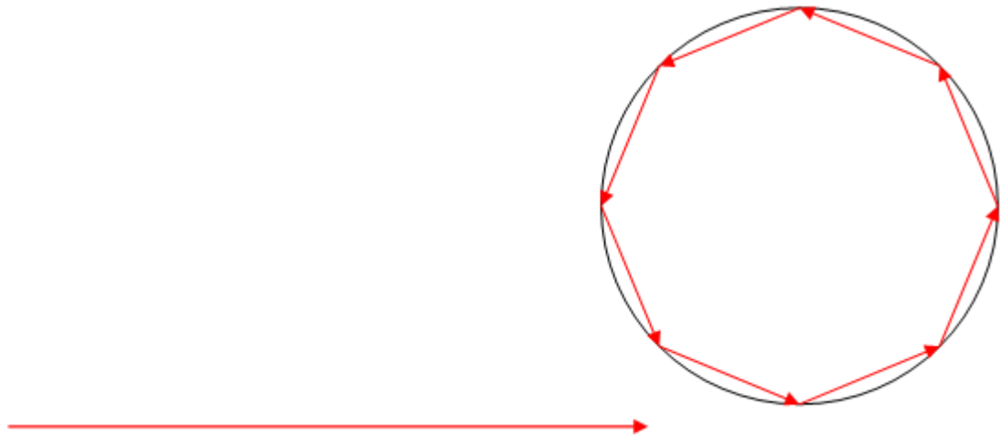
Figure 4 Whispering Gallery Modes (WGM) resonances occur due to TIR on the inner surface of the microsphere. They are efficiently excited with evanescent light due to the high angle of incidence near the bottom of the microsphere.
