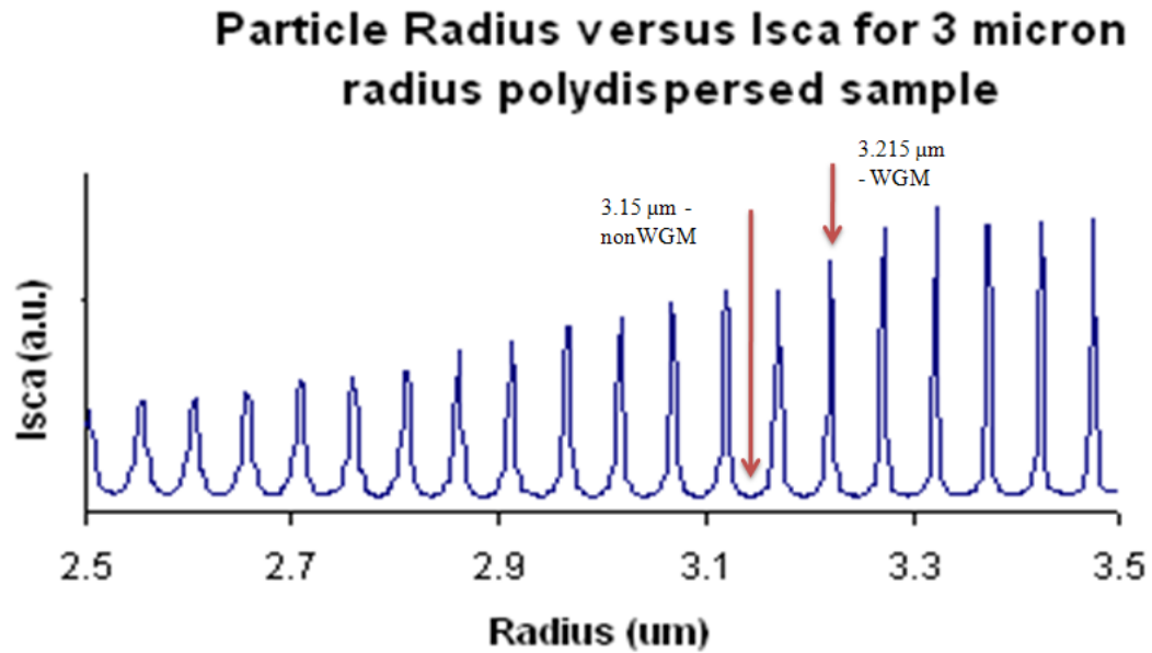
Figure 15 Theoretical calculation results for the microsphere size vs. scattered intensity for polydispersed PS microspheres in air with mean diameter of 6 \mu\text{m} .
