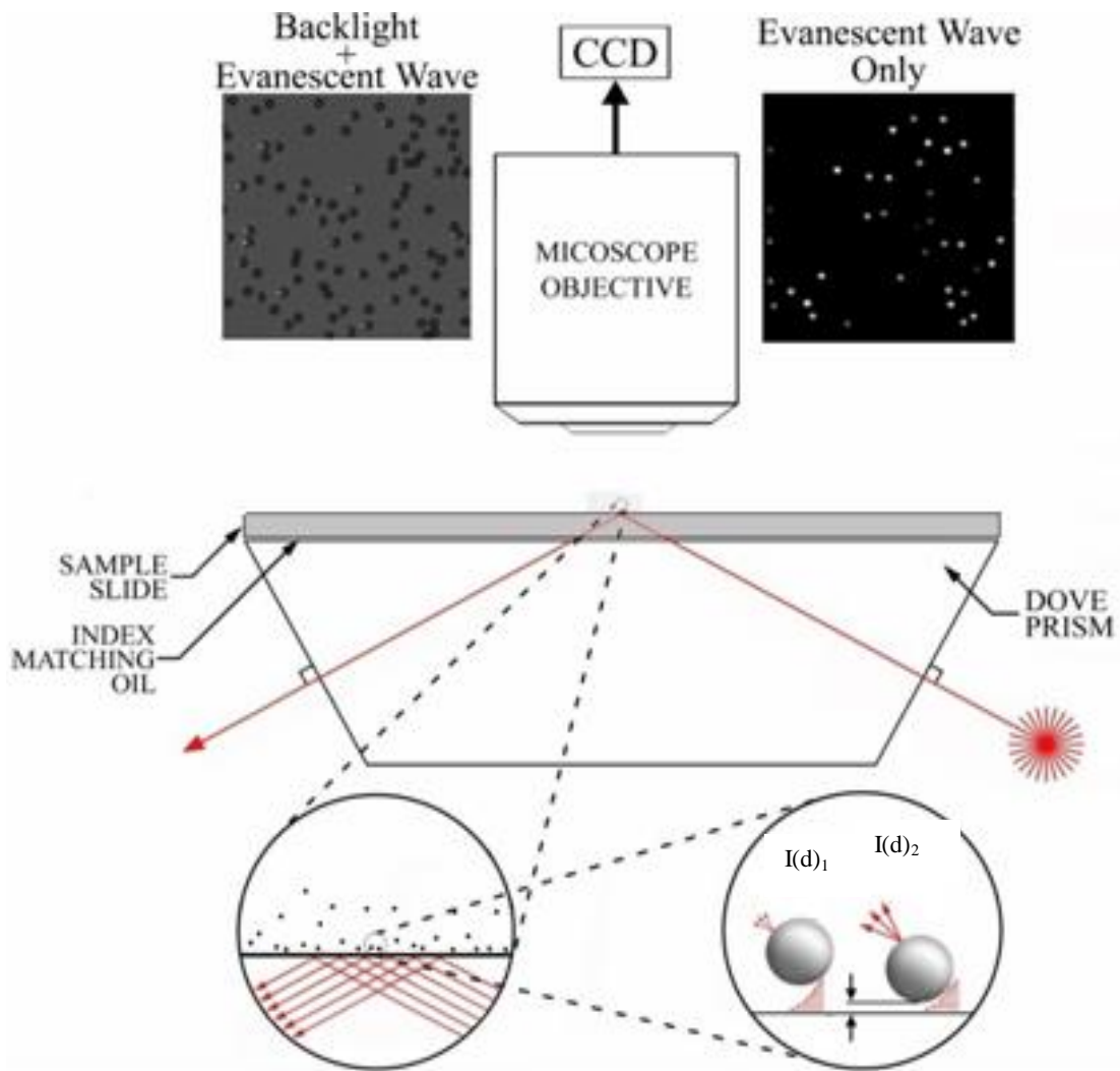
Figure 3 DCPM system for multiple particles. The laser light is incident on the prism from the right, the evanescent waves are generated above the slide and the microsphere sample on the slide is illuminated by these waves. The inset shows the microspheres of different sizes located at different distances above the slide. The images shown in above the setup is the different patterns of the microsphere scattering, the images are captured by CCD.
