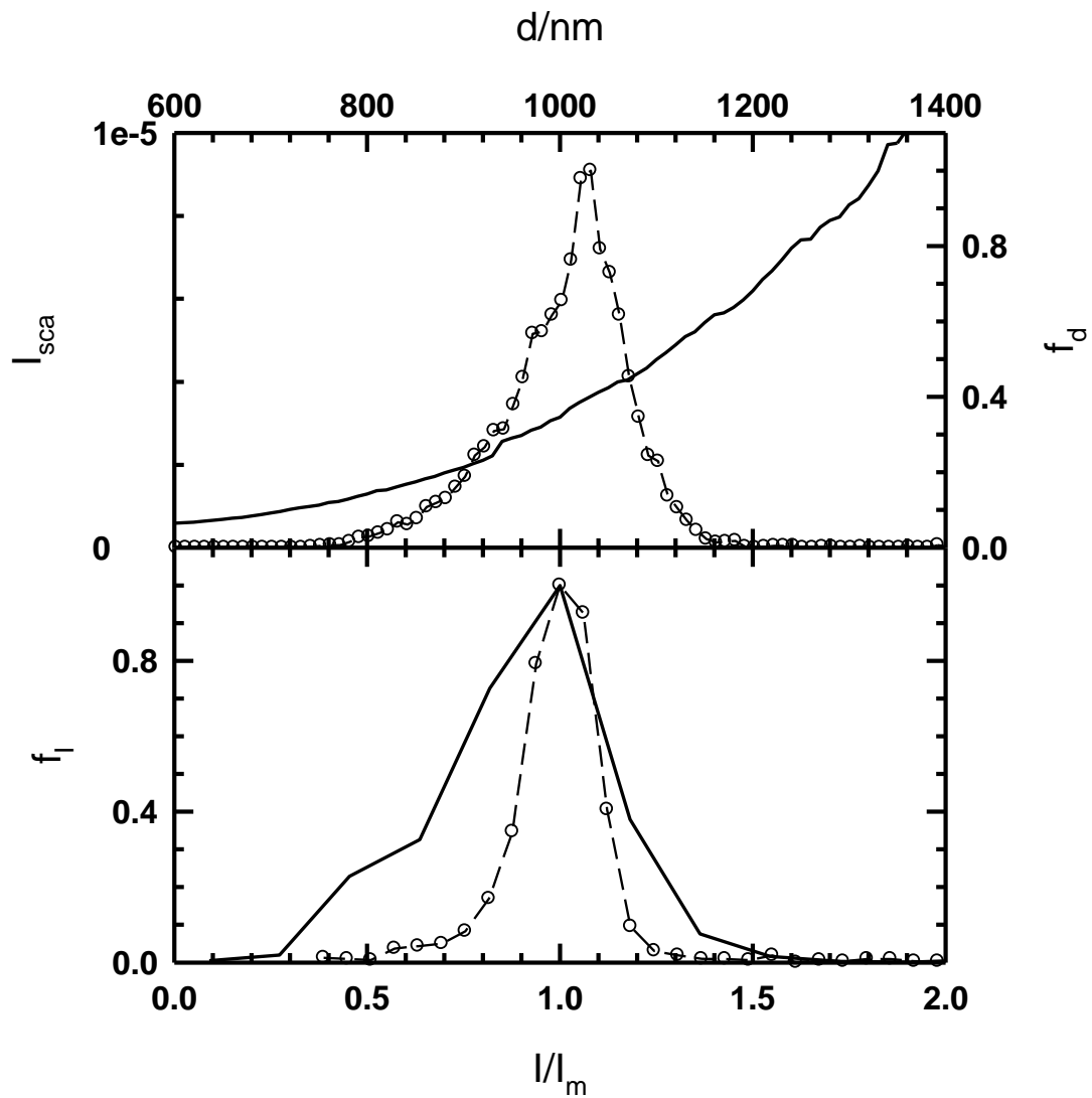
Figure 12 Comparison of values with experimental data for 1\mu\text{m} size distribution and scattering intensity of 1\mu\text{m} PS microspheres. (a) The solid lines represent the theoretical calculated values. For the size distribution plot the frequency ( f_d ) of microspheres are normalized to most probable frequency. (b) The histograms of scattering intensity obtained by theoretical calculations (solid lines) and experimental measurements (dash lines).
