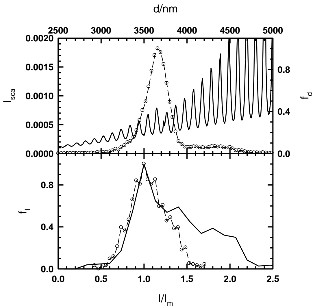
Figure 14 Size distribution and scattering intensity of the 4 \mu\text{m} polydispersed microsphere sample size distribution and scattering intensity of 4 \mu\text{m} PS microspheres. (a) The solid lines represent the theoretical calculated values. For the size distribution plot the frequency ( f_d ) of microspheres are normalized to most probable frequency. (b) The histograms of scattering intensity obtained by theoretical calculations (solid lines) and experimental measurements (dash lines).
