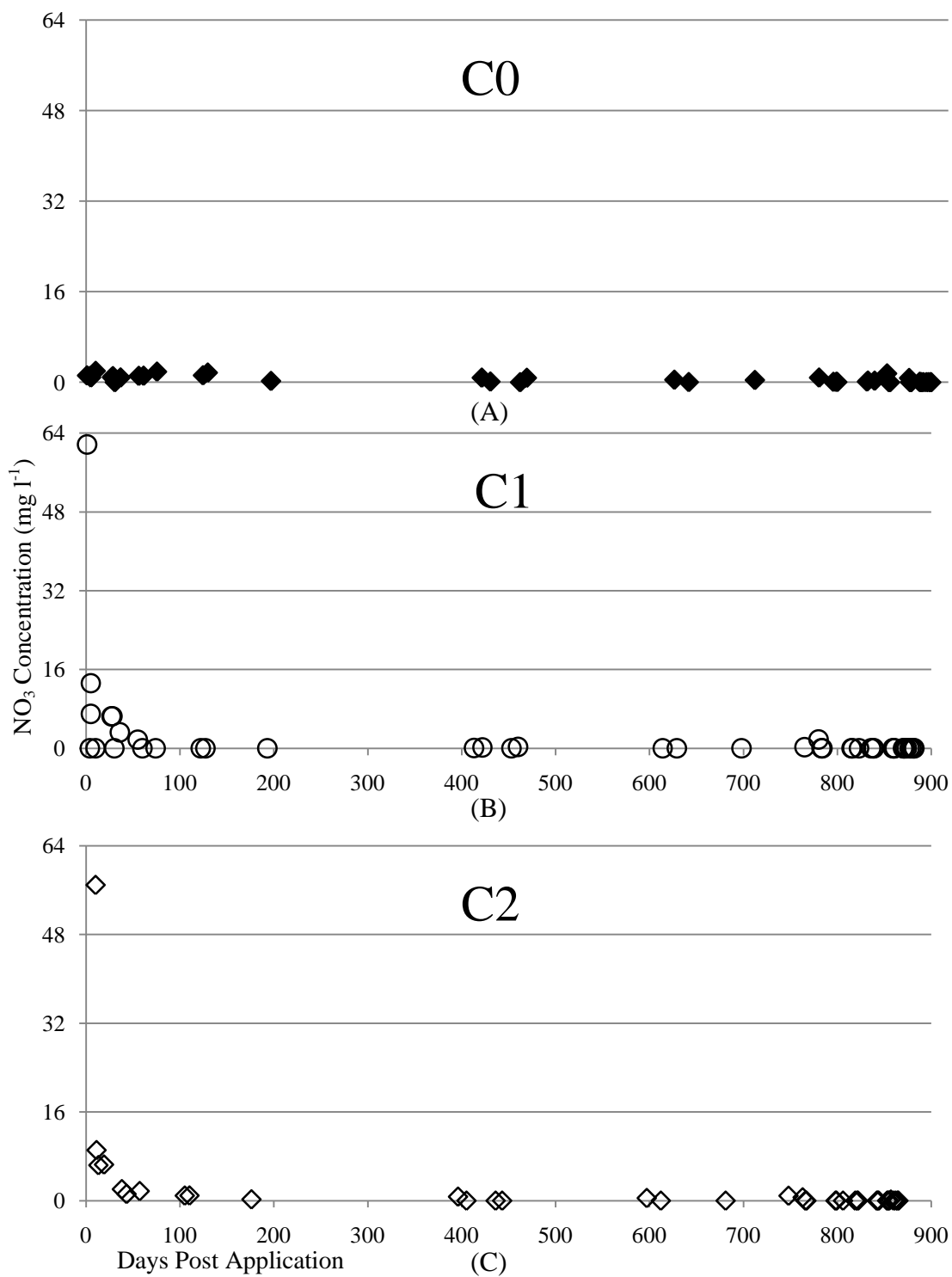
Figure 11 \text{NO}_3^- storm event concentration ( \text{mg l}^{-1} ) for A) C0, control, B) C1, 28 \text{ m}^3 \text{ ha}^{-1} and C) C2, 57 \text{ m}^3 \text{ ha}^{-1} over number of days after compost application. C0 and C1 begin on 26 January 2005 and C2 begins on 13 February 2005.
