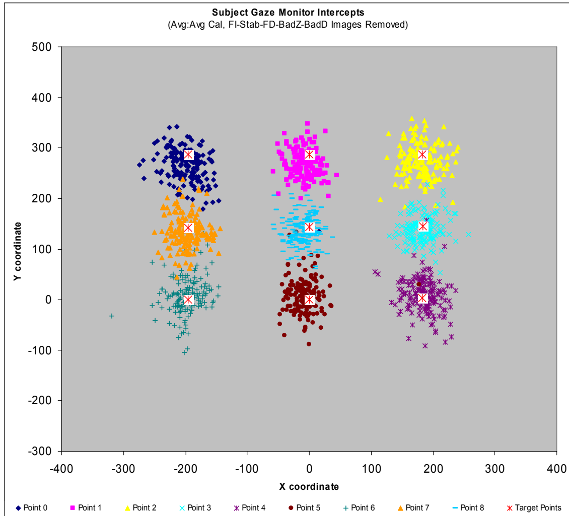
Fig. 25 Gaze monitor intercept (FI-Stab-FD-badZ-badD images excluded).
