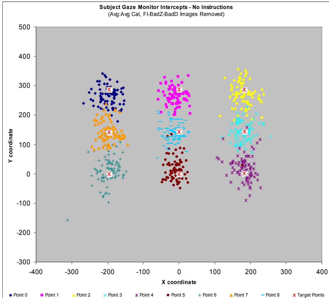
Fig. 27 Monitor intercepts (no instructions).
