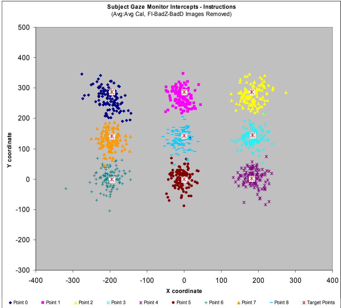
Fig. 26 Monitor intercepts (with instructions).
