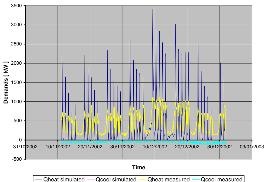
fig. 14 Heating and cooling demands and productions (November and December 2002)
